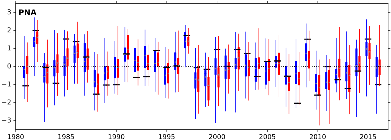
Figure 12. As in Figure 11, but for a PNA index. Anomaly correlation values for the ensemble mean are 0.69 for both systems. The 95% confidence interval for sampling error over years for SEAS5 is 0.47 to 0.83.
