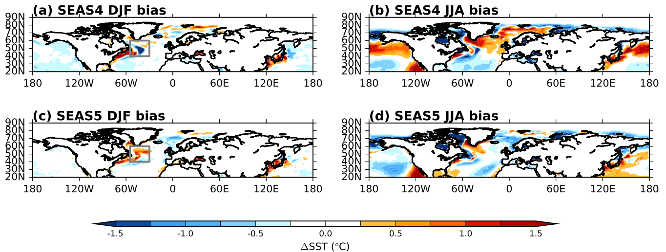
Figure 6. Summer-JJA and winter-DJF SST bias in the northern extratropics at one month forecast lead for SEAS4 (a,b) and SEAS5 (c,d) compared to the analysis they were initialised from (ORAS4, ORAS5). The region discussed in detail later in this section is outlined in grey here.
