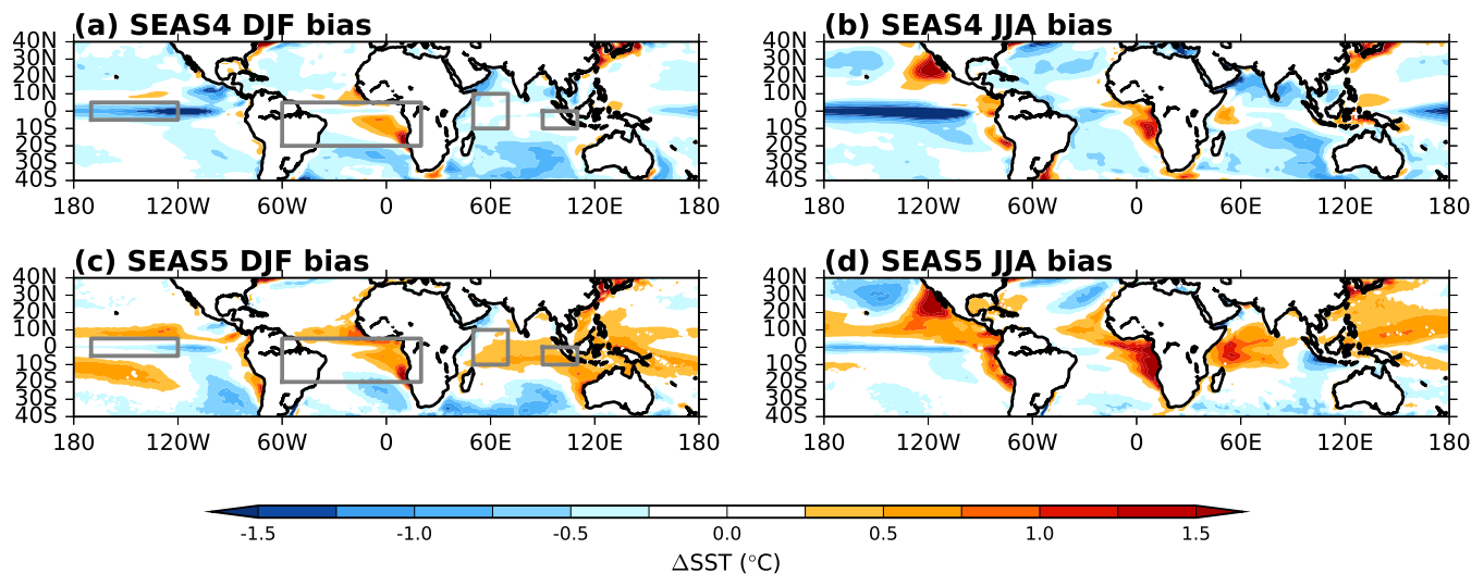
Figure 1. Winter-DJF and summer-JJA SST bias in the tropics at one month lead forecast for SEAS4 (a,b) and SEAS5 (c,d) compared to the analysis they were initialised from (ORAS4, ORAS5). The regions discussed in detail later in this section are outlined in grey here.
