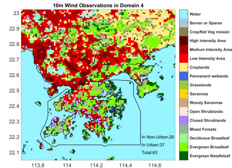
Figure S3: The 10-Meters Wind Observations in Domain 4.
