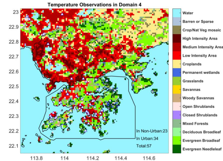
Figure S2: Temperature Observations in Domain 4.
