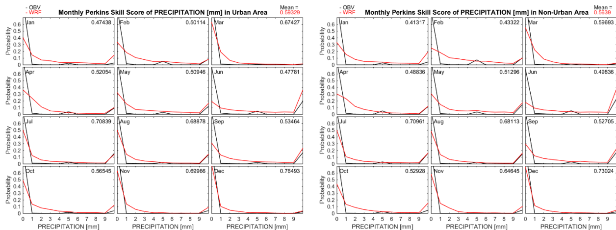
Figure S31: Monthly PSS of Precipitation in Urban (a) and Non-Urban (b) Area.
