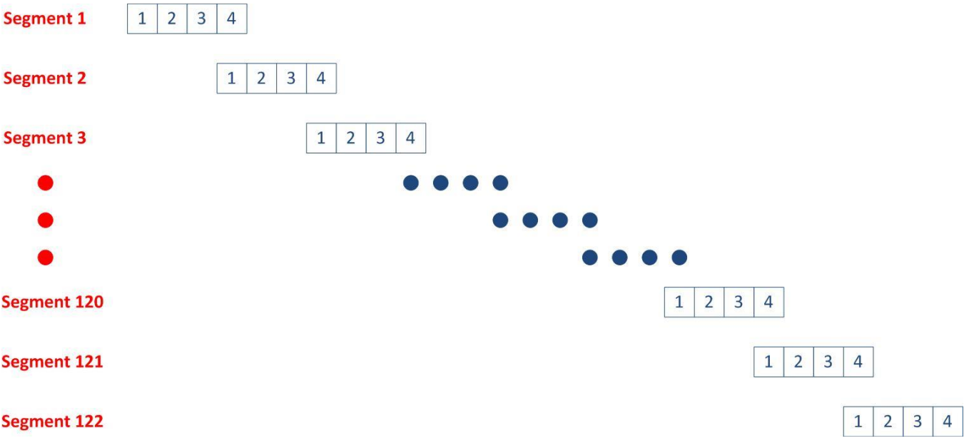
Figure S1: The Simulation Segments' Sequence.
