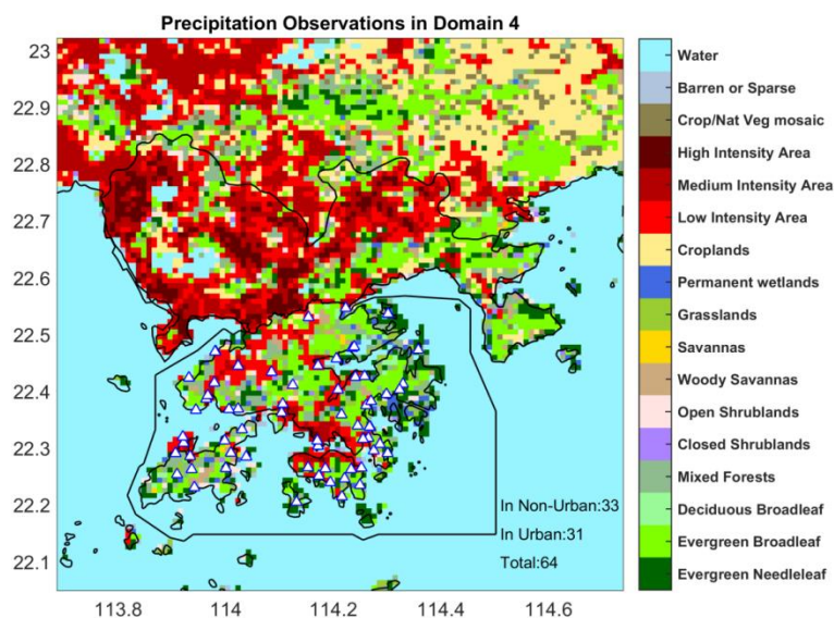
Figure S4: Precipitation Observations in domain 4.
