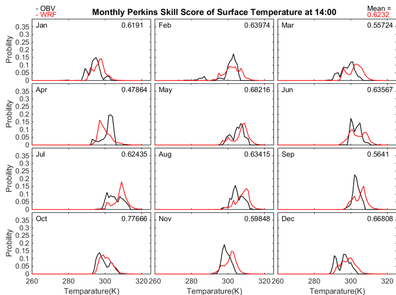
Figure S10: Monthly PSS of Surface Temperature at 14:00.
