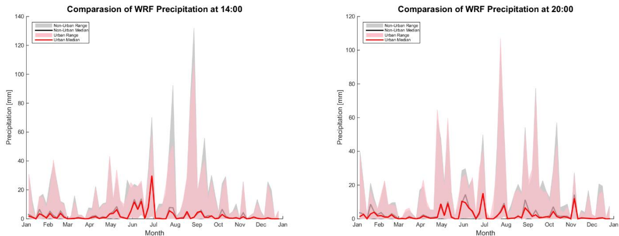
Figure S20: Comparison of WRF Precipitation (at 2:00, 8:00, 14:00 and 20:00) in Urban Area and in the Non-Urban area.
