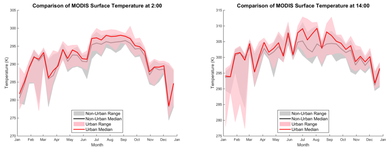
Figure S7: Comparison of MODIS Surface Temperatures (at 2:00 and 14:00) in Urban and Non-Urban Areas.
