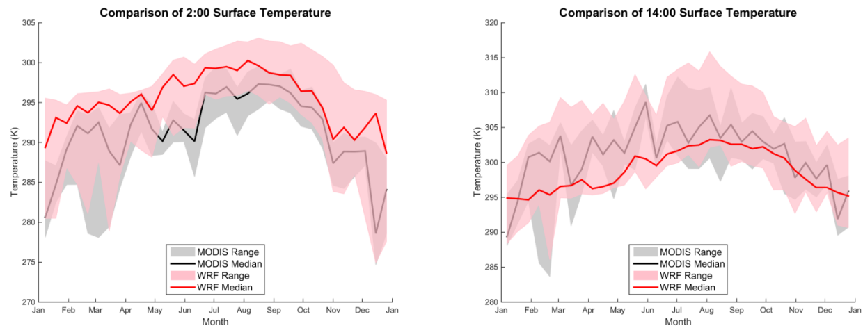
5 Figure S6: Comparison of Modelled and MODIS Surface Temperatures at 2:00 and 14:00.
