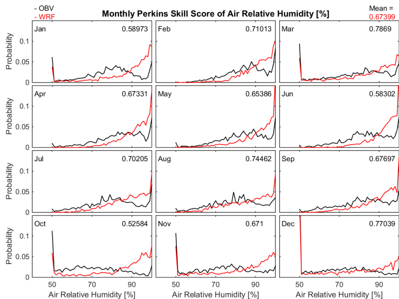
Figure S26: Monthly PSS of Relative Humidity.
