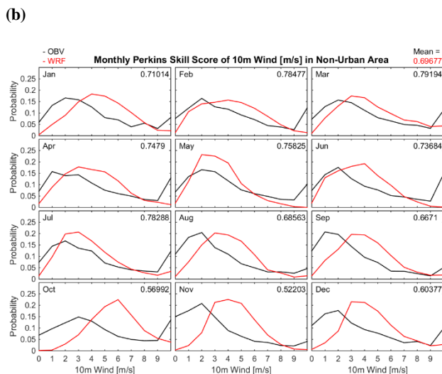
5 Figure S30: Monthly PSS of 10-Meters Wind Speed in Urban (a) and Non-Urban (b) Area.
