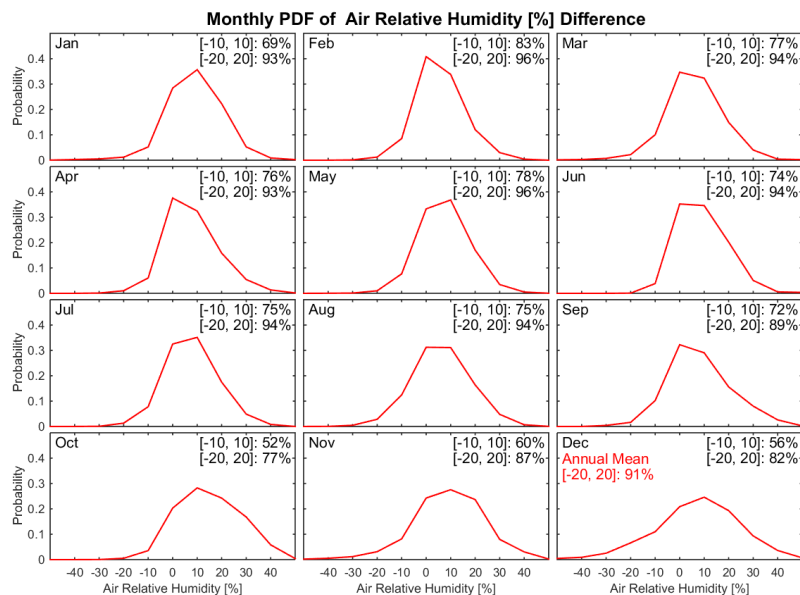
Figure S27: Monthly PDF of Humidity Difference.
