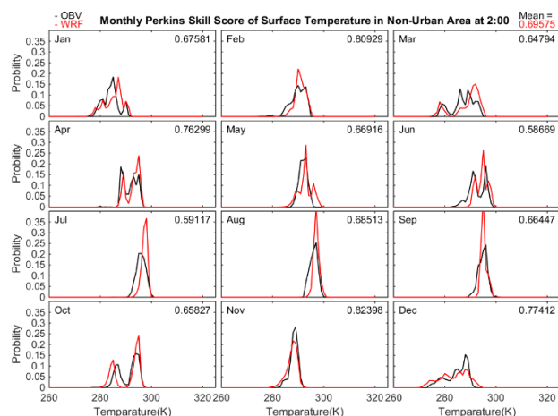
Figure S29: Monthly PSS of Surface Temperature in Urban (a) and Non-Urban (b) Area.
