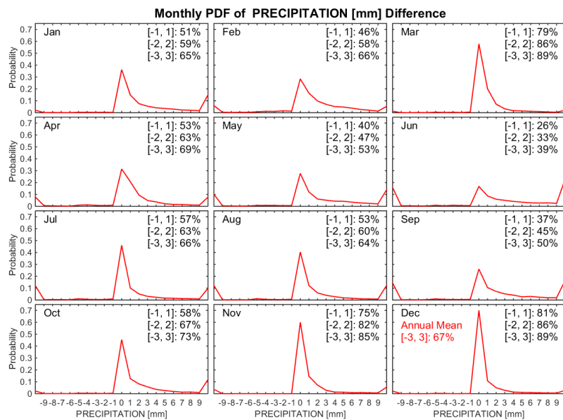
Figure S22: Monthly PDF of Precipitation Difference.
