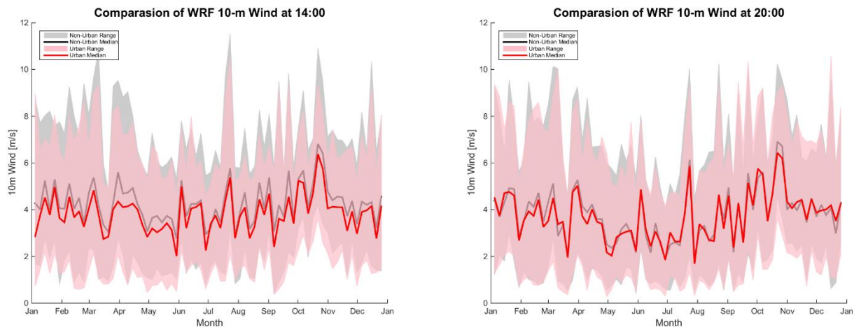
Figure S15: Comparison of WRF 10-meters Wind (at 2:00, 8:00, 14:00 and 20:00) in Urban Area and in the Non-Urban area.
