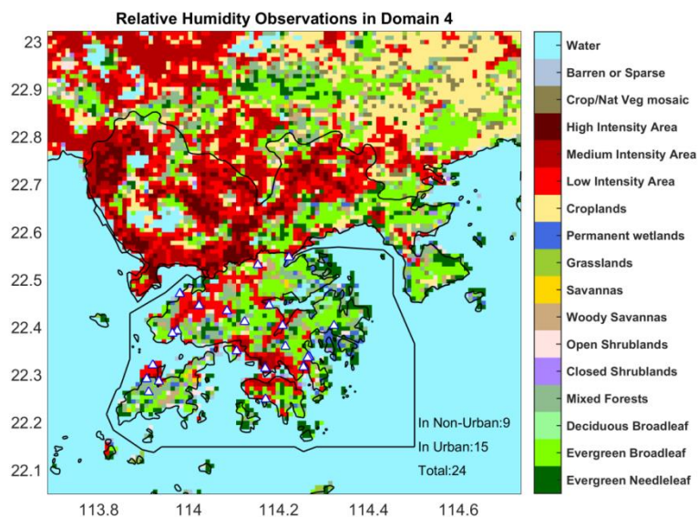
Figure S5: Relative Humidity Observations in domain 4.
