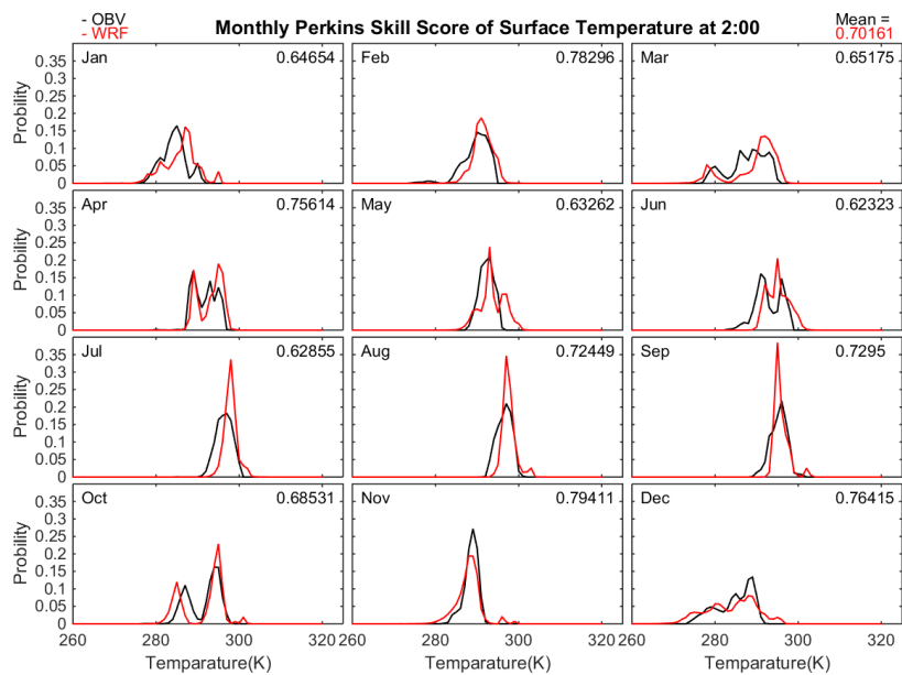
Figure S9: Monthly PSS of Surface Temperature at 2:00.
