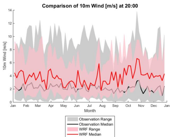
Figure S13: Comparisons of Modelled and Observed 10-Meters Wind Speed at 2:00, 8:00, 14:00 and 20:00.
