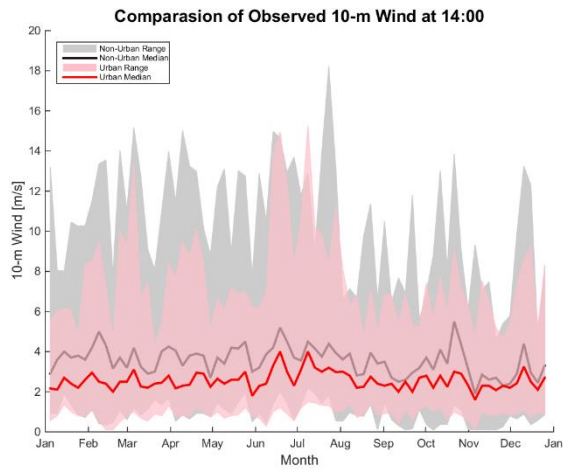
Figure S14: Comparison of Observed 10-Meters Wind (at 2:00, 8:00, 14:00 and 20:00) in Urban Area and in the Non-Urban area.
