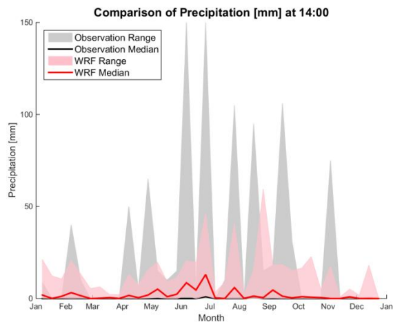
Figure S18: Comparison of Modelled and Observed Precipitations at 2:00, 8:00, 14:00, and 20:00.
