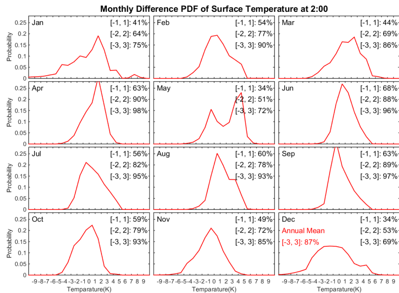
Figure S11: Monthly PDF of 2:00 Surface Temperature Difference.
