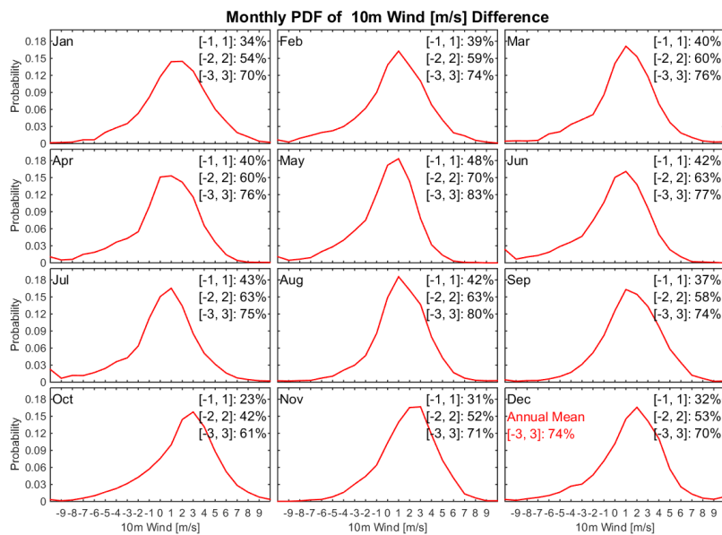
Figure S17: Monthly PDF of 10-Meters Wind Speed Difference.
