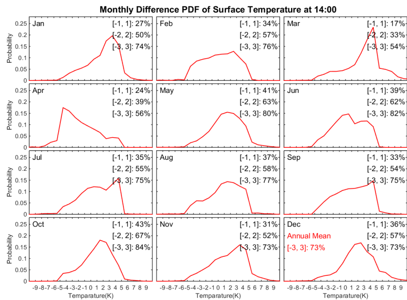
Figure S12: Monthly PDF of 14:00 Surface Temperature Difference.
