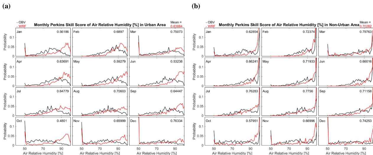
Figure S32: Monthly PSS of Relative Humidity in Urban (a) and Non-Urban (b) Area.
