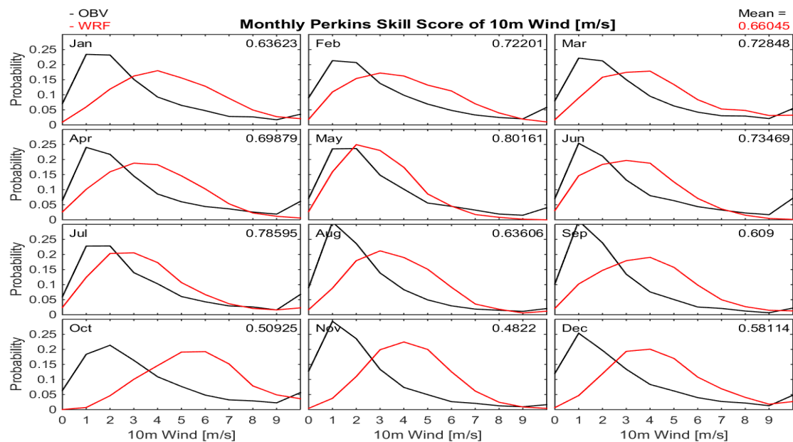
5 Figure S16: Monthly PSS of 10-Meters Wind Speed.
