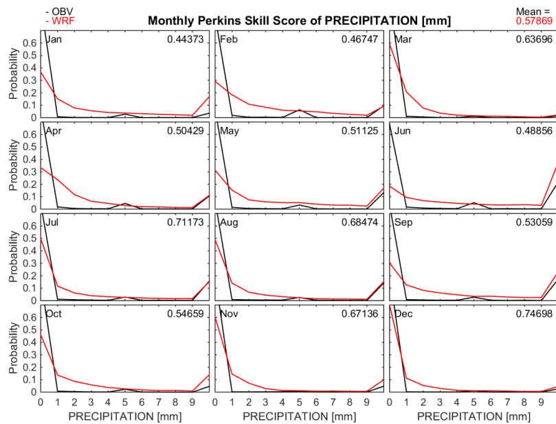
Figure S21: Monthly PSS of Precipitation.
