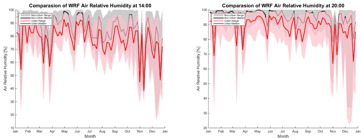
Figure S25: Comparison of Modelled Relative Humidity (at 2:00, 8:00, 14:00 and 20:00) in Urban and Non-Urban Areas.
