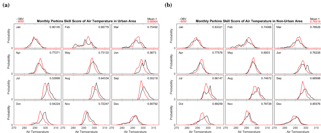
Figure S28: Monthly PSS of 2-Meters Air Temperature in Urban (a) and Non-Urban (b) Area.
