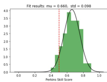
Figure 1. Histogram of the Perkins skill score for 72 monthly PDF analysis . A normal distribution was fit. The red dashed line indicate the lower bound for 95% confidence (PSS=0.500).
