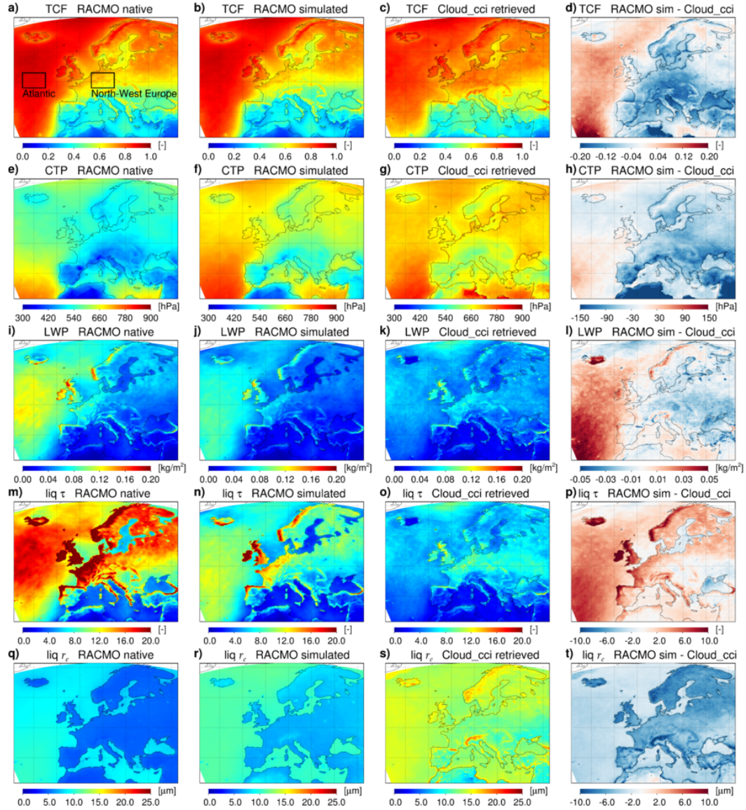
Figure 11. Maps of 2011–2014 mean modeled and retrieved cloud properties: a-d) total cloud fraction, e-h) cloud top pressure (hPa), i-l) LWP ( \text{kg m}^{-2} ), m-p) liquid \tau , and q-t) liquid r_e ( \mu\text{m} ). The columns show from left to right the native model, the simulator, the Cloud_cci data, and the difference between simulator and retrieval. All properties are all-sky averages, except CTP and r_e , which are in-cloud averages. In addition, CTP has been logarithmically averaged, while the other properties have been linearly averaged. Panel (a) shows the areas defined for the time series analysis in Fig. 10.
