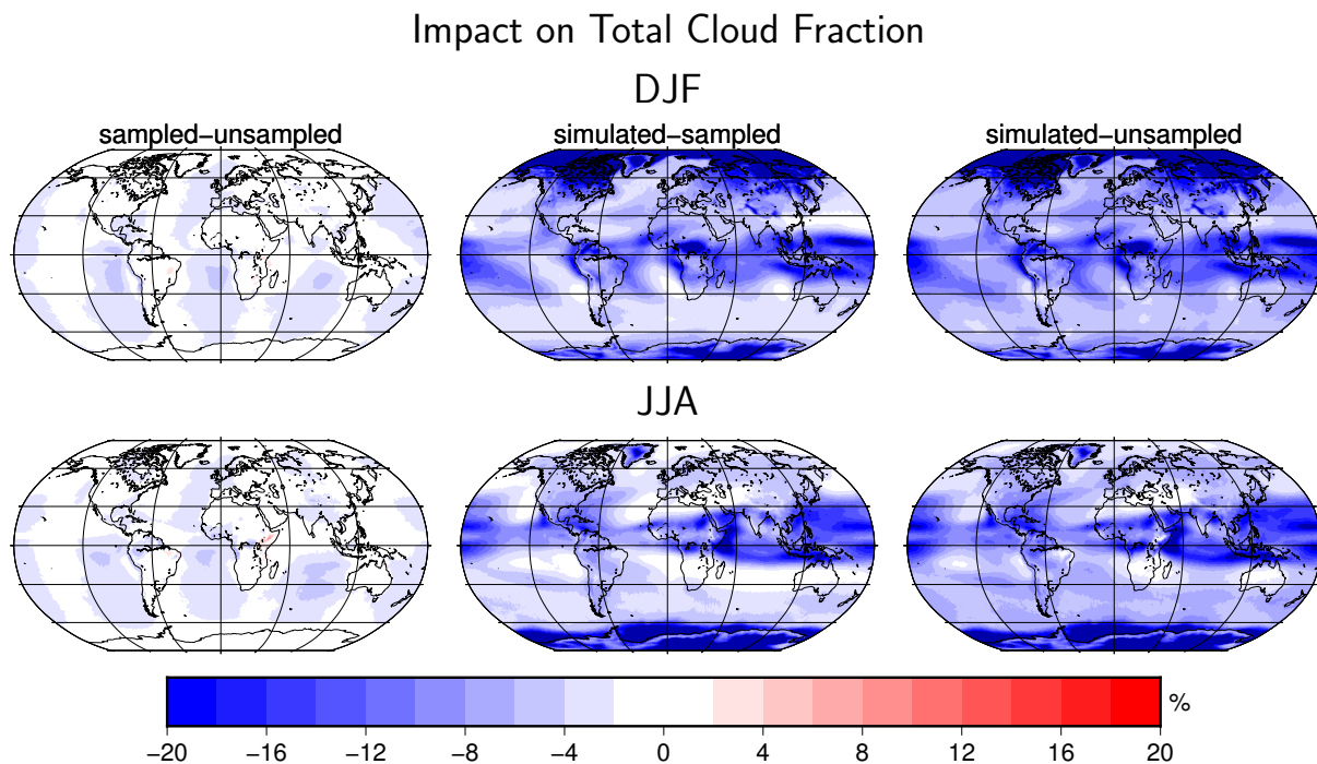
Figure 3. The simulated TCF minus the direct model output of TCF. The leftmost column shows the impact of sampling the model to match the EOT of the satellites in a similar way as in Fig. 2, but this time for TCF and using the EOT shown in Fig. 1. It is the temporally sampled direct model output minus the direct model output (sampled-unsampled). The middle column shows the simulated lack of sensitivity of the AVHRR sensor to optically very thin clouds ( \tau_c < 0.2 ). Specifically it shows the simulated Cloud_cci minus the temporally sampled direct model output (simulated-sampled). The rightmost column shows the combined impact on these two effects, i.e., clouds removed and temporal sampling, compared to the direct model output (simulated-unsampled). The top row is valid for DJF, and the bottom is for JJA. The data covers the period 1982–2014.
