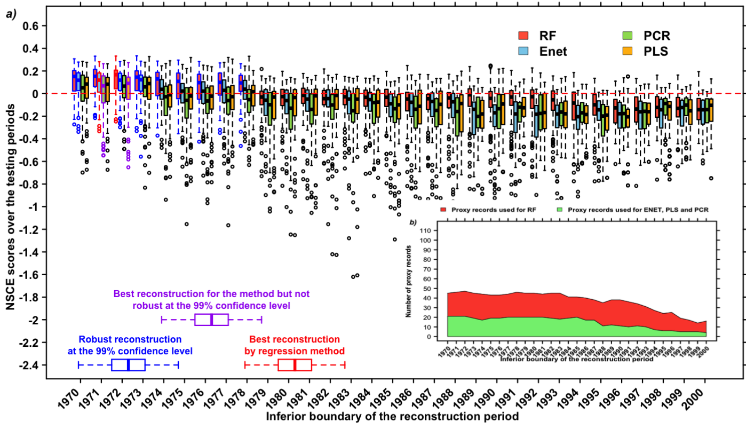
FIGURE 7 – a) Reconstructions are performed using 31 reconstruction period for the four methods: from 1000-1970 to 1000-2000 by moving the superior born by 1 with R = 50 training/testing samples. RF reconstructions are performed using the proxy records significantly correlated at the 80% confidence level with the NAO over the training periods (section 3.1.1). PCR reconstructions are performed using by selecting the proxy records significantly correlated at the 95% confidence level with the NAO over the training periods (section 3.1.1). PLS and Enet reconstructions are performed using by selecting the proxy records significantly correlated at the 95% confidence level with the NAO over the training periods (section 3.1.1). a) Red boxplots are the NSCE scores obtained using RF method. Blue boxplots are the NSCE scores obtained using Enet method. Red green are the NSCE scores obtained using PCR method. Yellow boxplots are the NSCE scores obtained using PLS method. Boxplots with blue edges are the scores significantly positives at the 99% confidence level. Boxplots with red edges correspond to the scores associated with the best reconstruction for each method. b) Proxy records available/used by reconstruction period. Red area gives: Number of records used for: Green area: Number of records used for Enet, PCR and PLS for each reconstruction period.
