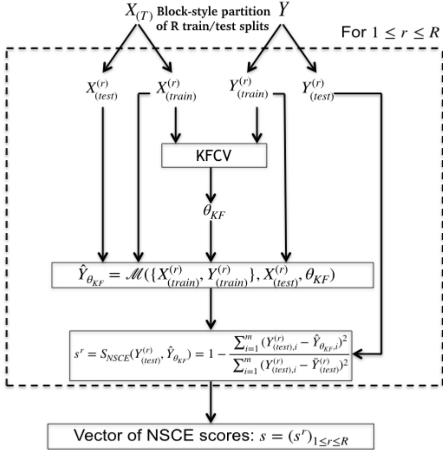
FIGURE 4 – Scheme of the whole procedure for scores calculation for a given method \mathcal{M} . Y is the index of the chosen mode of variability. X_{(T)} is the proxy dataset restricted to the period where Y is known. \{X_{(train)}^{(r)}, Y_{(train)}^{(r)}\} is the r^{\text{th}} training sample and \{X_{(test)}^{(r)}, Y_{(test)}^{(r)}\} is the r^{\text{th}} testing sample. \theta_{KF} is the empirically optimal set of parameters obtained by applying the KFCV (Fig 3; section 2.3.3)
