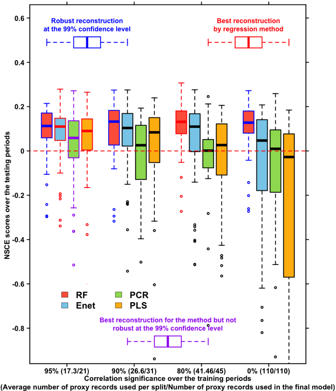
FIGURE 6 – Boxplot of NSCE scores obtained for the four methods and different groups of proxy records by reconstructing the NAO index on the period 1000-1970 with R = 50 training/testing samples. Green boxplots are the NSCE scores obtained for the PCR method. Yellow boxplots are the NSCE scores obtained for the PLS method. Red boxplots are the NSCE scores obtained for the RF method. Blue boxplots are the NSCE scores obtained for the Enet method. The first cluster of boxplots is the NSCE scores obtained by using all the available proxy records over the period (110 proxy records). The second cluster of boxplots is the NSCE scores obtained by using only proxy records significantly correlated with the NAO index at the 80% confidence level over the training periods. The third cluster of boxplots is the NSCE scores obtained by using only proxy records significantly correlated with the NAO index at the 90% confidence level over the training periods. The fourth cluster of boxplots is the NSCE scores obtained by using only proxy records significantly correlated with the NAO index at the 95% confidence level over the training periods. Boxplots with blue edges are the scores significantly positives at the 99% confidence level. Boxplots with red edges correspond to the scores associated with the best reconstruction for each method.
