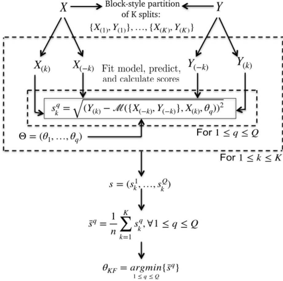
FIGURE 3 – Scheme of a K-Fold cross validation procedure to select the optimal control parameter of a specific learning method \mathcal{M} . X is the input set of predictors and Y the corresponding variability mode index. \forall 1 \leq i \leq n , \{X_{(k)}, Y_{(k)}\} is the k^{\text{th}} block-style based group of observation and \{X_{(-k)}, Y_{(-k)}\} contains all observations except the i^{\text{th}} . \Theta = (\theta_1, \dots, \theta_Q) is the ensemble of possible values of the s control parameters \theta \in \mathbb{R}^s .
