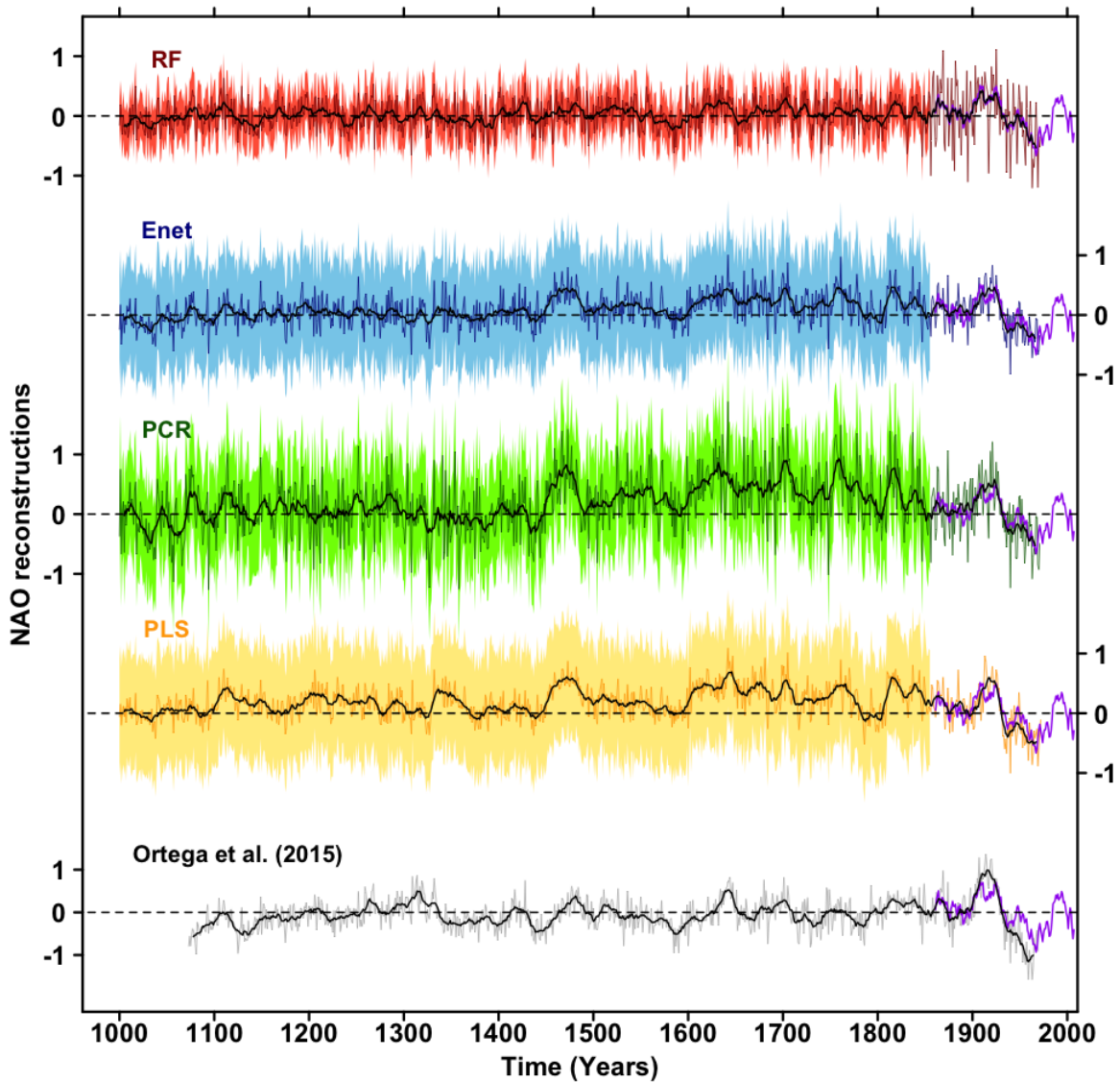
FIGURE 8 – Red line: RF reconstruction on the period 1000-1972 (section 3.1.2), using proxy records significantly correlated at the 80% confidence level with the NAO over the training periods (section 3.1.1). Blue line: Enet reconstruction on the period 1000-1971 (section 3.1.2) by selecting the proxy records significantly correlated with the NAO index at the 95% confidence level over the training periods (section 3.1.1). Green line: PCR reconstruction on the period 1000-1971 (section 3.1.2) by selecting the proxy records significantly correlated with the NAO index at the 95% confidence level over the training periods (section 3.1.1). Orange line: PLS reconstruction on the period 1000-1972 (section 3.1.2) by selecting the proxy records significantly correlated with the NAO index at the 95% confidence level over the training periods (section 3.1.1). Black line (tiny): Ortega et al. calibration constrained reconstruction [Ortega et al., 2015]. Red area: Regression uncertainties (see supplementary material 3) for RF reconstruction. Blue area: Regression uncertainties for Enet reconstruction. Blue area: Regression uncertainties for PCR reconstruction. Orange area: Regression uncertainties for PLS reconstruction. Heavy black lines are the corresponding 11-year filtered reconstructions for each method. Purple lines: superposed 11-years filtered Jones et al. (1997) NAO index.
