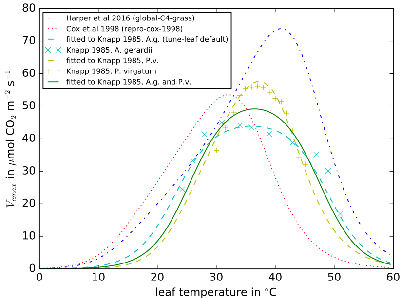
Figure 4. V_{cmax} against leaf temperature for A. gerardii (cyan diagonal crosses) and P. virgatum . (yellow vertical crosses), using the normalised observations from Figure 2 in Knapp (1985), scaled using the fitted light response curves of A. gerardii and P. virgatum at 35°C shown in Figure 3. JULES parameters are fitted to these derived A. gerardii observations (cyan dashed line) and P. virgatum . observations (yellow dashed line) and a combination of both (green solid line). Also shown are the relations from the repro-cox-1998 (red dotted line) and global-C4-grass runs (blue dot-dashed line). Model lines have been created using the Leaf Simulator package.
