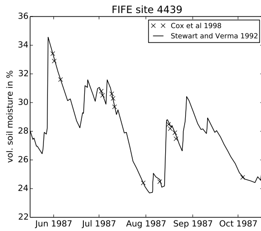
Figure A3. Soil moisture data from Cox et al. (1998), compared to the derived time series of top 1.1m soil moisture in Figure 1 of Stewart and Verma (1992). Both datasets are for FIFE site 4439 in 1987.
