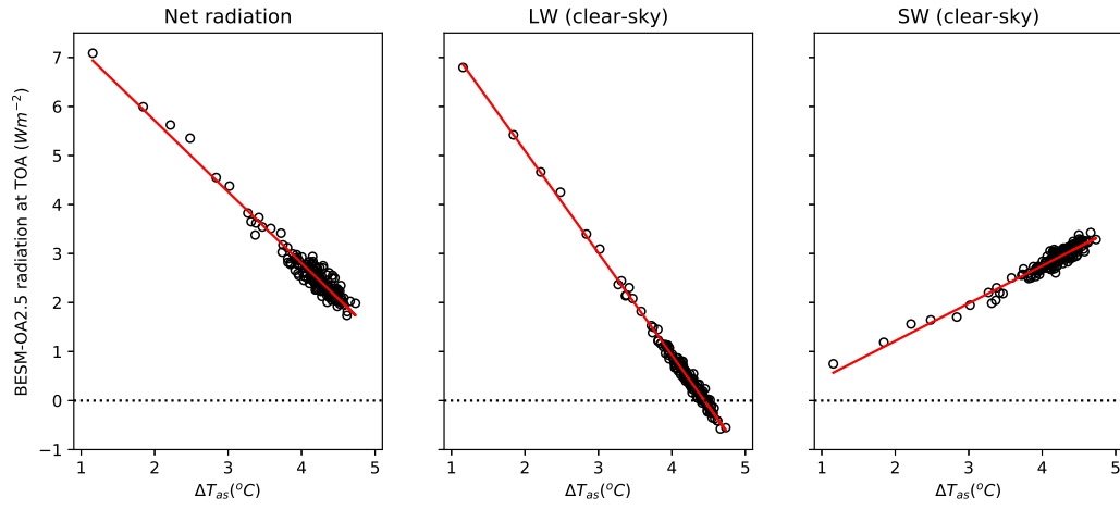
Figure 1. Annual global-mean linear regression between \Delta\bar{T}_{as} and: (a) Net radiation, (b) \Delta LW (clear-sky), and (c) \Delta SW (clear-sky) for BESM-OA2.5
