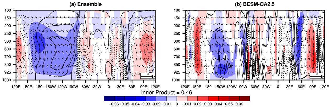
Figure 13. Difference (averaged over years 120-150) between the abrupt4xCO2 and piControl conditions for generalized vertical motion [omega (Pa/s), in shades] and the mean zonal and vertical motion (vectors), averaged between 5°S and 5°N, for (a) the CMIP5 ensemble and (b) BESM-OA2.5. The contours represent the averaged piControl vertical motion (omega) in the same region. The white regions have confidence levels less than 90%.
