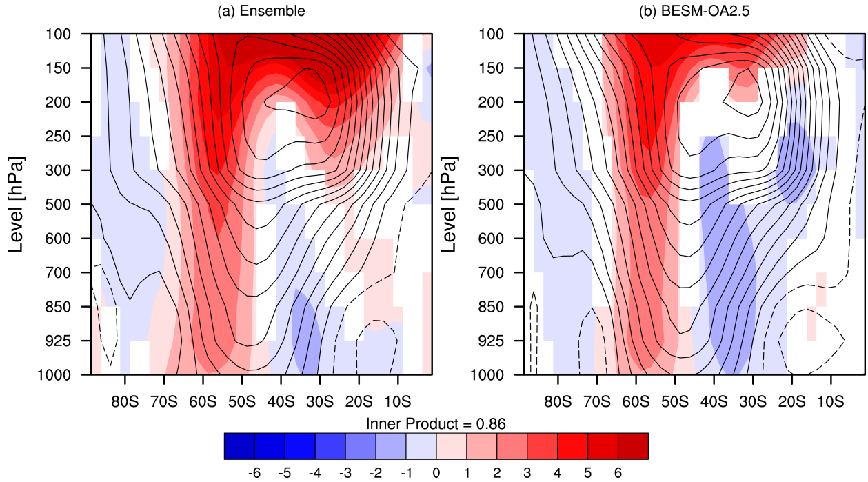
Figure 12. Vertical profile of the difference (averaged over years 120-150) in the zonal wind (in m/s) between two scenarios (abrupt4xCO2 minus piControl, shaded), and the piControl conditions (contours) for (a) the ensemble of CMIP5 models and (b) BESM-OA2.5. The white areas have confidence levels less than 90%.
