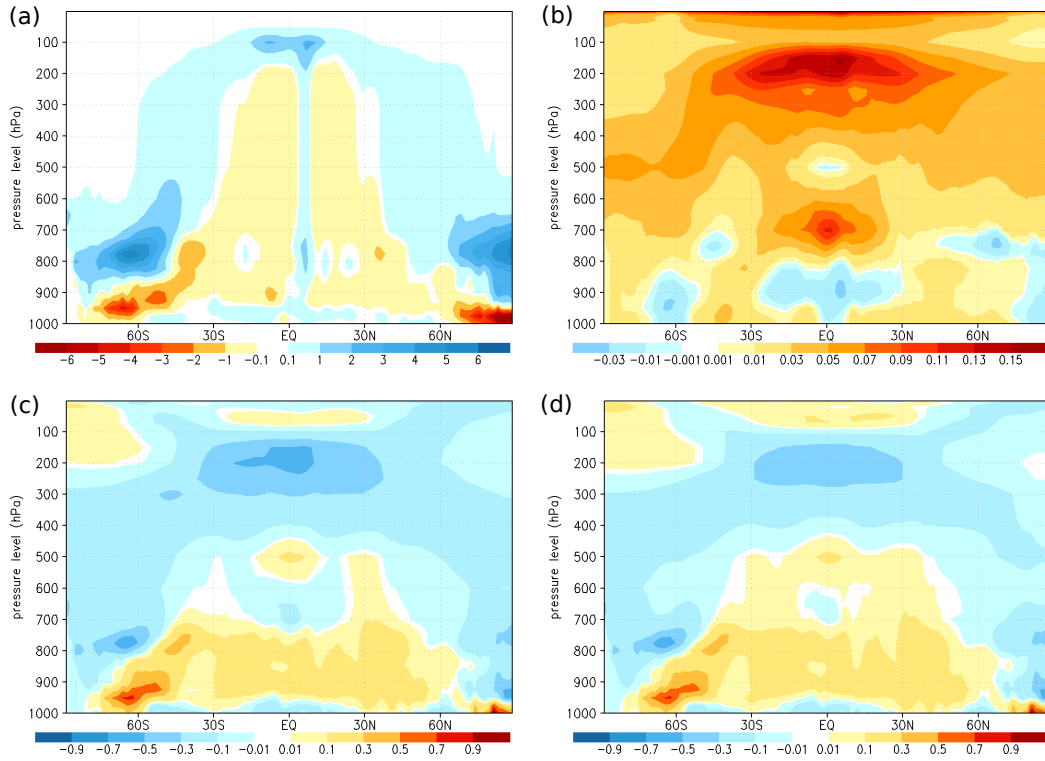
Figure 7. Vertical profiles of the zonal mean of the 4xC 2 - piControl mean difference for the following variables: (a) cloud fraction, radiative heating/cooling rate ( dT/dt , in K day^{-1} ) of (b) shortwave, (c) long wave and (d) sum of the shortwave and longwave for BESM-OA2.5.
