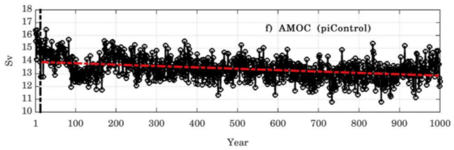
Fig. 1. Maximum AMOC simulated by the piControl from the beginning of the simulation up to 1000 years. The red dash-dot lines shows the linear trend.
