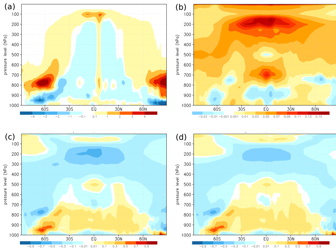
Fig. 3. Vertical profiles of the zonal mean of the 4xCO 2 - piControl mean difference for the following variables: (a) Cloud fraction, Radiative heating-cooling rate (dT/dt) of (b) shortwave, (c) longwave ...
