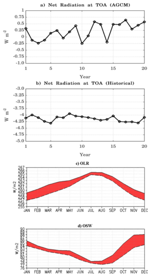
Fig. 1. Net of the radiation at the TOA by (a) AGCM and (b) BESM-OA2.5 Historical. (c) and (d) outgoing LW and outgoing SW radiation, respec...
