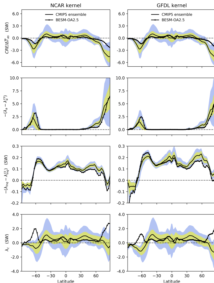
Fig. 2. Cloud feedback and the albedo and SW humidity feedbacks cloud masking for the CMIP5 multi-model ensemble-mean (solid line) and BESM-OA2.5 (solid line with dots)...
