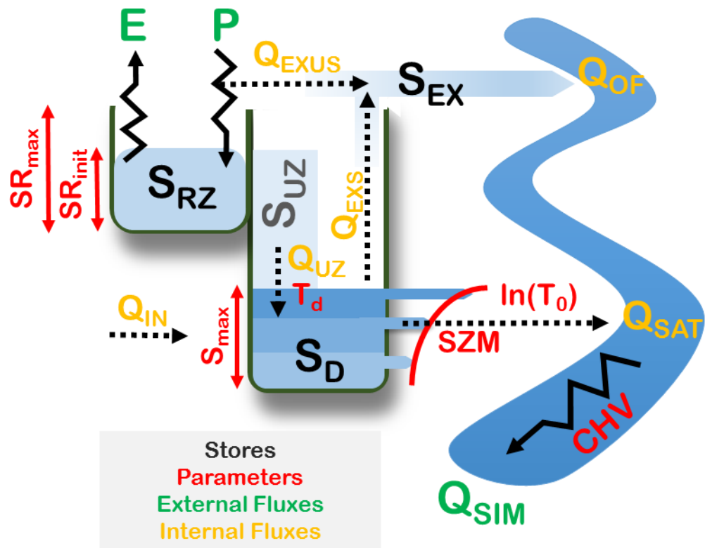
Figure 3. Simplified conceptual diagram of the model structure currently implemented in DECIPHÉR. All scientific notations are described in Table 1.
