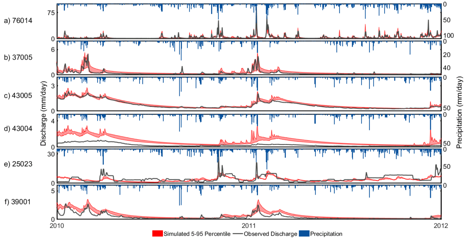
Figure 9. Observed discharge and uncertainty bounds for the behavioural simulations (5 th and 95 th percentile of the likelihood-weighted simulated discharge) for six catchments with different characteristics (shown in Table 5). The plots show a two year period (2010-2012) from the 55 year time series simulated.
