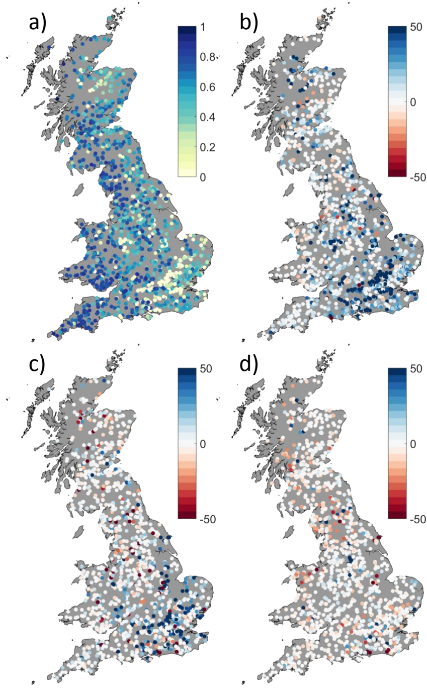
Figure 7. Model performance for the best simulation (as defined by the combined rank across all four metrics) for each evaluation metric a) NSE (-), b) Bias in Runoff Ratio (%), c) Bias in Low Flow Volume (%), and d) Bias in Slope of the Flow Duration Curve between the 30 th and 70 th percentile
