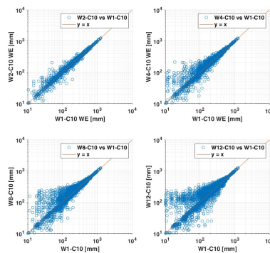
Fig. 1: Scatter plot of the pixel-by-pixel comparison of SWE, obtained by updating the SWE classes at decreasing frequency ranging from 2 weeks to 12 weeks. The updating frequency of 1 week is used as reference. The study period is from October 2010 to June 30 2011.
