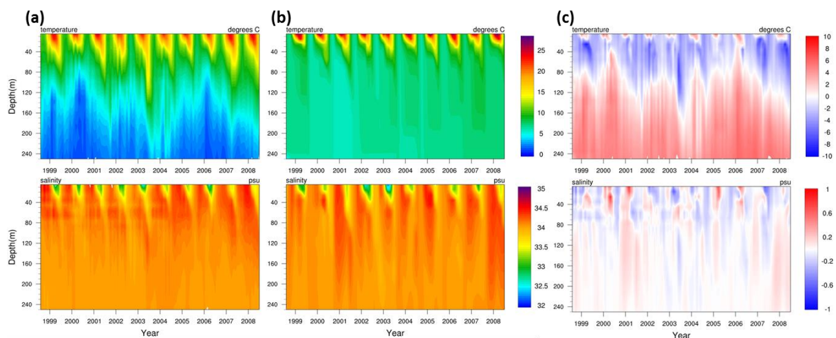
Figure 3: Comparison of the vertical distribution for water temperature [°C], salinity [psu] at point 107 for the 10-year period (1999–2008); (a), (b), and (c) represent observation, GOTM-TOPAZ, and the difference (GOTM-TOPAZ minus observation), respectively.
