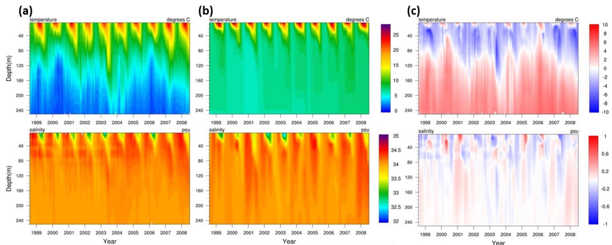
Figure 3: Comparison of the vertical distribution for water temperature [ ^{\circ}\text{C} ], salinity [psu] at point 107 for the 10-year period (1999–2008); (a), (b), and (c) represent observation, GOTM-TOPAZ, and the difference (GOTM-TOPAZ minus observation), respectively.
