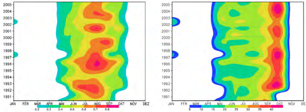
Fig. 13. Seasonal cycle of thermocline structure. Left: thermocline intensity ( C^{\circ} m^{-1} ) averaged over the entire thermal stratified area. Right same as left but for thermocline depth (m).
