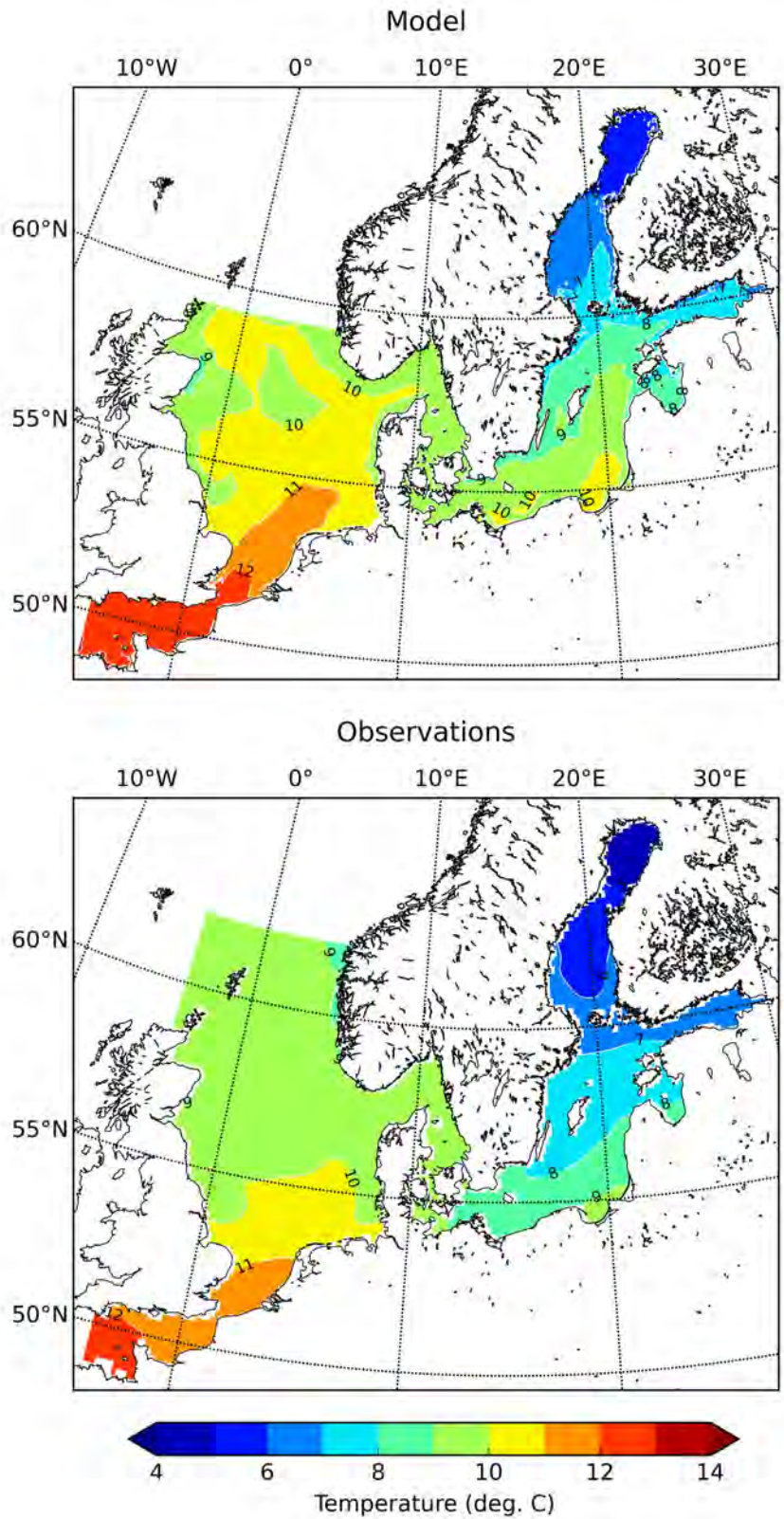
Fig. 5. Mean surface (0-10 m) temperature for Baltic, North Sea and English Channel, as simulated by Nemo-Nordic for the period 1979-2010 (upper figure) and from observations (lower figure) from Janssen et al. (1999).
