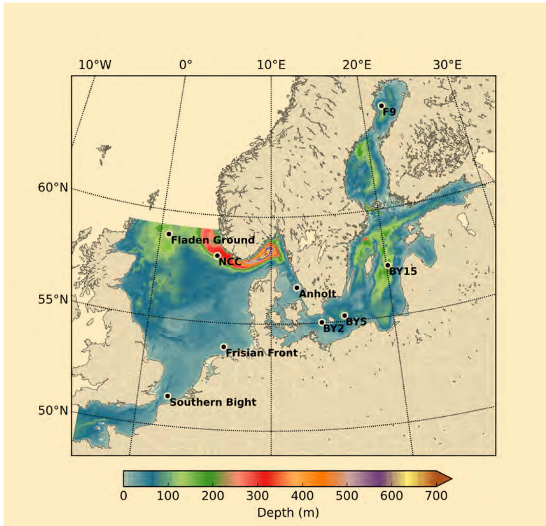
Fig. 1. The model domain and bathymetry of Nemo-Nordic. The filled circles show the locations of validation stations for salinity and temperature.
