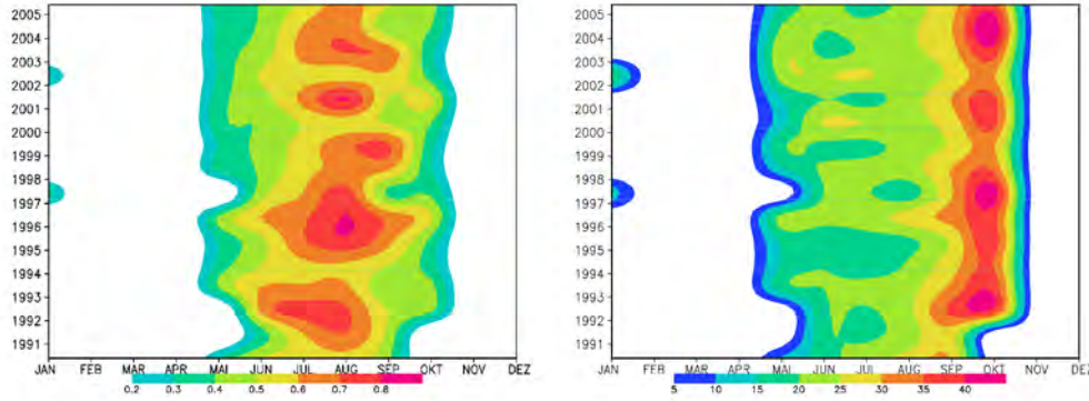
Fig. 15. Seasonal cycle of thermocline structure. Left: thermocline intensity (Degrees \text{m}^{-1} ) averaged over the entire thermal stratified area. Right same as left but for for thermocline depth (m).
