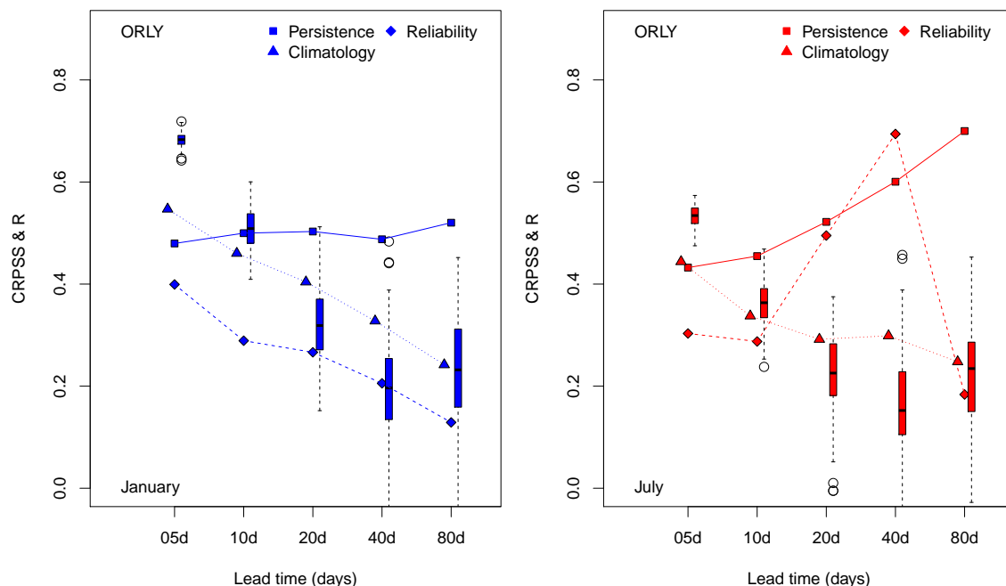
Figure 7. Skill scores for temperature in Orly (continued).
