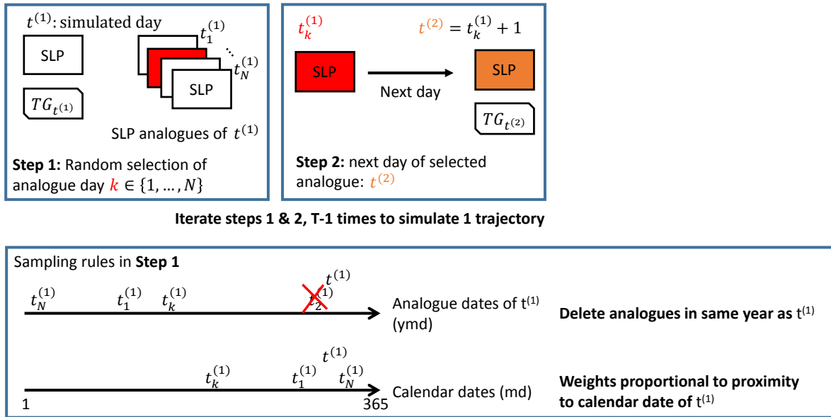
Figure 2. Schematic of the iteration procedure to simulate one random trajectory of temperature (TG) from SLP analogues. The values of t^{(k)} are the days to be simulated by the system. The values of t_1^{(k)}, \dots, t_N^{(k)} are the analogue days for t^{(k)} . The red SLP rectangles are the randomly selected analogues, according to the rule defined in the lower box. This procedure is repeated S times to generate an ensemble of trajectories.
