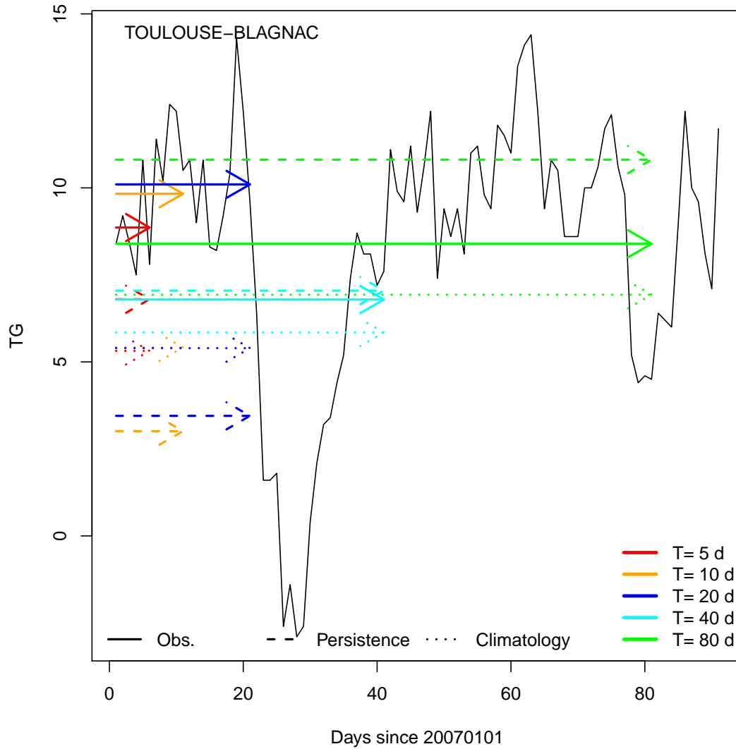
Figure 3. Illustration of average forecast for daily mean temperature (TG) in Toulouse, for Jan. 1st 2007. The continuous black line indicates the observations of TG for the first 90 days of 2007. The colors indicate lead times T . The continuous arrows are for averages of observed TG from Jan. 1st 2007 to the lead time T . The dashed lines are for the persistence forecast of TG and the dotted lines are for the climatology forecast of TG on Jan. 1st 2007.
