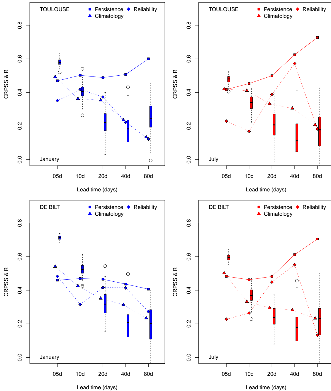
Figure 7. Skill scores for mean daily temperature in Toulouse, De Bilt, for lead times T of 5, 10, 20, 40 and 80 days. Square indicate CRPSS_{pers} , triangles CRPSS_{clim} and circles are fore correlation. The diamonds indicate the reliability of CRPS (on the same scale as CRPSS). Blue symbols (left) are for January and red symbols (right) are for July. Triangles are identical for January and July. The boxplots for the correlation indicate the spread across the 100 member ensemble forecasts.
