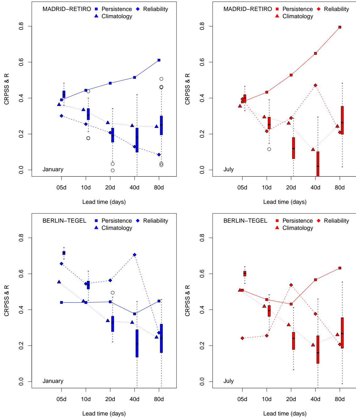
Figure 7. Skill scores for temperature in Madrid and Berlin (continued).
