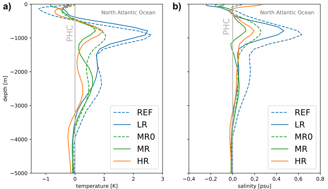
Figure 3. Profiles of potential temperature a) and salinity b) in the North Atlantic Ocean for years 71–100 of the pre-industrial simulations. Shown is the mean difference to the PHC climatology (PHC 3.0, updated from: Steele et al., 2001). With the medium- and high-resolution meshes, the biases around 1000 m depth decrease strongly for both temperature and salinity.
