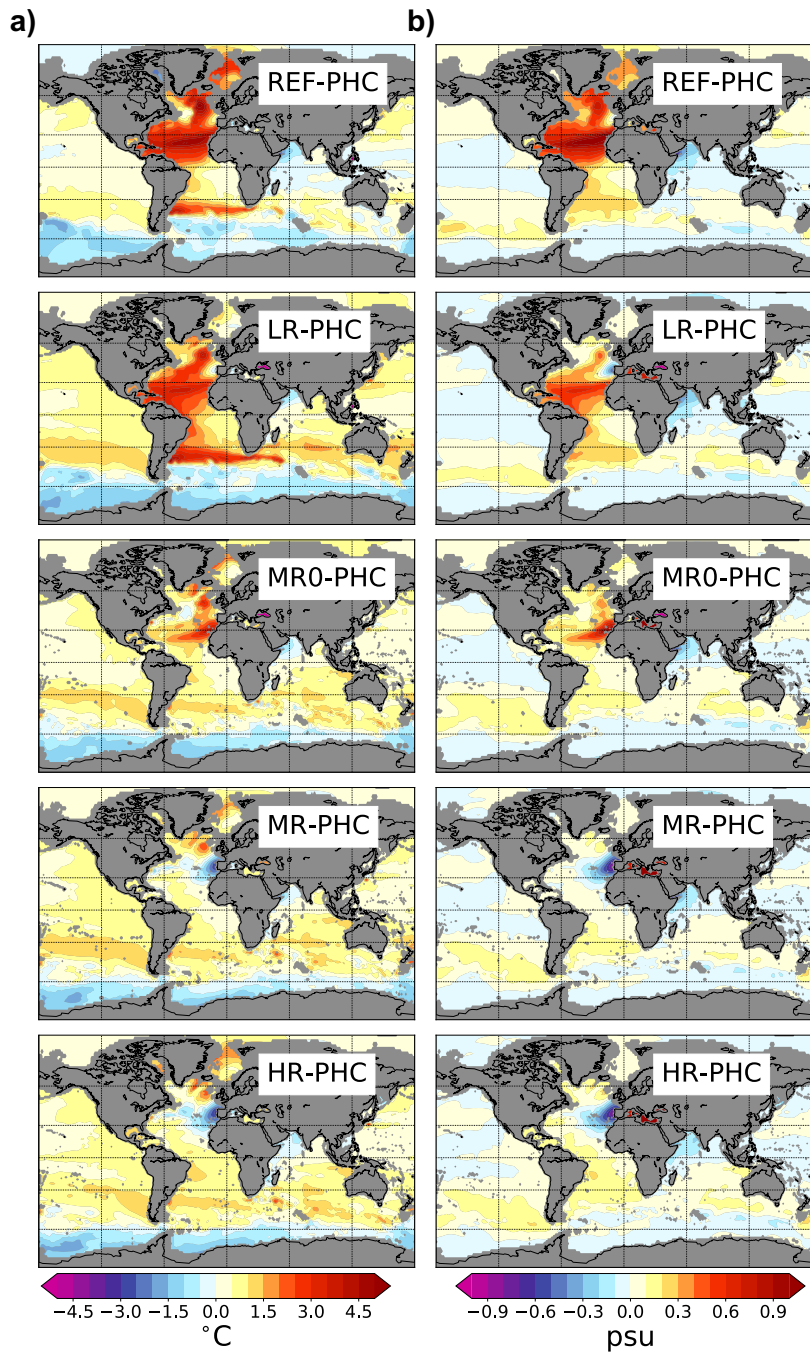
Figure 6. a) Potential temperature [ ^{\circ}\text{C} ] and b) salinity [psu] biases with respect to the PHC climatology (PHC 3.0, updated from: Steele et al., 2001) at 1000 m depth, plotted on the observational grid. A systematic decrease of the temperature and salinity biases in the North Atlantic with increasing resolution (top to bottom) is evident.
