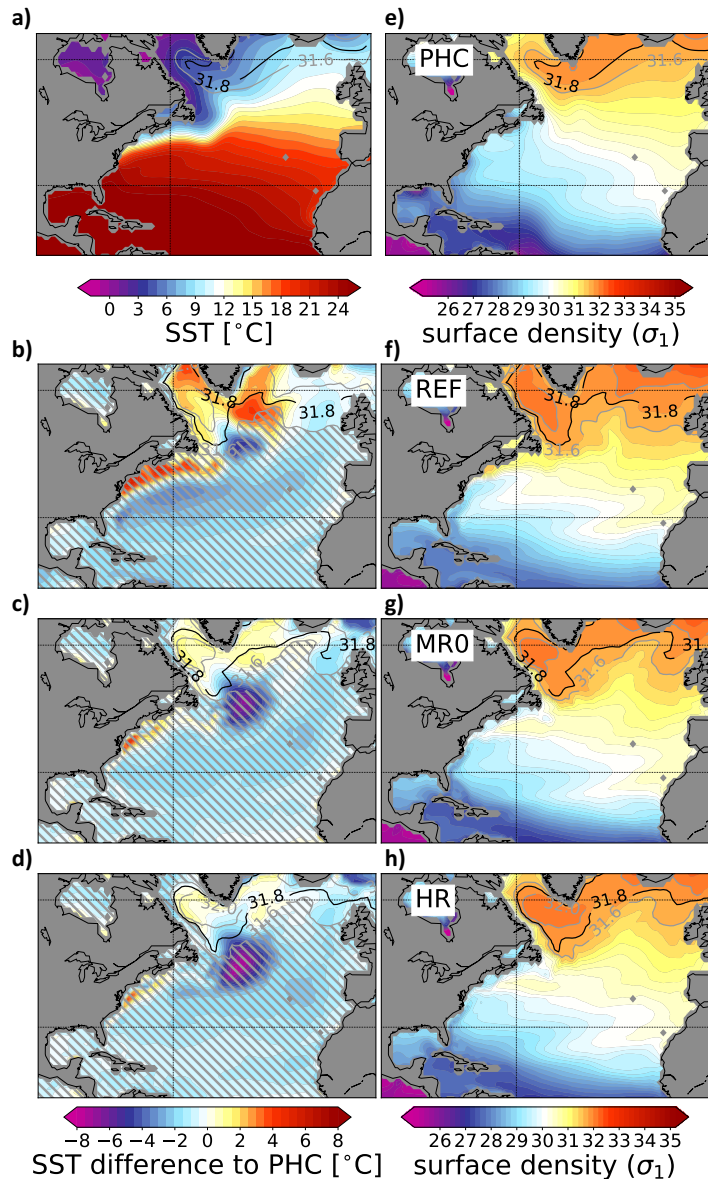
Figure 7. a) The North Atlantic sea surface temperature and e) \sigma_1 -density structure at the ocean surface, as determined from the PHC climatology (PHC 3.0, updated from: Steele et al., 2001). Black and gray contours indicate outcropping areas for typical isopycnal surfaces found in the deep ocean around 1000 m (e.g. \sigma_1 = 31.8 ). f)–h) Same for the simulated density structure in REF, MR0, and HR (years 71–100). b)–d) Sea surface temperature (SST) biases in the 3 simulations (years 71–100) with respect to PHC in Fig. 7a. Three simulated \sigma_1 -density contours that represent the 'mapping' to deeper ocean layers are overlaid with black and gray contours (identical to the contour levels in Fig. 7f–h). To highlight the SST improvements in the areas encircled by these contours, hatching grays out regions that are not in contact with the deep ocean around 600–1000m.
