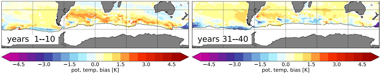
Figure 11. Southern Ocean maps of along-isopycnal potential temperature biases [K] in a) LR and b) HR for years 1–10 and 31–40. Black contours show the outcropping location of the \sigma_1=31.8 isopycnal. For animations of the bias development with a 10-yr running window, see supplementary animations S1 and S2 (Rackow et al., 2018b).
