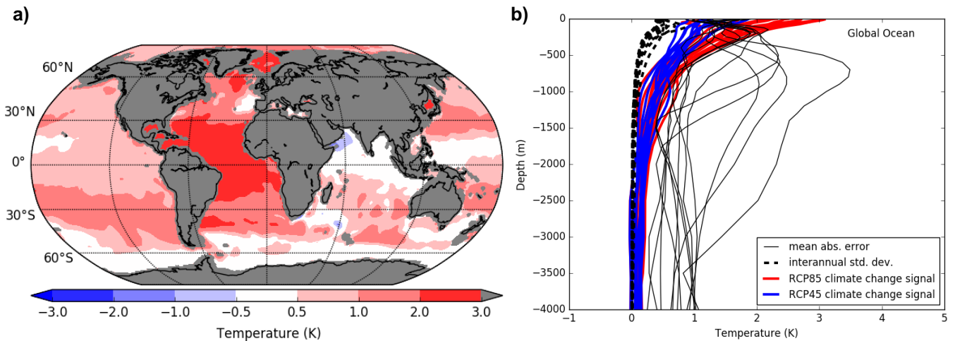
Figure 1. Biases in CMIP5 models with respect to the PHC climatology (PHC 3.0, updated from: Steele et al., 2001). a) Ensemble mean DJF potential temperature bias [K] at a depth of 1000 m in CMIP5 historical simulations for the period 1971–2000. b) Individual depth-profiles of the mean absolute potential temperature error in the CMIP5 models (black lines). The interannual standard deviation [K] (black dashed lines) and the RCP4.5 and RCP8.5 climate change signal [K] (2071–2100 minus 1971–2000; blue and red lines) are given for comparison.
