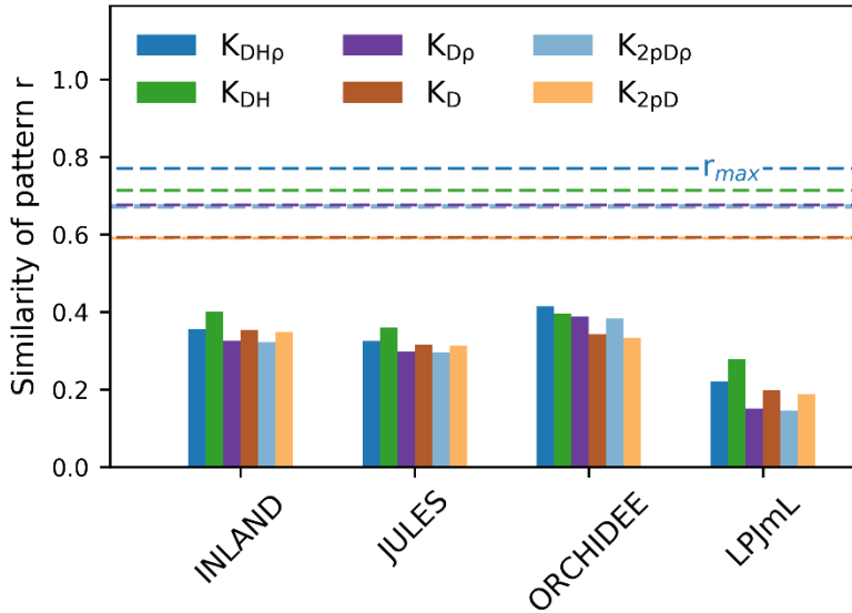
Figure 5: The similarity of the observed vs. simulated spatial pattern of AGB at pixel scale (as indicated by r given in bars). The similarity is calculated for different versions of observed AGB derived from six allometric equations (indicated by the colors, see Tab. S1). The dashed line shows the maximum achievable correlation coefficients r_{max} from the observational data and for the different allometric equations.
