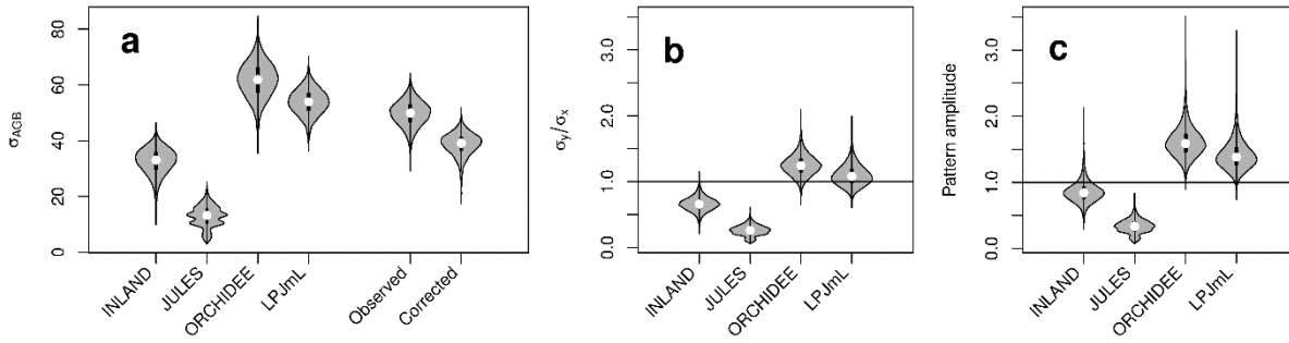
Figure 4: (a) Standard deviations of AGB (in MgC/ha) for the four models and observational data (for the other allometric equations see also Table S2, S3). For the observational data, the global variability at point scale (“observed”) and the corrected variability at pixel scale (“corrected”) is given; (b) ratio of standard deviations without correcting for within-pixel variability, (c) corrected metrics of pattern amplitude ( \sigma_y/\sigma_{x,corr} ).
