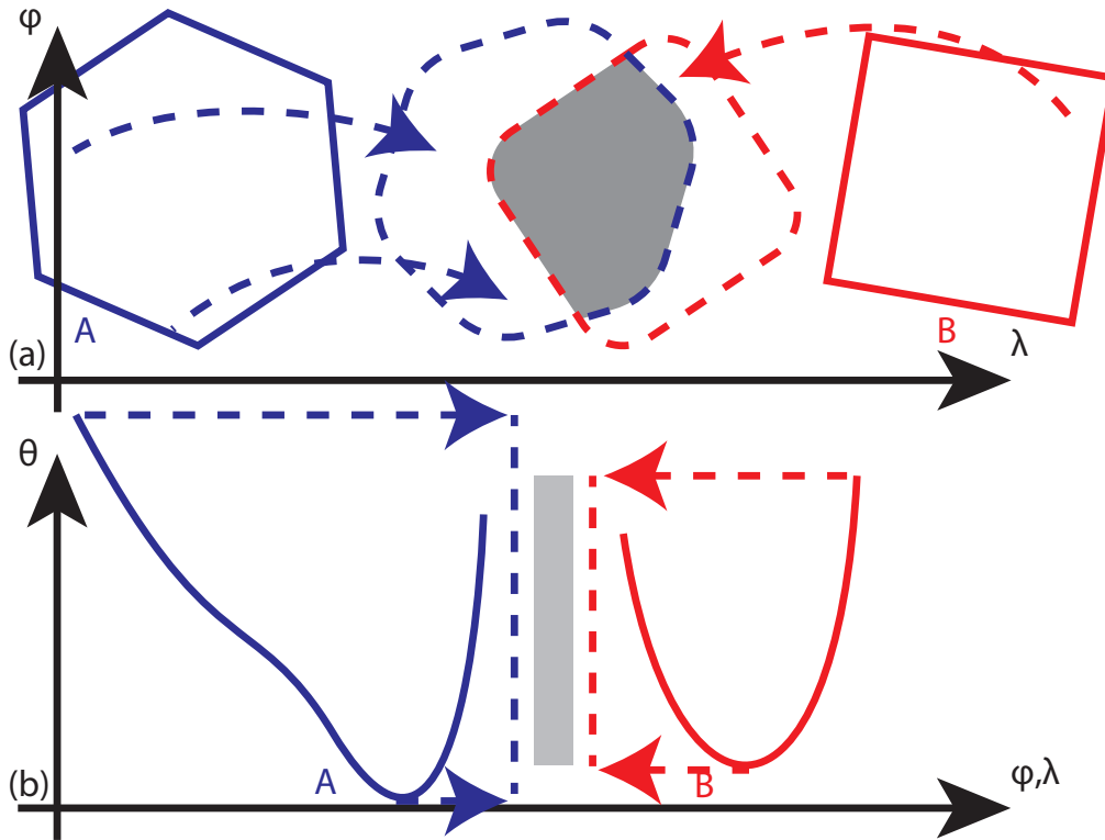
Figure 2. Schematic for the (a) horizontal and (b) vertical components of time correspondence similarity quantified by overlap (gray) of a basin A at t_0 (blue) and basin B at t_0 + \Delta t (red) at the intermediate half-time (dashed). (a) For the horizontal, each cell in the basin is advected, and overlap occurs in the common cells. (b) For the vertical, the potential temperature range [\theta_{min}, \theta_{max}] of each basin is held constant, and overlap is the one-dimensional intersection of the ranges.
