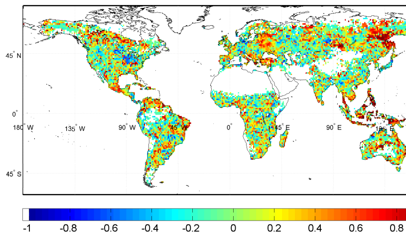
Figure 12. Correlation of annual BF from GFED and SEVER, over 1997-2006.
