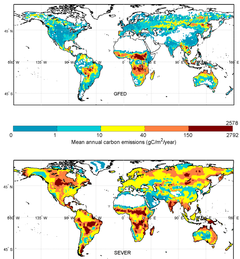
Figure 9. Mean Annual emissions (gC/m 2 /year) over 1997-2006. Top: GFED; Bottom, SEVER-FIRE.
