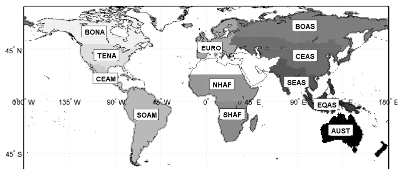
Figure 13. Regions used for inter-annual variability analysis. BONA: Boreal North America; TENA: Temperate North America ; CEAM: Central America ; SOAM: South America ; EURO: Europe ; NHAF: Northern Hemisphere Africa ; SHAF: Southern Hemisphere Africa ; BOAS: Boreal Asia ; CEAS: Central Asia ; SEAS: South East Asia ; EQAS: Equatorial Asia ; AUST: Australia.
