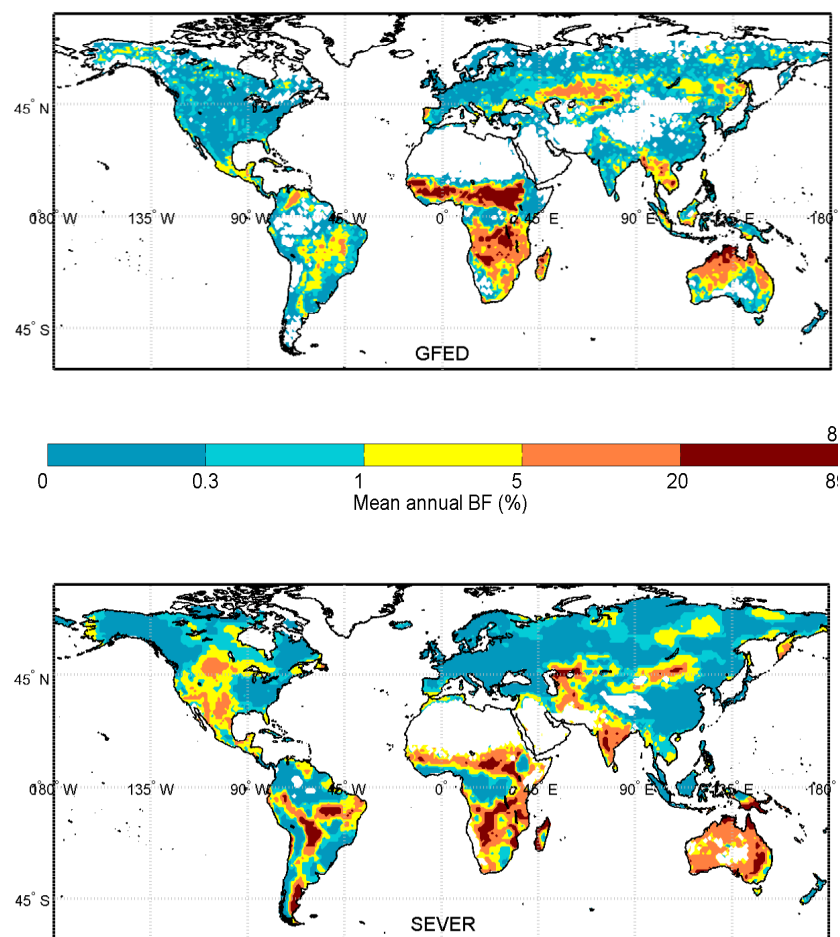
Figure 5. Mean Annual Burned Fraction (percentage) over 1997-2006. Top: GFED; Bottom, SEVER-FIRE.
