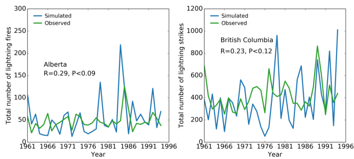
Figure 2. Total number of lightning fires observed (Wierzchowski et al., 2002) and simulated. Left: in Alberta; Right: in British Columbia.
