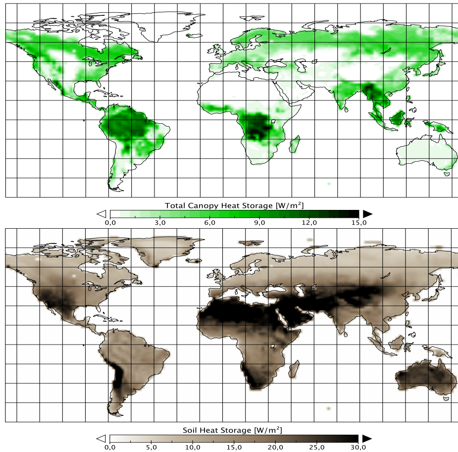
Figure 4. Comparison of Canopy and Soil Heat Storage: Global distribution of the positive contributions of the Canopy Heat Storage S_{\text{canopy}} (upper panel) and the Soil Heat Storage S_{\text{soil}} (bottom panel), both in \text{W/m}^2 as a thirty-year mean (1979-2008).
