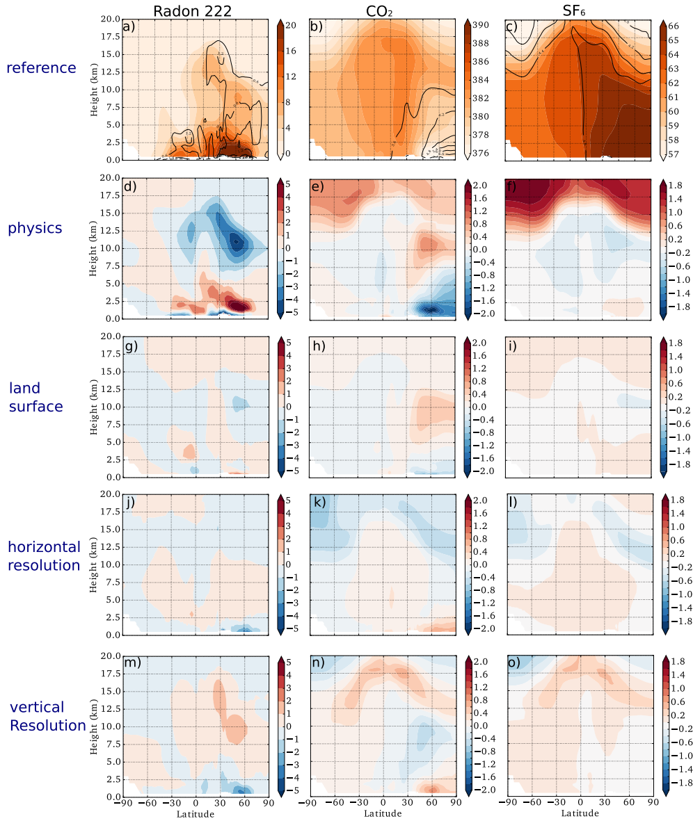
Figure 3. Zonal-mean mole fraction of (a) ^{222}\text{Rn} in 10^{21}\text{mol/mol} , b) \text{CO}_2 in ppm, (c) \text{SF}_6 in 0.1 ppt from 5A-96L39. The standard deviation is superimposed with contour lines. (d-f) Zonal-mean mole fraction difference between 6A-96L39 and 5A-96L39 (effect of the new physics). (g-i) As (d-f) but between 6A-96L39 and 6AWOR-96L39 (effect of the land surface model ORCHIDEE). (j-l) As (d-f) but between 6A-144L39 and 6A-96L39 (effect of the horizontal resolution). (m-o) As (d-f) but between 6A-144L79 and 6A-144L39 (effect of the vertical resolution). The zonal mean is calculated for afternoon hours from 2005 to 2010 in summer (JJA).
