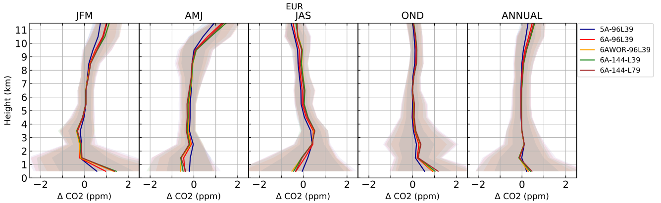
Figure 11. Same as for Figure 10 but over Europe from the CONTRAIL dataset during the period 2006-2011. The domain is portrayed in Figure 2.
