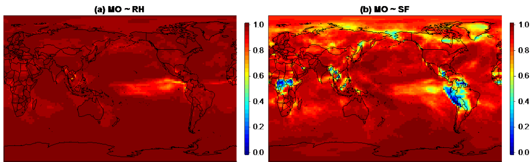
Figure 7: R^2 values calculated at every grid-cell (for the full 1991 – 2015 MDA8 O_3 JJA time series) 5 for MO and RH (left) and MO and SF (right).
