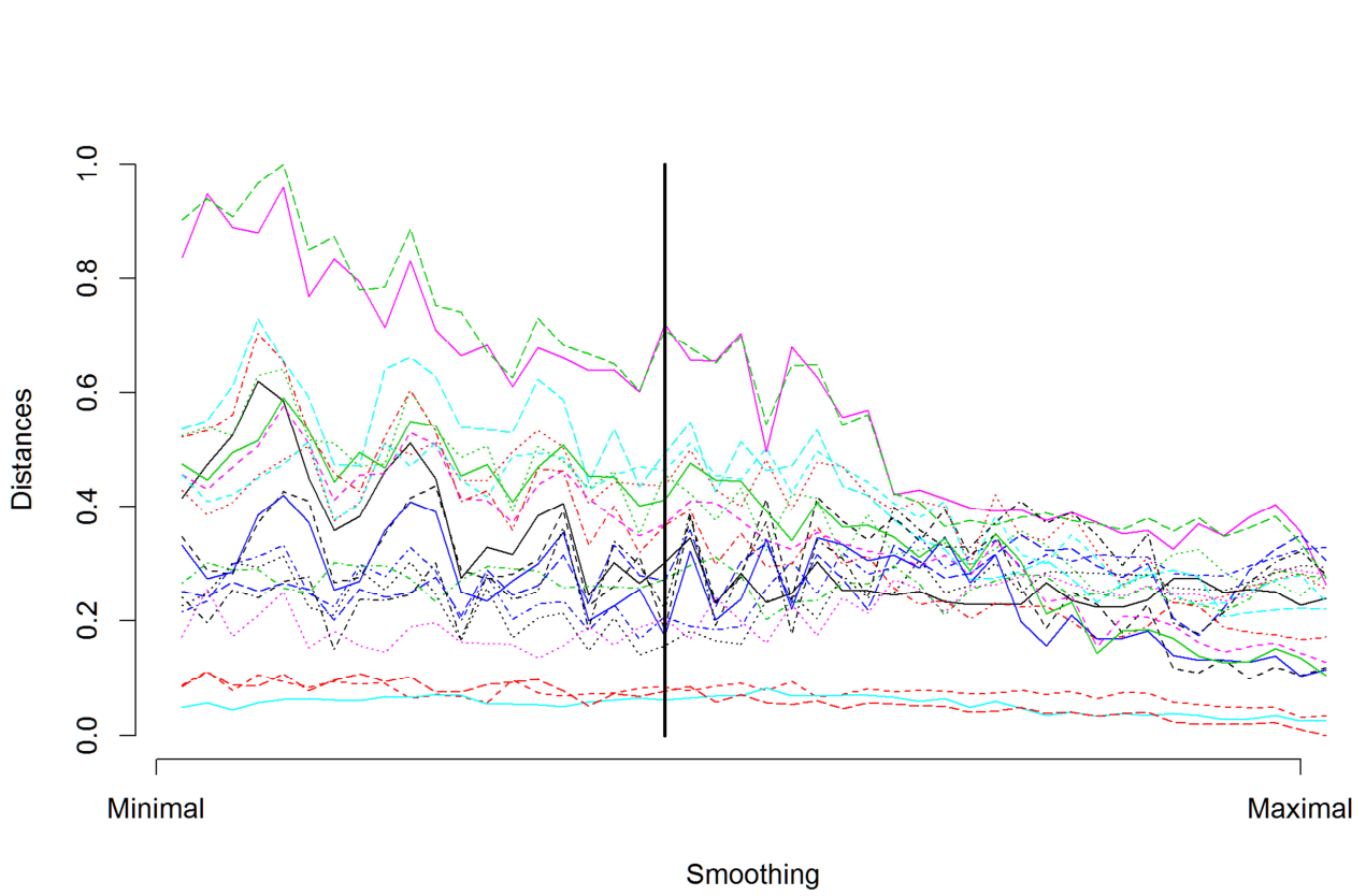
Figure 5. The same as Fig. 4, but for distances d_1 .
