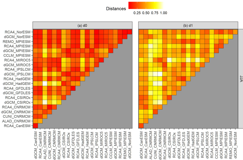
Figure 75. The same as Fig. 64, but for running 30-year mean relative changes in summer (JJA) mean precipitation over Eastern Europe region (the curves shown in Fig. 2b, underlying data in Fig. 2a).
