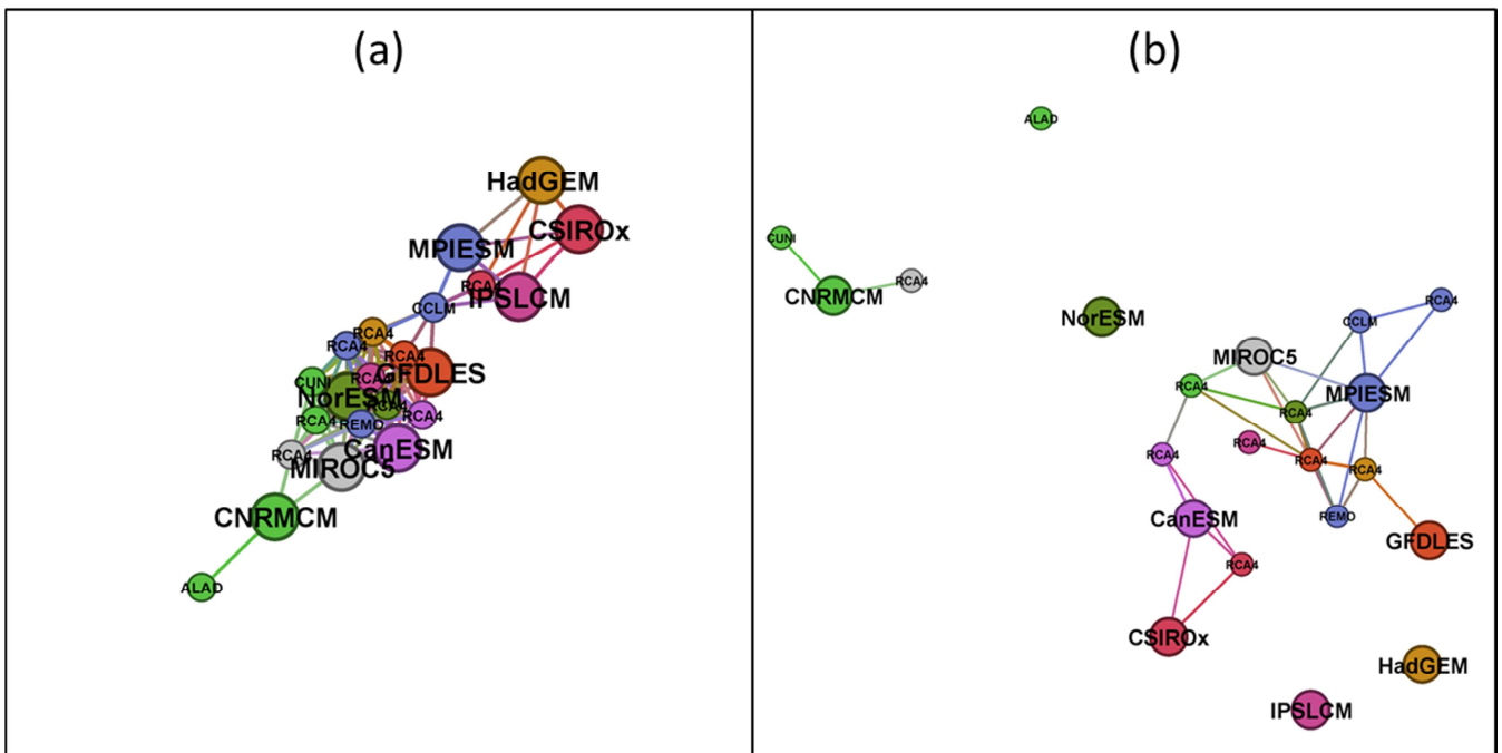
Figure 108. The same as Fig. 79, but for running 30-year mean relative changes in summer (JJA) mean precipitation over Eastern Europe region (underlying similarity matrices in respective panels of Fig. 75).
