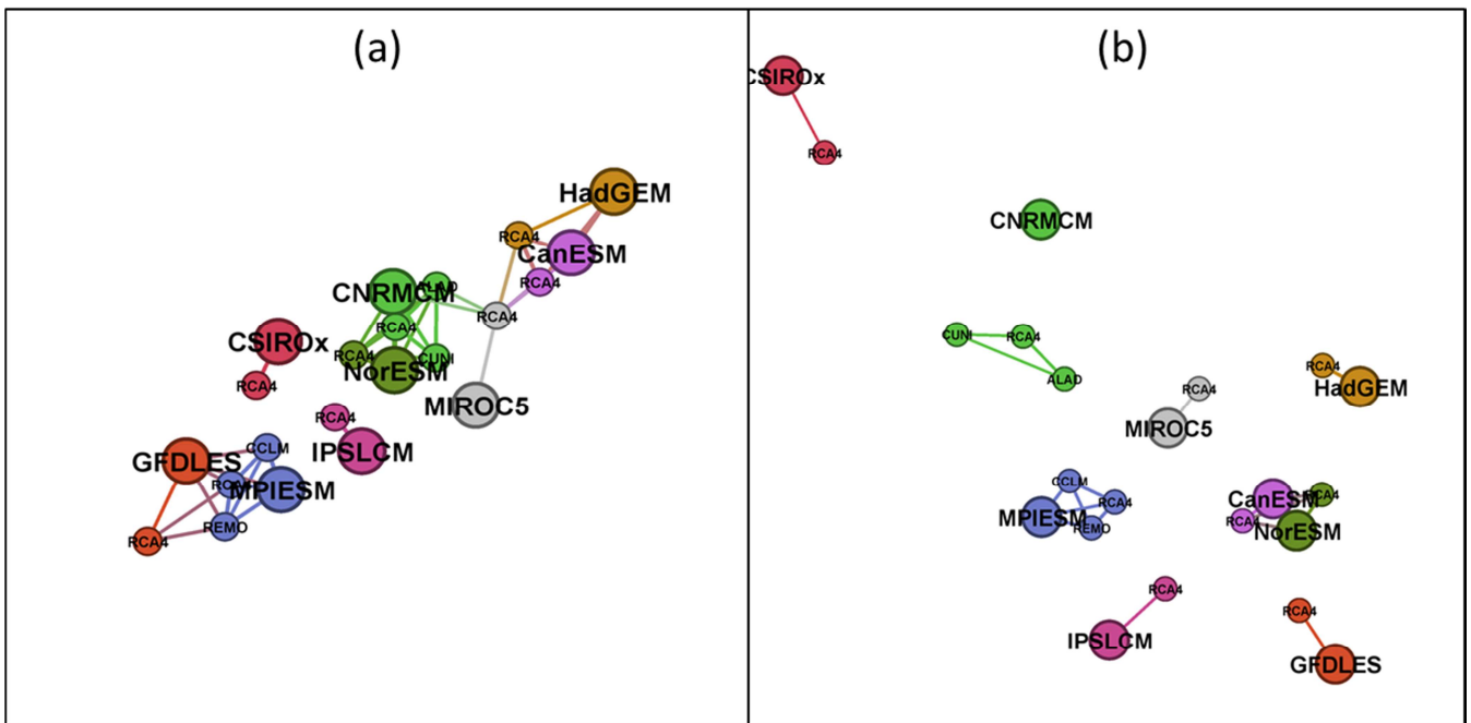
Figure 27. (a) Layout graph based on d_0 distances for running 30-year mean changes in winter (DJF) mean air temperature over the British Isles (underlying similarity matrix in Fig. 64a). (b) The same as (a), but for d_1 distances (underlying similarity matrix in Fig. 64b).
