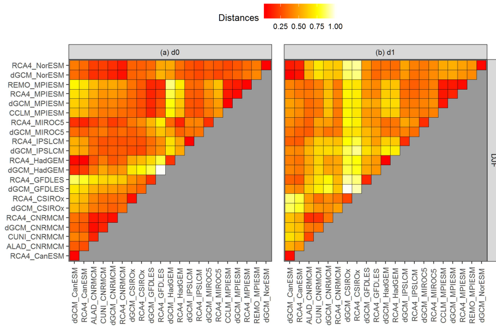
Figure 64. (a) Heatmap of the d_0 distances for running 30-year mean changes in winter (DJF) mean air temperature over British Isles (the curves shown in Fig. 1b, underlying data in Fig. 1a) with redder colour for larger similarity, brighter colour for smaller similarity between 5 respective curves. The values of the semimetric d_0 are scaled to the interval [0,1]. The acronyms of the model simulations are explained in Sect. 2. The definition of the distances is explained in Sect. 3.1. (b) The same as (a), but for d_1 distances.
