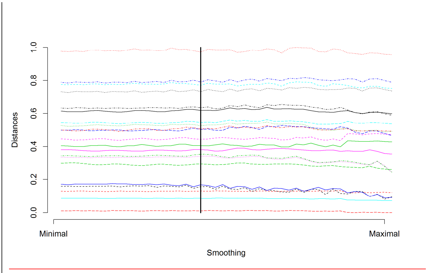
Figure 4. Normalized d_0 distances between simulated air temperature curves (data shown in Fig. 1a) of randomly selected model and other models in dependence on amount of smoothing. Starting values represent d_0 distances between original curves, values at the end represent d_0 distances for oversmoothed data. The vertical line depicts the amount of smoothing used in the presented study.
