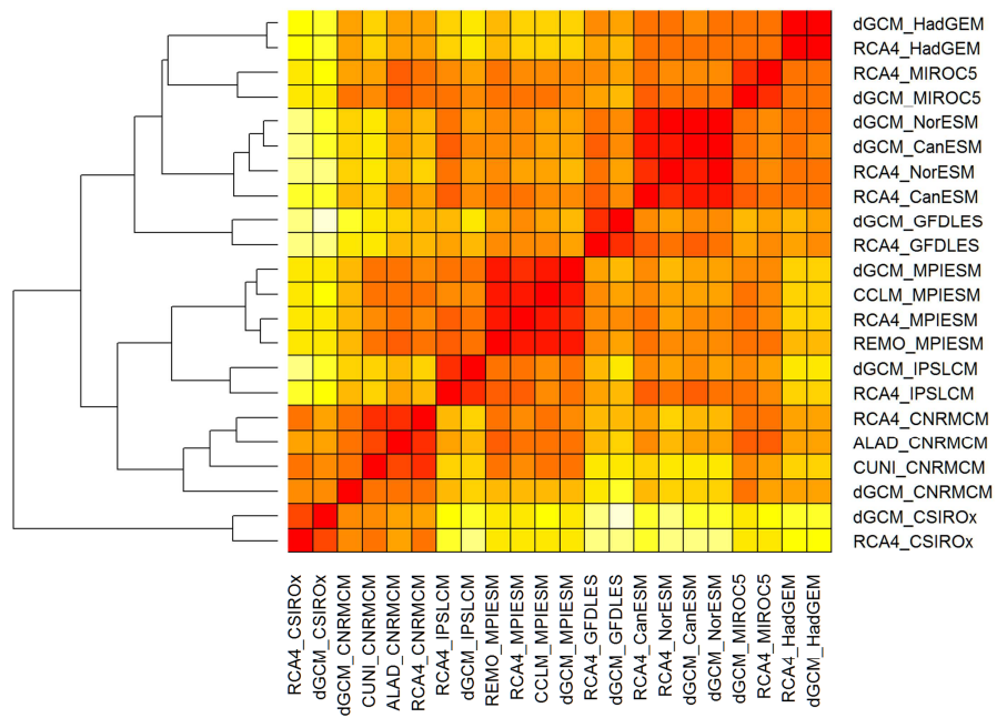
Figure 86. An example of the dendrogram resulting from hierarchical cluster analysis based on d_1 distances for running 30-year mean changes in winter (DJF) mean air temperature over British Isles (underlying similarity matrix in Fig. 64b).
