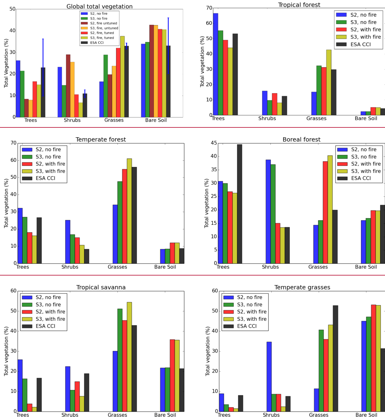
Figure 5: Present day (2014 5 ) total vegetation cover (percentage) globally (top left), and by WWF biome (5 out of 8 shown here: tropical forest, temperate forest, boreal forest, tropical savanna, and temperate grasses. Tundra, Mediterranean wood and desert not shown). Trees = total broadleaf and needleleaf trees, grasses = total C3 and C4 grasses. Top left panel includes results prior to tuning, plus uncertainty bars for the ESA observations of vegetation cover shown in blue.
