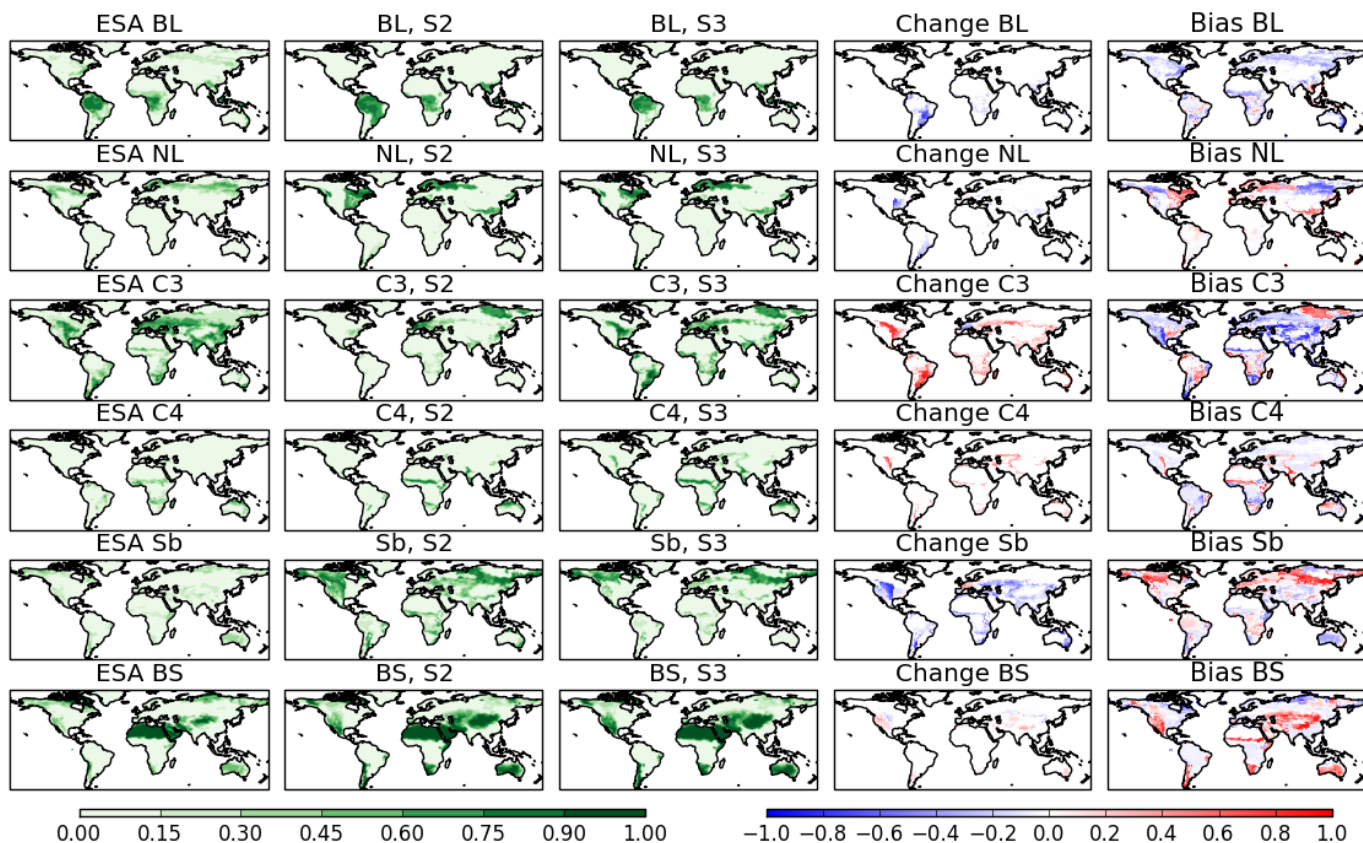
Figure 1: Present day (2014 5 ) vegetation fractions for the TRENDY S2 ( without LULCC , no fire ) and S3 experiment ( with LULCC , LULCC only ) by PFT, without fire, compared to observations. Left column shows ESA CCI observations (2010), second column shows vegetation without LULCC (S2), third column shows vegetation with LULCC (S3), fourth column shows the change resulting from LULCC (difference between column 2 and 3), and right column shows bias of S3 compared to observations (difference between column 1 and 3). BL = broadleaf, NL = needleleaf, C3 = C3 grasses, C4 = C4 grasses, Sb = shrub, BS = bare soil.
