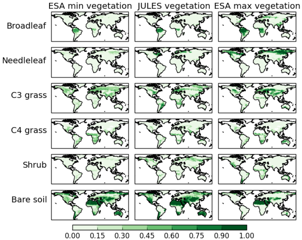
Figure 4: Present day (2014) vegetation fraction PFT, as modelled by JULES -INFERN0- with LULCC and fire (SF3, central column), compared to the range of uncertainty from ESA CCI observations (V1, 2010) (Minimum fractions left column, maximum fractions right column). Top row = broadleaf, second row = needleleaf, third row = C3 grass, fourth row = C4 grass, fifth row = shrub, sixth row = bare soil.
