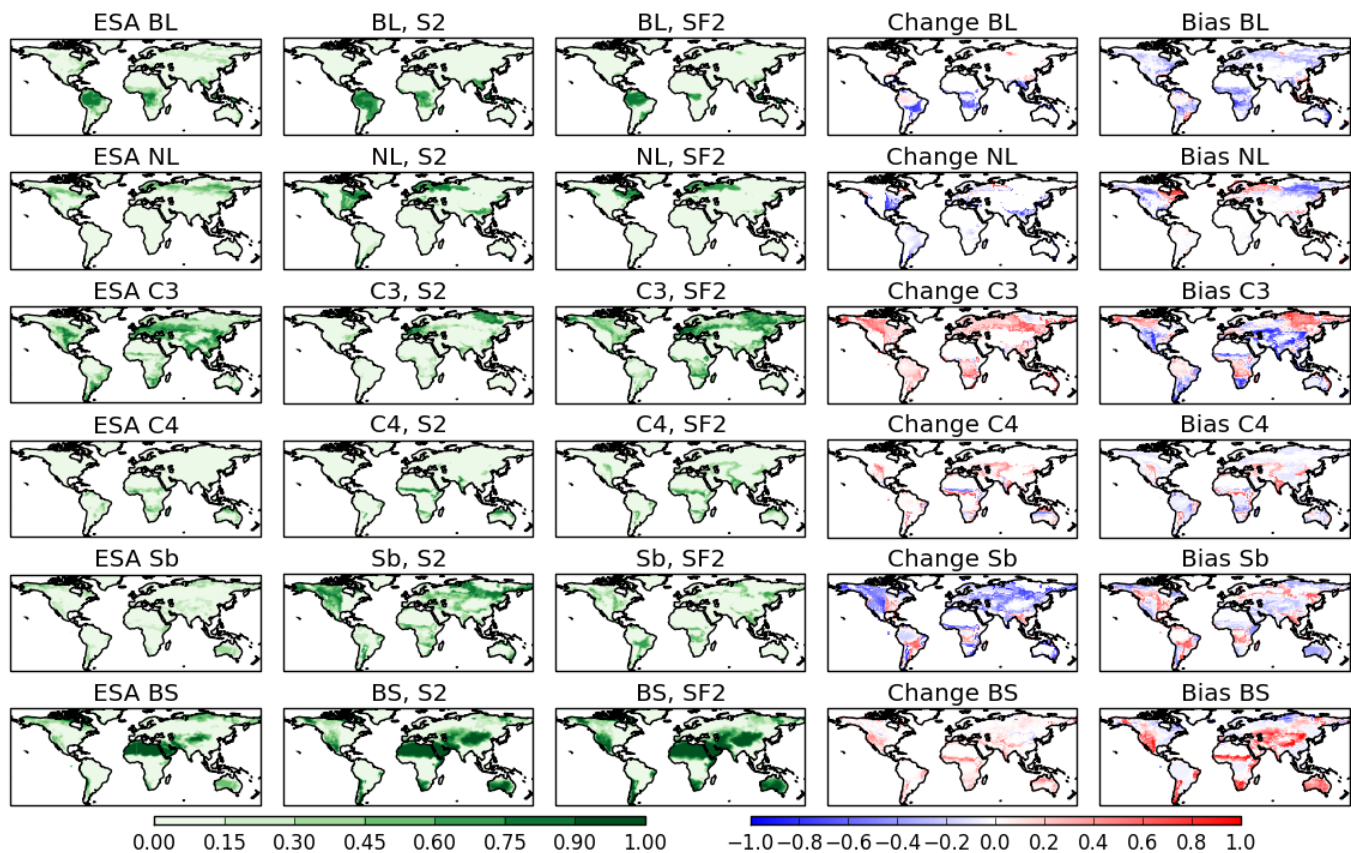
Figure 3: Present day (20145) vegetation fractions for the TRENDY S2 experiment (no LULCC, no fire) and SF2 (fire only) by PFT compared to observations. Left column shows ESA CCI observations (2010), second column shows vegetation without fire or LULCC (S2), third column shows vegetation with fire only (SF2), fourth column shows the change resulting from fire (difference between column 2 and 3), and right column shows the bias of SF2 compared to observations (difference between column 1 and 3). BL = broadleaf, NL = needleleaf, C3 = C3 grasses, C4 = C4 grasses, Sb = shrub, BS = bare soil.
