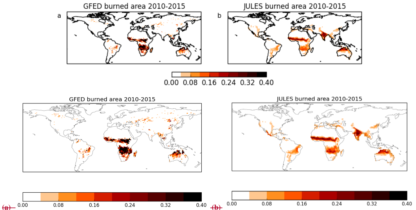
Figure 2: Average 2010-2015 burned area from GFED 4.1s observations (a) and as modelled by JULES-INFERNO (b)
