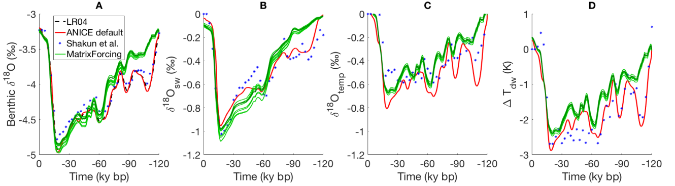
Figure 12: A) modelled benthic oxygen isotope abundance from the default ANICE model (de Boer et al., 2014) and the LGM benchmark experiment compared to different datasets (LR04, Shakun et al. (2015)). B) \delta^{18}O of seawater due to depletion of heavy isotopes. C) contribution to benthic oxygen isotope abundance due to changes in deep-water temperature. D) derived deep-water temperature anomaly.
