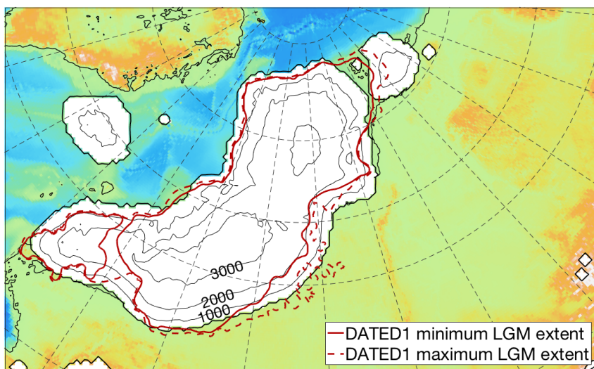
Figure 10: Comparison of the larger simulated Eurasian ice-sheet at LGM with the DATED-1 reconstruction (Hughes et al., 2016). Contour lines show ice thickness. The modelled ice-sheet has a volume of 24 m sea-level equivalent, in agreement with the DATED-1 ice-sheet.
