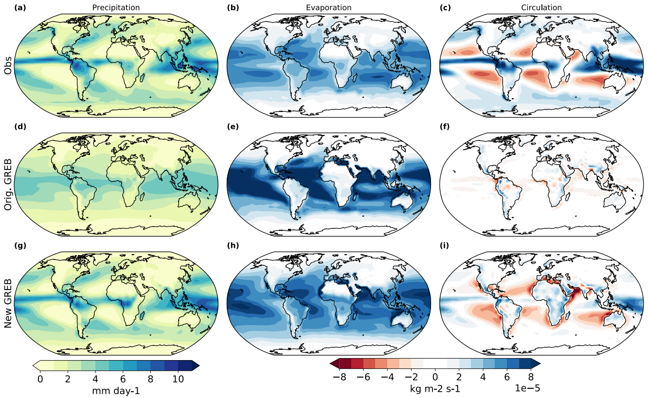
Figure 2: The decomposition of the hydrological cycle into its parts precipitation in mm/day (left column), evaporation (middle column) and circulation in kg/m 2 /s (right column) in observations (upper row), the original GREB model (middle row) and the new GREB model (lower row) for the annual mean.
