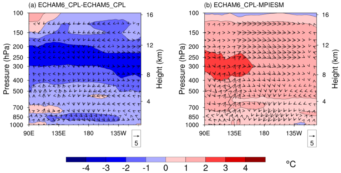
Figure 13: Simulation differences in the vertical structure of atmospheric circulation and the temperature over the SEC area: (a) between ECHAM6-NEMO3.6 and ECHAM5-NEMO3.6, (b) between ECHAM6-NEMO3.6 and MPI-ESM. Vector units: m/s, contour unit: °C.
