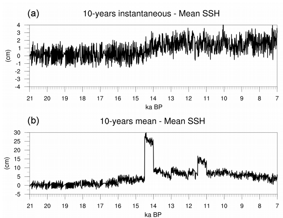
Figure 11: Time series of (a) 10-years instantaneous; and (b) 10-years averaged mean SSH (cm) during the test simulation with MPI-ESM.
