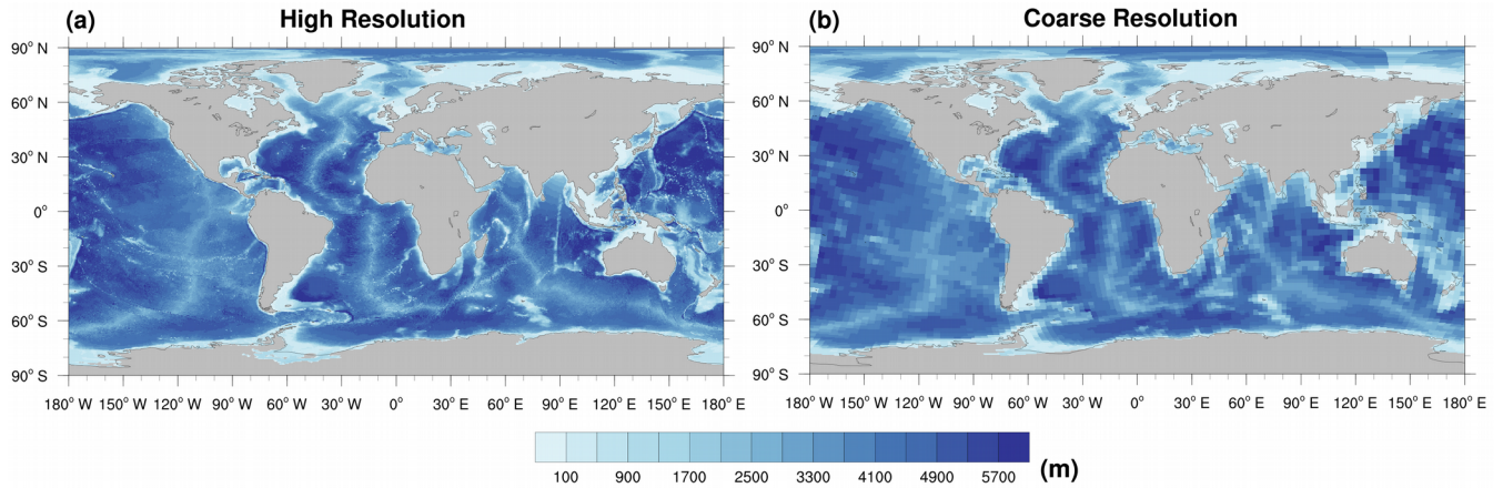
640 Figure 2: Present-day global ocean bathymetry (m) and land-sea mask for (a) the high resolution (HR, 10' x 10') dataset; and (b) the generated coarse resolution (GR30) grid for running MPIOM.
