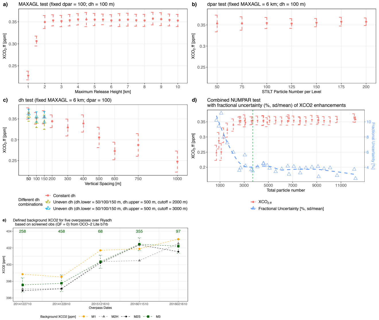
Figure 6. Results of sensitivity tests for one sounding (a-d) and background comparisons for 5 tracks (e) over Riyadh. Random error for each simulation is indicated as dashed red error bars (a-d); and potential biases are shown as the trend of the mean XCO 2 enhancements (red dots; a-d) derived from 100 times of bootstrap. c) Vertical spacing tests include several tests with constant dh (red dots and error bars) and two tests with uneven dh above/below the cutoff level. Two uneven dh tests both use three different lower dh (50, 100 and 150 m) and a fixed upper dh of 500 m, but with two different cutoff levels, i.e., 2 km (yellow triangles and error bars) and 3 km (blue triangles and error bars). d) A summary plot of mean and SD of XCO 2 enhancements (red dots and dashed red error bars) and fractional uncertainties (% , sd/mean) as functions of total particle number (NUNPAR). Green dashed vertical line denotes the configuration used in this study. e) Background comparisons using different methods (M1, M2H, M2S, and M3) for 5 tracks. The amounts of screened observations used for M3 background are labeled in dark green. M3 background errors (including spatial variation and retrieval errors over the background region) are indicated as dashed green error bars.
