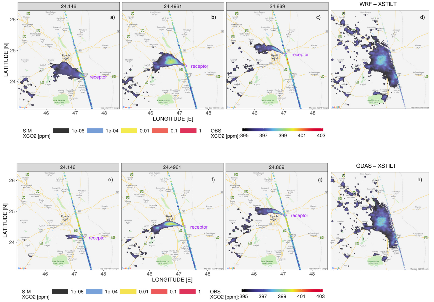
Figure 7. Spatial maps of 1 km \times 1 km modeled XCO_2 contributions (ppm; log-scale) from 3 selected soundings along with screened observations (QF = 0) on 1000UTC 12/29/2014 over Riyadh, with meteorological fields driven by WRF (a-d) and GDAS (e-h). Panel d and h denote the latitude-integrated XCO_{2,ff} contributions (with weights of receptor spacings, e.g., 0.02^\circ ) using WRF and GDAS, derived from spatial XCO_2 enhancements for over 60 column receptors along each overpass. The sum of the latitude-weighted spatial XCO_2 enhancements over all gridcells (in panel d or h) equals to the latitude-integrated XCO_{2,ff} signal (ppm-degree) reported in Sect. 3.5. Only large enhancements > 10^{-6} ppm are plotted.
