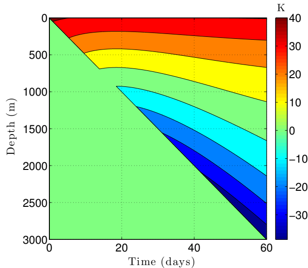
Figure 13. Temperature change \Delta T_a at the borehole wall while drilling a 3 km borehole through the example sedimentary sequence (Fig. 8) over a 60 day period. This thermal disturbance is used to establish the boundary condition at the borehole wall during drilling.
