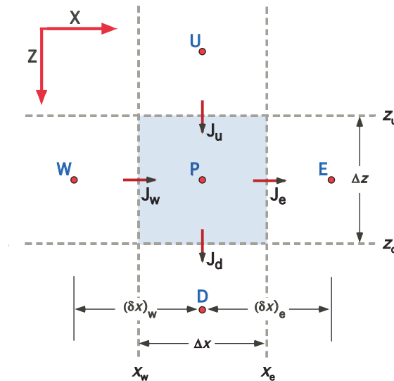
Figure 7. Schematic showing the nomenclature associated with a control-volume centered on grid point P for 2-D cartesian (XZ) coordinates. The control-volume is bounded by interfaces located at x_w , x_e , z_u , and z_d , through which enthalpy fluxes J_w , J_e , J_u , and J_d pass. Grid points W, E, U, and D are located at the center of the neighboring CVs. The nomenclature for 2-D cylindrical coordinates is completely analogous with R replacing X. Three dimensional (3-D) cartesian coordinates introduces an additional axis (Y) with neighboring grid points S and N.
