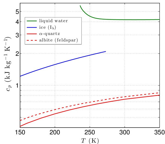
Figure 1. Variation of the specific heat with temperature for liquid water, ice, and two common minerals (quartz, albite).
