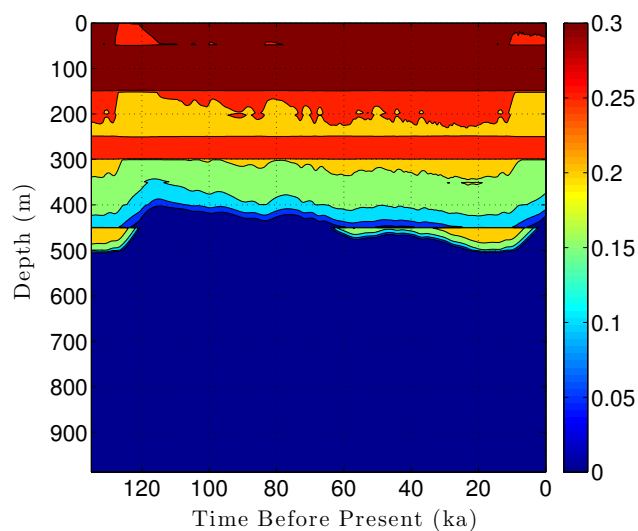
Figure 10. Ice content \phi_i variations over the last ice-age cycle within the example sedimentary sequence (Fig. 8). Unfrozen water \phi_e variations mirror the ice content fluctuations.
