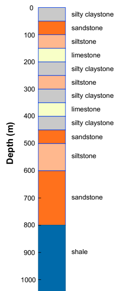
Figure 8. Vertical sequence of sedimentary rocks used for the permafrost example simulations.
