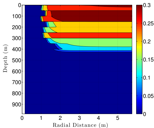
Figure 14. Volumetric ice content \phi_i in the sedimentary sequence (Fig. 8) penetrated by a newly completed 3 km deep borehole. Radial distance is measured from the central axis of the borehole.
