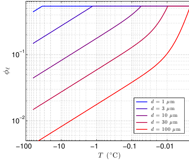
Figure 2. Sensitivity of the volume fraction of liquid water \phi_\ell to particle diameter d with \lambda = 0.36 \mu\text{m K}^{1/3} and T_f = 273.15 \text{ K} . The porosity, \phi = 0.54 in this example, sets the upper limit on \phi_\ell .
