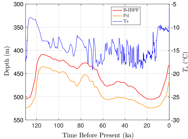
Figure 9. Upper boundary condition ( T_s ) used to explore the response of a sedimentary sequence (Fig. 8) to surface-temperature changes over the last ice-age cycle. Also shown are the depths for the base of permafrost ( P_d ) and the base of ice-bearing permafrost (B-IBPF).
