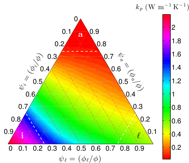
Figure 5. Variation of the pore thermal conductivity k_p on Earth at -10^\circ\text{C} with the relative volume fractions of liquid water ( \psi_\ell ), ice ( \psi_i ), and air ( \psi_a ) within the pores. Threshold \alpha is 0.75 in this example.
