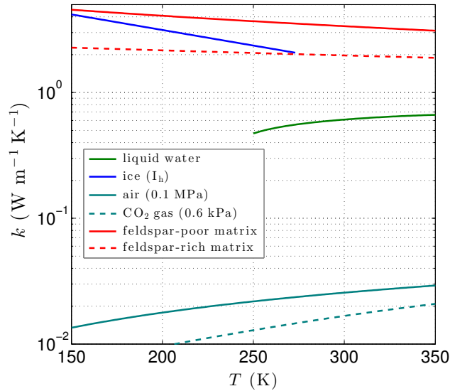
Figure 6. Variation of the thermal conductivity with temperature for liquid water, ice, air (terrestrial atmosphere), CO 2 gas (Martian atmosphere), and magmatic/metamorphic matrix minerals with k_m^o = 3.5 \text{ W m}^{-1} \text{ K}^{-1} (feldspar-poor) and k_m^o = 2.0 \text{ W m}^{-1} \text{ K}^{-1} (feldspar-rich).
