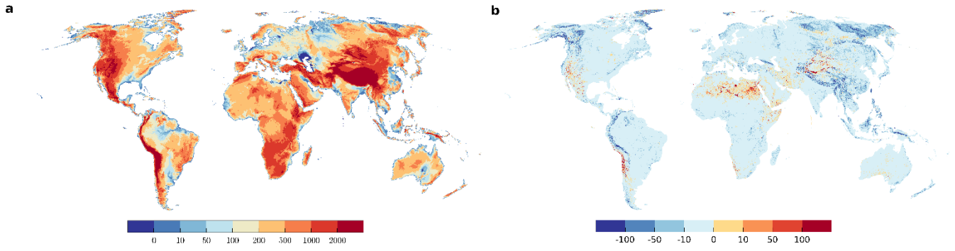
Figure 3 (a) Simulated equilibrium hydraulic head [ m ]. Maximum value 6375 m, minimum value -414 m (Extremes included in dark blue and dark red). (b) Difference between 30 th percentile of the 30'' land surface elevation per 5' grid cell (chosen elevation for surface water bodies) and simulated equilibrium hydraulic head. Maximum value 1723 m, minimum value -1340 m (Extremes included in dark blue and dark red).
