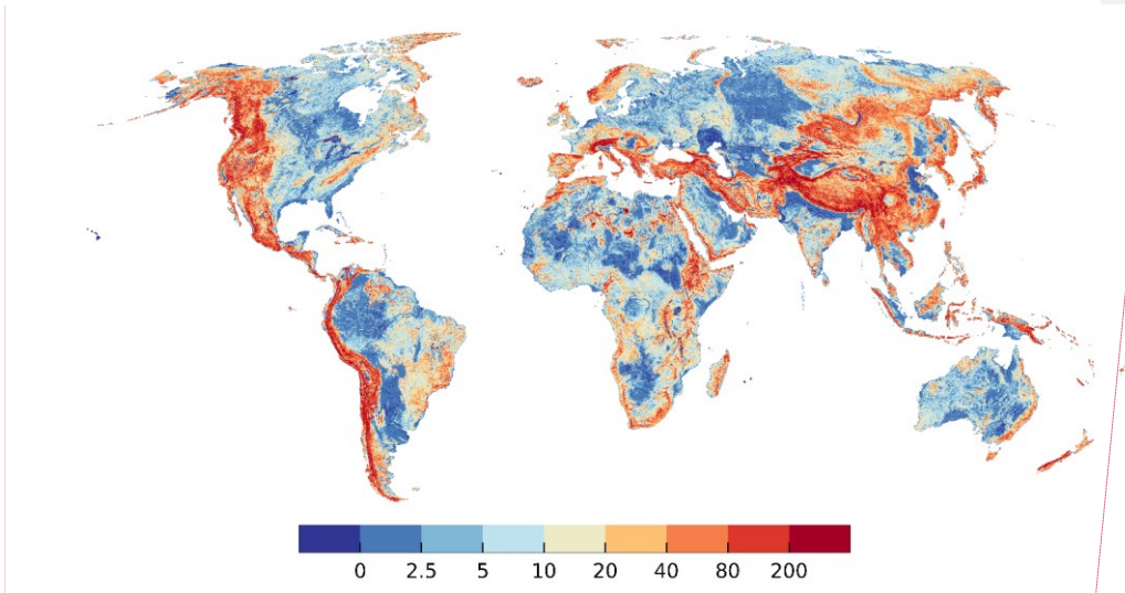
Figure S5 Arithmetic mean [ m ] of the 30" land surface elevation per 5' grid cell and simulated equilibrium hydraulic head (simulated depth to GW). Maximum value 2070 m, minimum value -414 m (Extremes included in dark blue and dark red).
