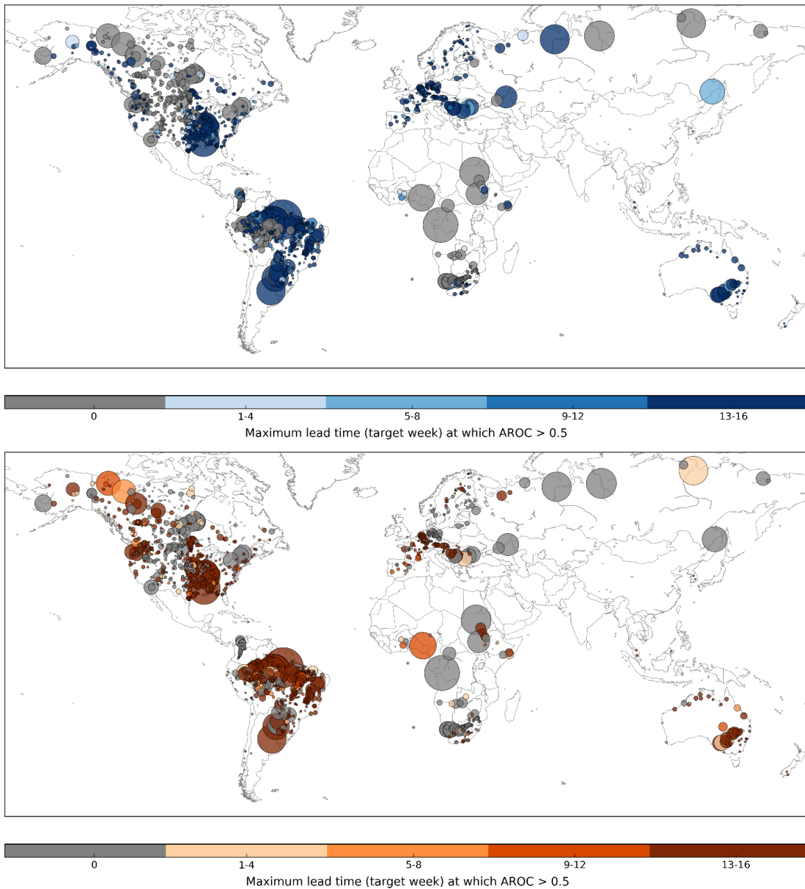
Figure 6: Maximum forecast lead time (target week, averaged across all months) at which the area under the ROC curve (AROC) is greater than 0.5 for high flow events (flow exceeding the 80 th percentile of climatology, top panel) and low flow events (flow below the 20 th percentile of climatology, bottom panel), at each observation station. This is used to indicate the maximum lead time at which forecasts are more skilful than the long-term average. Dot size corresponds to the upstream area of the location – thus larger dots represent larger rivers and vice versa. Grey dots indicate that (on average, across all months) forecasts are less skilful than climatology at all lead times.
