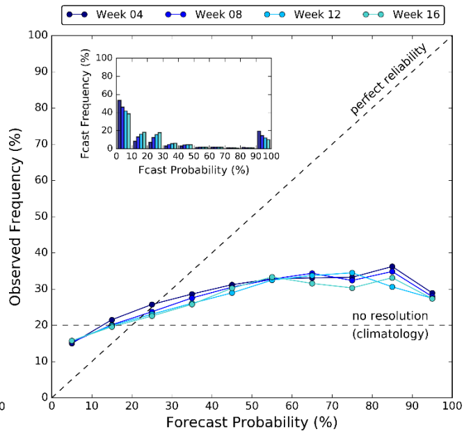
Figure 8: Attributes diagram for forecasts of low flow events (flow below the 20 th percentile of climatology, left) and high flow events (flow exceeding the 80 th percentile of climatology, right), aggregated across all observation stations globally. Results are shown for lead time weeks 4, 8, 12 and 16, and indicate the reliability of the forecasts. The histograms (inset) show the frequency at which forecasts occur in each probability bin, and are used to indicate forecast sharpness. Attributes diagrams for selected river basins are provided in the supplementary material.
