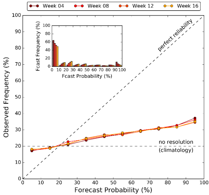
Figure 8: Attributes diagram for forecasts of low flow events (flow below the 20 th percentile of climatology, left) and high flow events (flow exceeding the 80 th percentile of climatology, right), aggregated across all observation stations globally. Results are shown for lead time weeks 4, 8, 12 and 16, and indicate the reliability of the forecasts. The histograms (inset) show the frequency at which forecasts occur in each probability bin, and are used to indicate forecast sharpness. Attributes diagrams for selected river basins are provided in the supplementary material.
