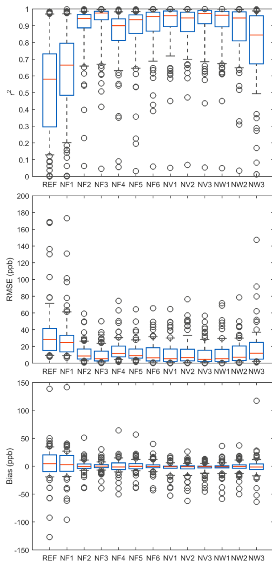
Figure 3 FLEXPART CTM model performance based on boxplots of coefficient of determination, RMSE and bias in daily average methane model fractions at surface stations for different kernel settings (see Table 1). Independent validation stations are included. The red line in the boxplots indicates the median, the bottom and top box edges are the 25th and 75th percentiles, and whisker ends are at 9th and 91st percentiles. The circles are outliers.
