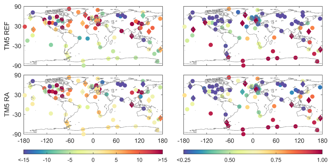
Figure 8 Bias (ppb, left) and r^2 (right) of modelled methane at all surface stations for TM5 (reference, top and reanalysis, bottom) simulations.
