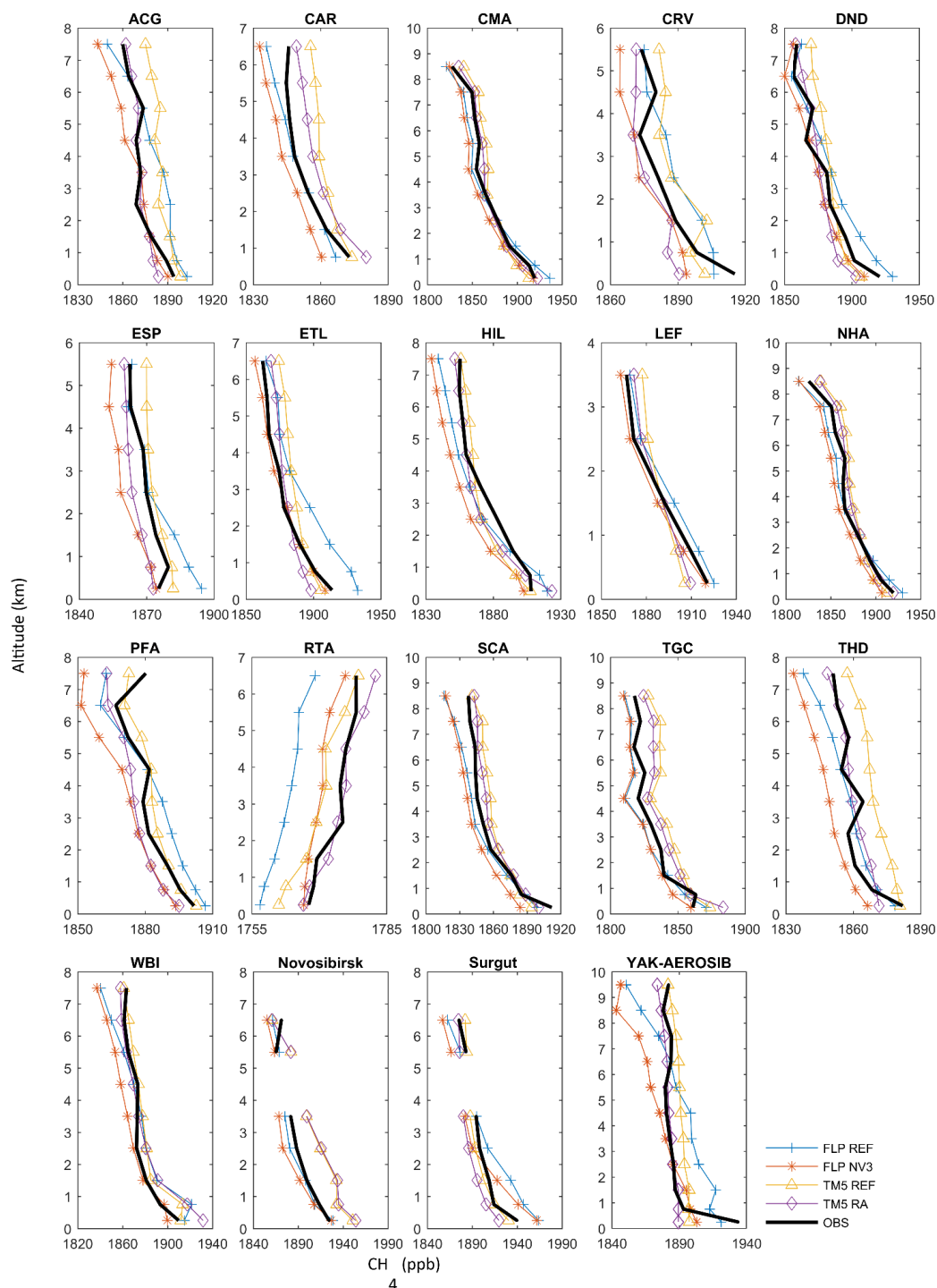
590 Figure 10 Averaged modelled and observed vertical profiles in 2013 at 16 NOAA locations, during the YAK-Aerosib campaign and at Surgut and Novosibirsk. FLP refers to FLEXPART CTM.
