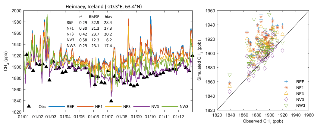
Figure 6 Methane (ppb) as observed and modelled at Heimaey in 2013 for a selection of FLEXPART CTM simulations, shown as time series (left) and scatter plot (right).
