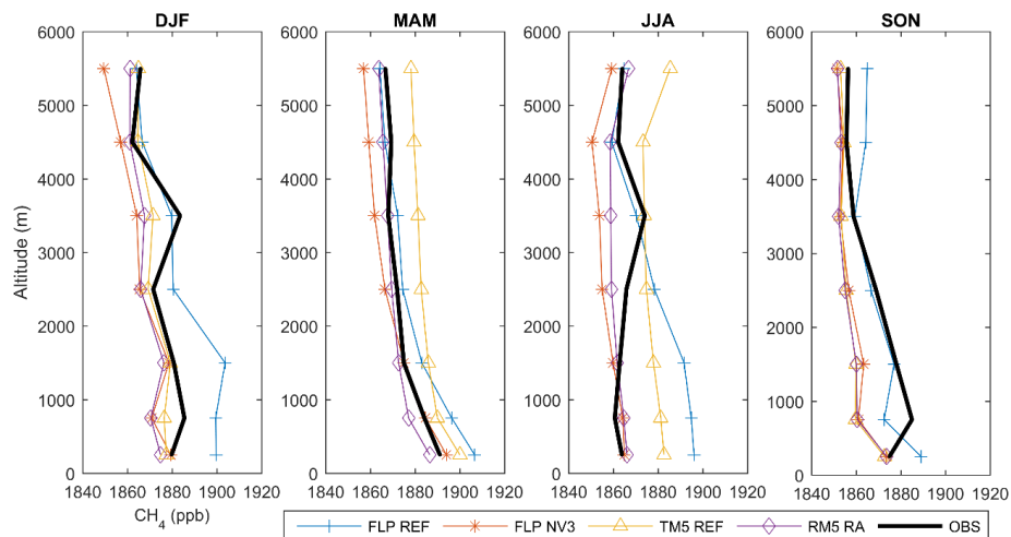
Figure 11 Seasonal observed and modelled methane profiles in 2013 at Estevan Point (Canada). FLP refers to FLEXPART CTM.
