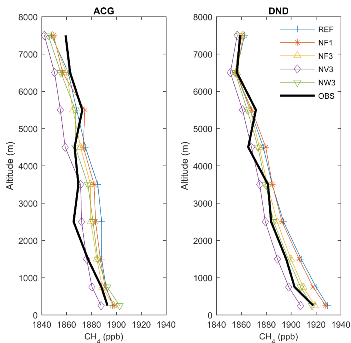
Figure 7 Averaged annual vertical methane profiles for 2013 based on monthly averaged data at NOAA profile locations ACG (Alaska Coast Guard, United States of America) and DND (Dahlen, North Dakota, United States of America). See Figure 1 for approximate profile locations.
