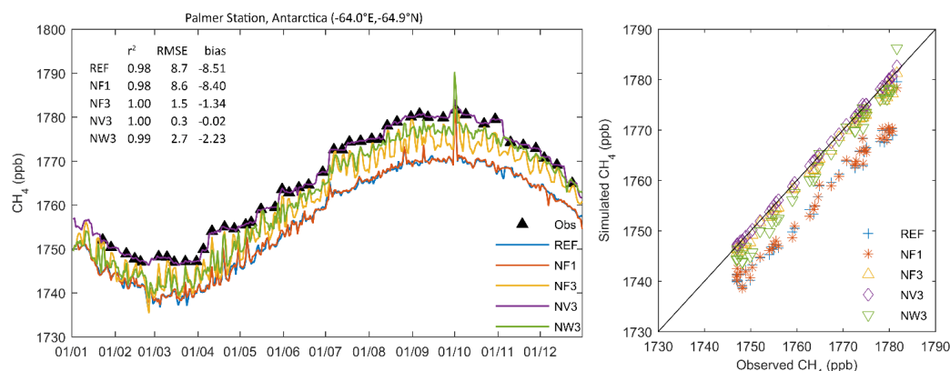
Figure 5 Methane (ppb) as observed and modelled at Palmer Station in 2013 for a selection of FLEXPART CTM simulations, shown as time series (left) and scatter plot (right).
