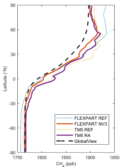
Figure 9 Zonal mean surface methane (ppb) in 2013 based on FLEXPART CTM, TM5 and GLOBALVIEW-CH4.
