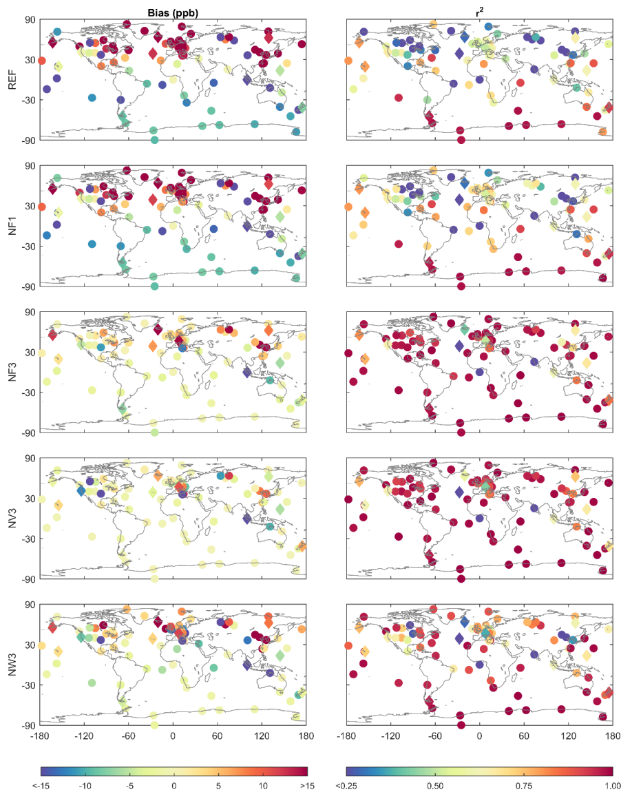
570 Figure 4 Bias and coefficient of determination of modelled methane at all surface stations, including validation stations (diamonds) for a selection of simulations (see Table 1 for settings). Some bias values exceed (-)15 ppb (also see Figure 3); colour limits were chosen to show the influence of nudging at the majority of stations.
