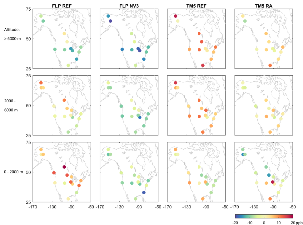
595 Figure 12 Model bias of FLEXPART CTM (abbreviated FLP) and TM5 at three altitude ranges for NOAA profiles in 2013 in North America.
