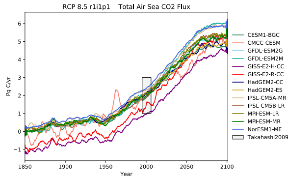
Figure 14. The total annual flux of CO 2 from the air to the sea in Pg/Year under the RCP8.5 scenario
