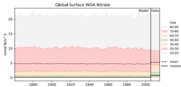
Figure 4. A plot produced by the time series package. The figure shows the time developers of many metrics at one: the mean, median and several percentile ranges of the observational data and the model data. In this case, the model data is the global surface mean nitrate in HadGEM2-ES in the historical simulation.
