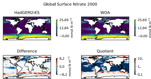
Figure 9. Four spatial distributions showing the model (top left), the observational data (top right), and the difference between them (bottom left) and their quotient (bottom right). The model data in these plots is the global surface nitrate in HadGEM2-ES in the historical simulation in ensemble member r1i1p1 in the year 2000. The observational data comes from the annual nitrate dataset in the World Ocean Atlas.
