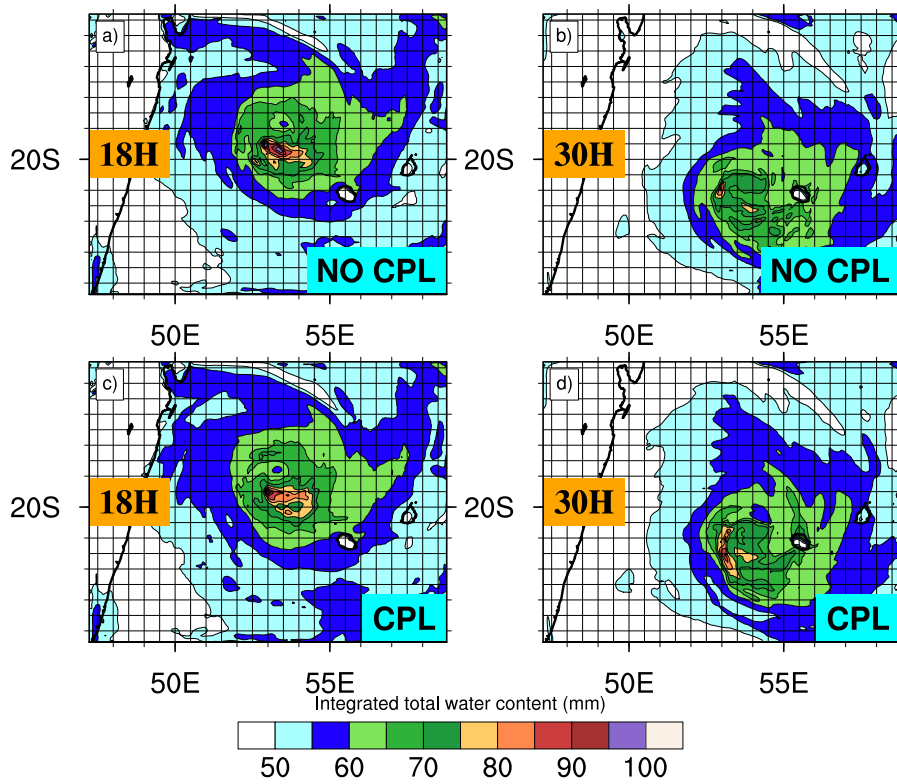
Figure 7. Total integrated water content in mm after 18h (a, c) and 30h (b, d) of simulation, respectively. Top panels (a, b) show results for the non coupled system (NO CPL i.e atmosphere only) and bottom panels (c, d) show results for the coupled system (CPL).
