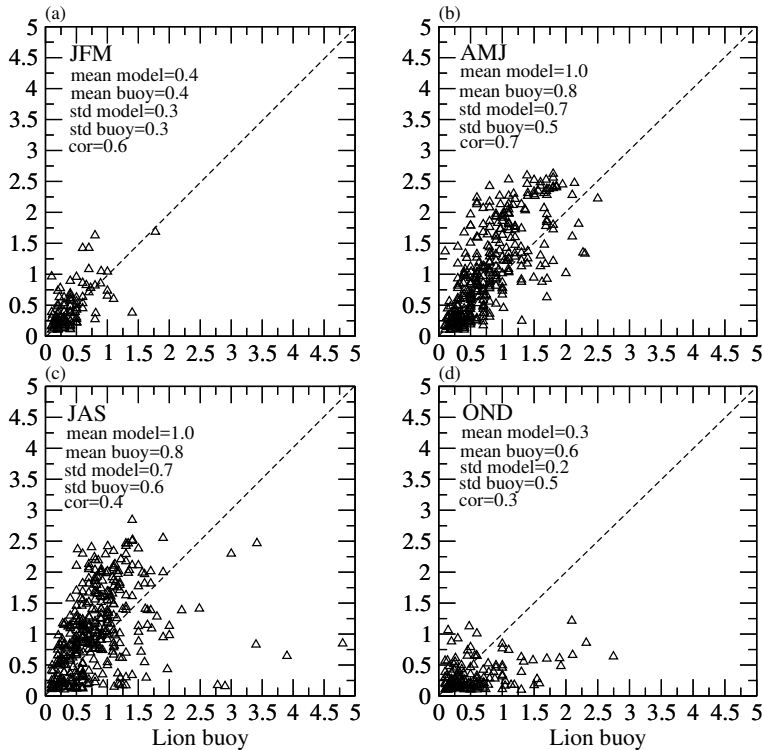
Figure 4. Amplitude in ^{\circ}\text{C} of the 2009-2013 SST diurnal cycle for the Lion Buoy (x-axis) and the model simulation (y-axis), according to the season a) JFM, b) AMJ, c) JAS and d) OND. Only values above 0.1^{\circ} are kept. Mean values and standard deviations are given for each season, as well as the daily temporal correlation.
