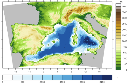
(c) AROME-NEMO WMED
