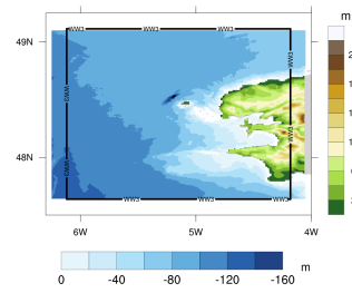
(f) MESONH-MARS3D-WW3
