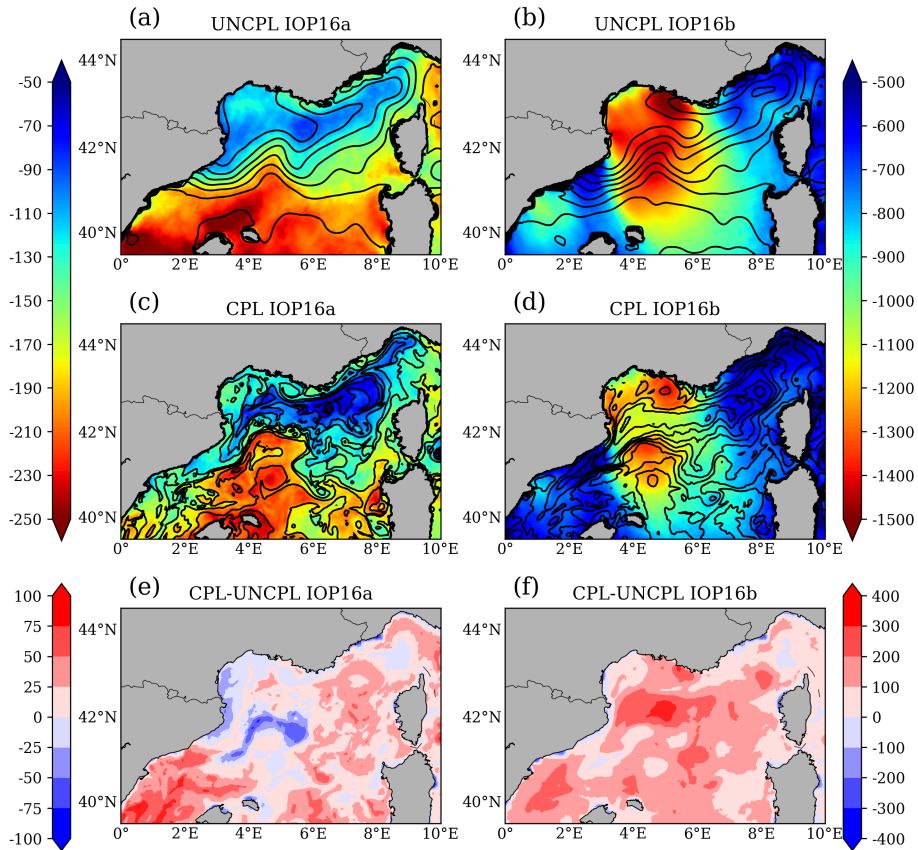
Figure 6. Spatial distribution of non-solar heat flux ( Q_{ns} , W m^{-2} ) and SST in black contours (contour interval of 0.5^{\circ}C ) averaged over IOP16a (left) and IOP16b (right) for UNCPL simulation (a, b), CPL simulation (c, d) and difference between CPL and UNCPL (e, f).
