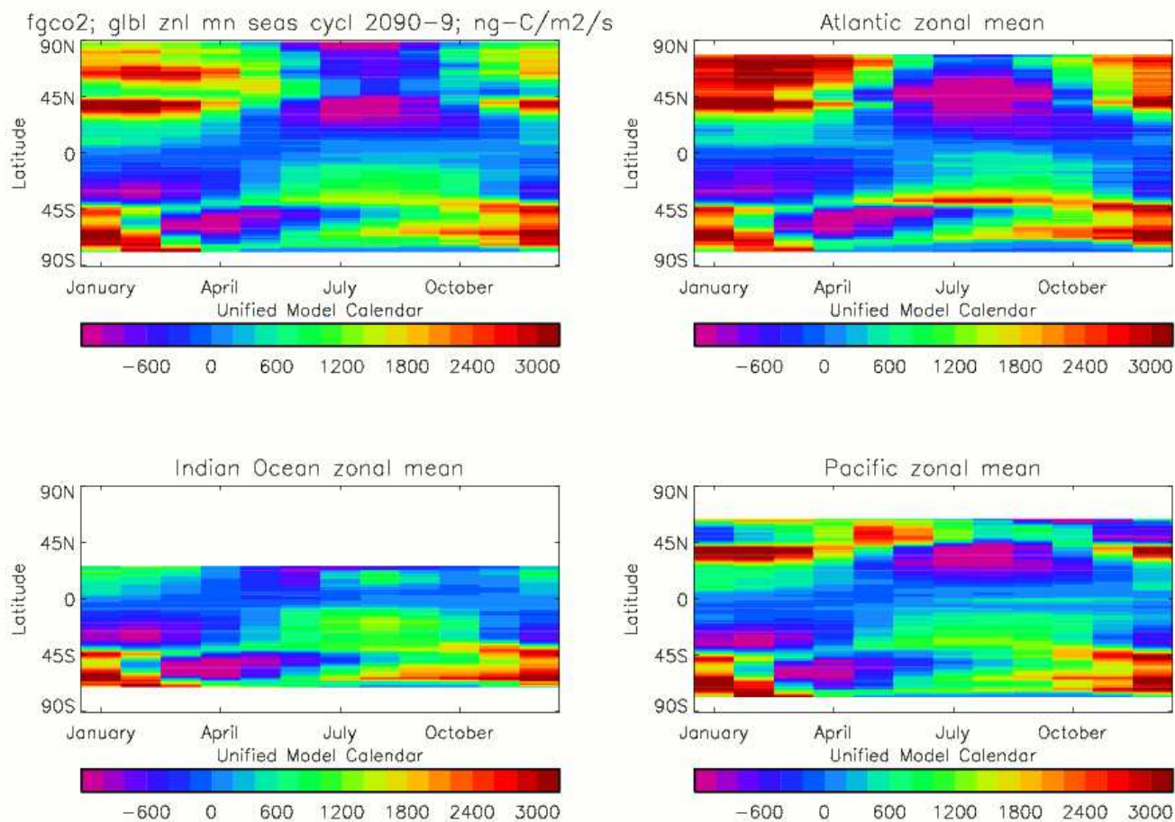
Figure 42. The seasonal cycle (monthly means) of the total air-to-sea \text{CO}_2 flux ( \text{ng C m}^{-2} \text{s}^{-1} ) averaged over the model years 2090-2099 inclusive. Zonal mean of: upper left panel, global ocean; upper right, Atlantic Ocean basin; lower left, Indian Ocean basin; lower right, Pacific Ocean basin
