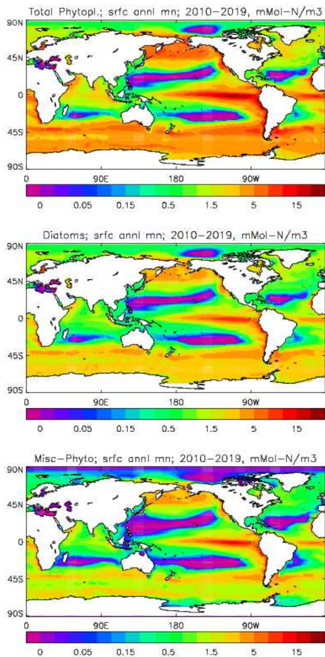
Figure 6. Phytoplankton surface biomass (in mMol N m -3 ), averaged over the model years 2010-2019 inclusive: top panel, total phytoplankton; middle panel, Diatoms; bottom panel, misc-Phytoplankton.
