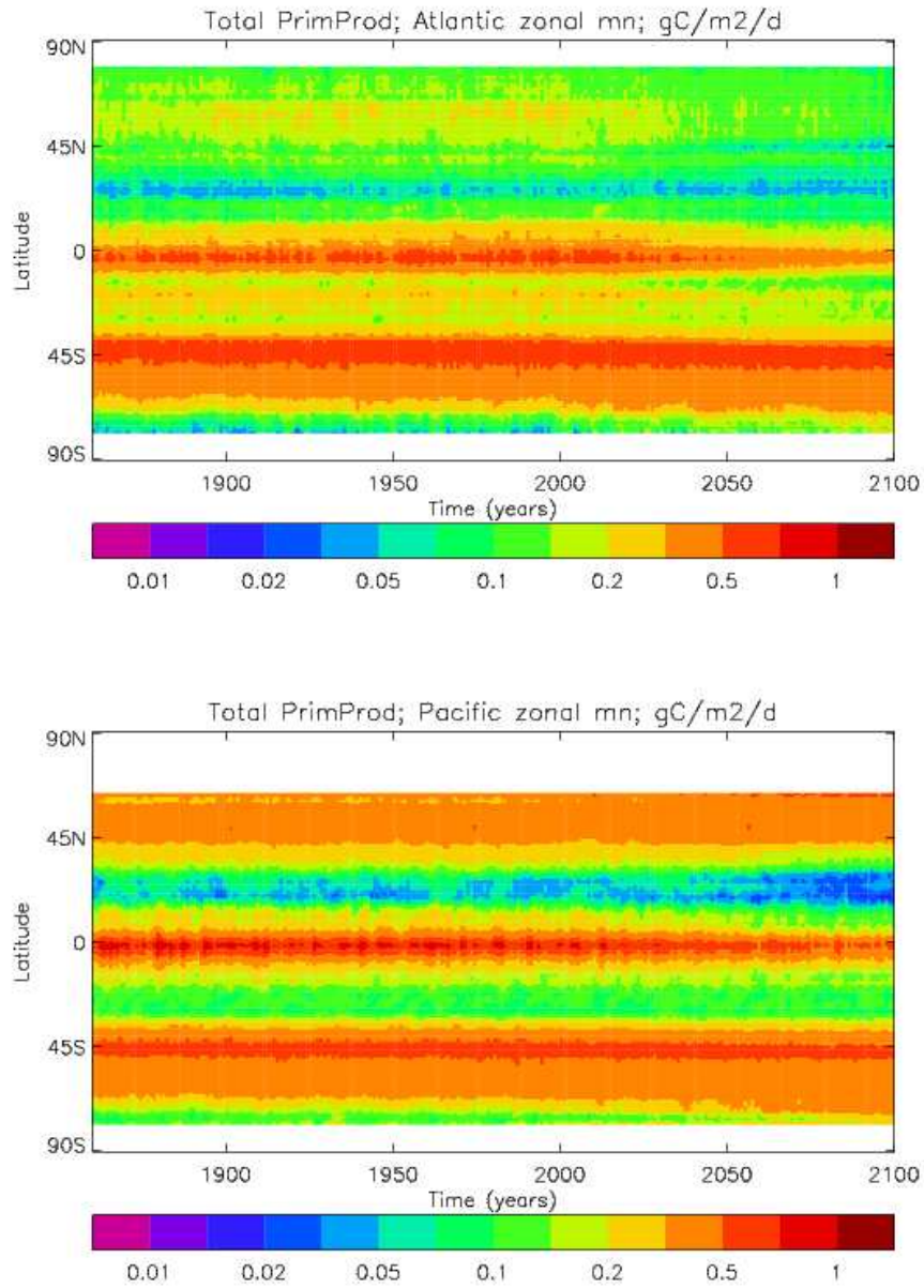
Figure 38. Change in annual mean depth-integrated total Primary Production ( \text{g C m}^{-2} \text{d}^{-1} ) during the model years 1860 to 2099 in the CMIP5 Historical and RCP8.5 simulations. Upper panel, Atlantic Ocean basin zonal mean; lower panel, Pacific Ocean basin zonal mean.
