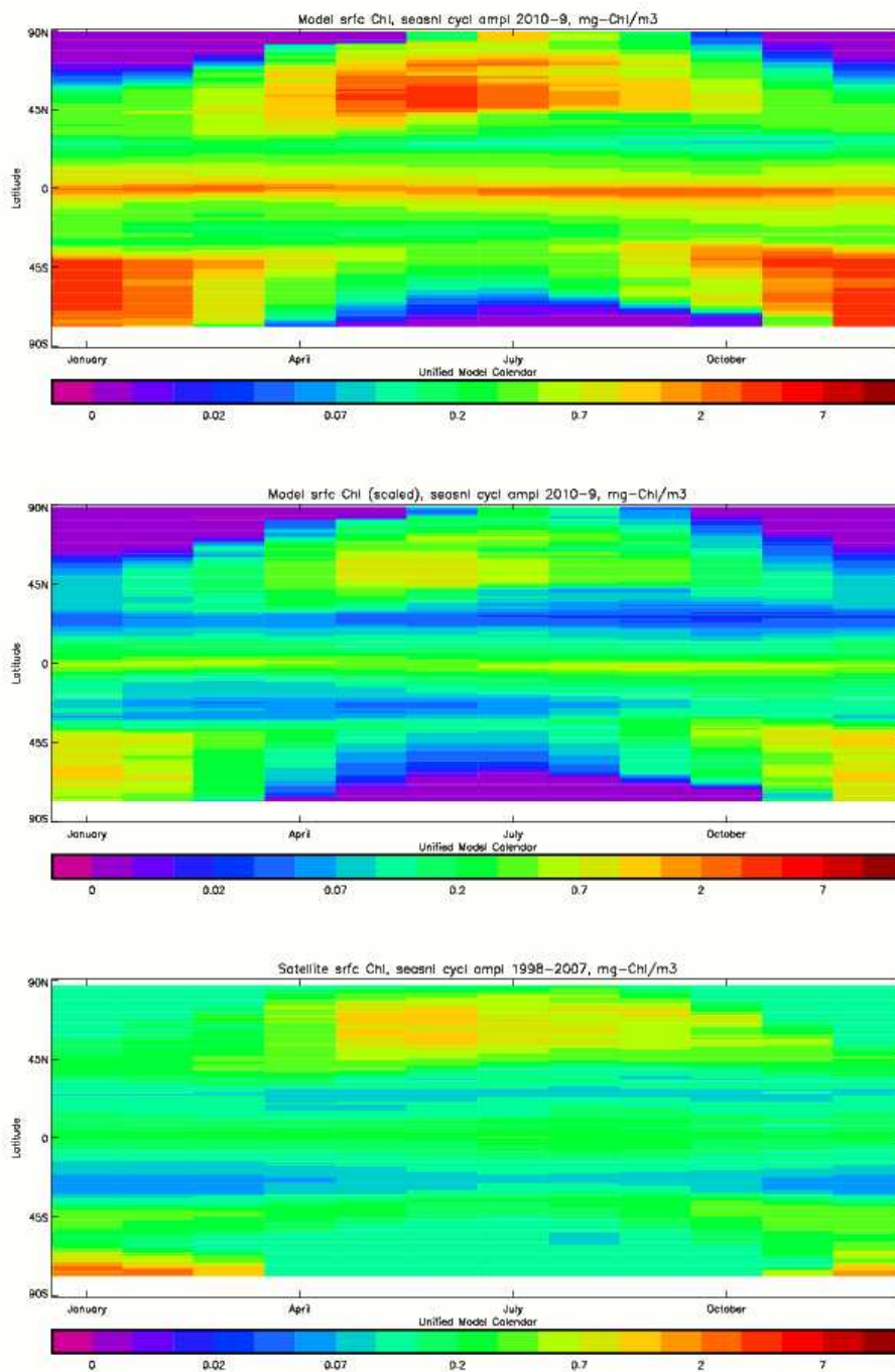
Figure 3. Seasonal cycle of global zonal mean surface chlorophyll, in \text{mg Chl m}^{-3} : top panel, average over the years 2010-9 inclusive from the model, Historical+RCP8.5 scenario; middle, the same but scaled by factor 0.213/0.812 (=0.262) so that the model mean matches the observations; bottom, satellite-derived data from GlobColor, averaged over 1998-2007 inclusive.
