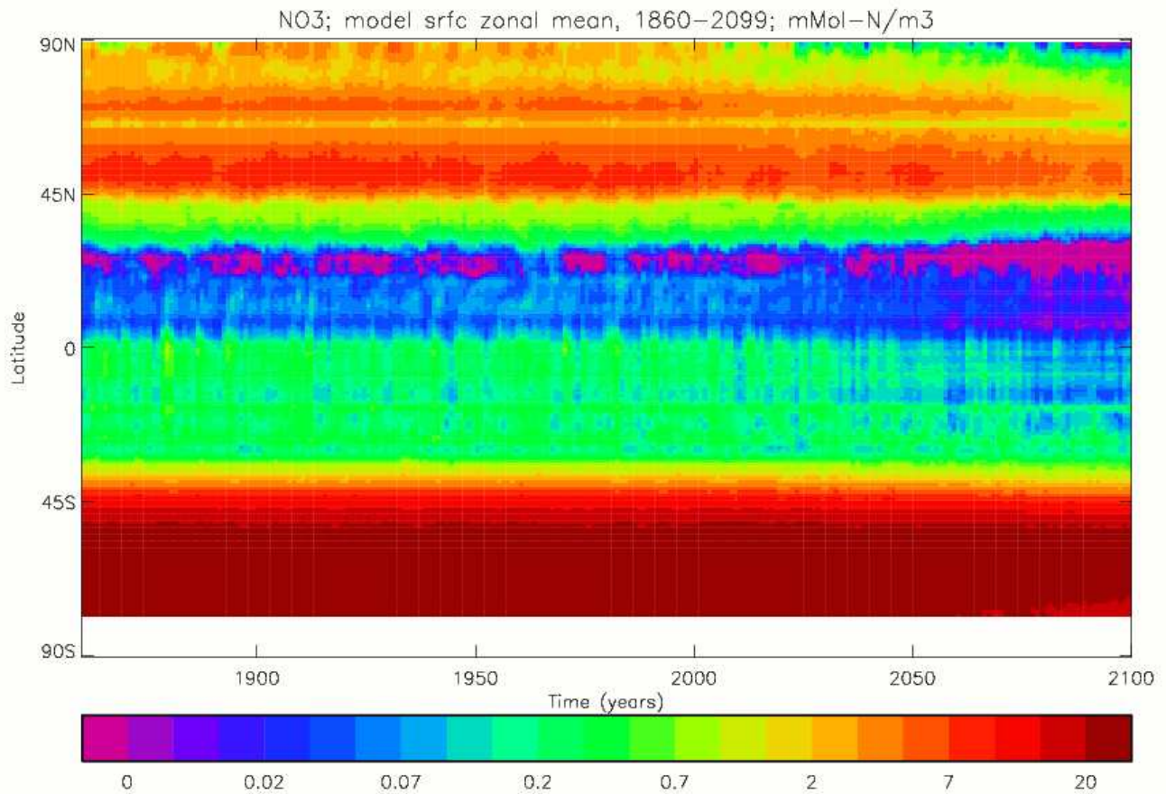
Figure 34. Surface dissolved nitrate concentration (mMol N m -3 ), global zonal and annual means for model years 1860 to 2099, from the CMIP5 Historical and RCP8.5 simulations, showing the response to changing climatic forcing
