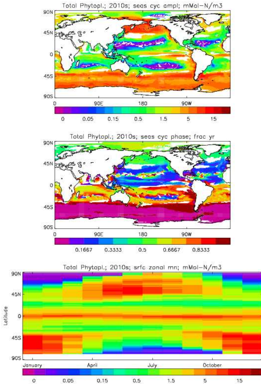
Figure 7. Total phytoplankton surface biomass mean seasonal cycle, averaged over model years 2010 to 2019 inclusive. Top panel, amplitude (in \text{mMol N m}^{-3} ) and middle panel, the phase (fraction of year when peak value occurs) of the seasonal cycle, determined by the best-fitting sine-curve (only points where the residual variance is less than half that of the original cycle are shown). Bottom panel, the global zonal mean for each month ( \text{mMol N m}^{-3} ).
