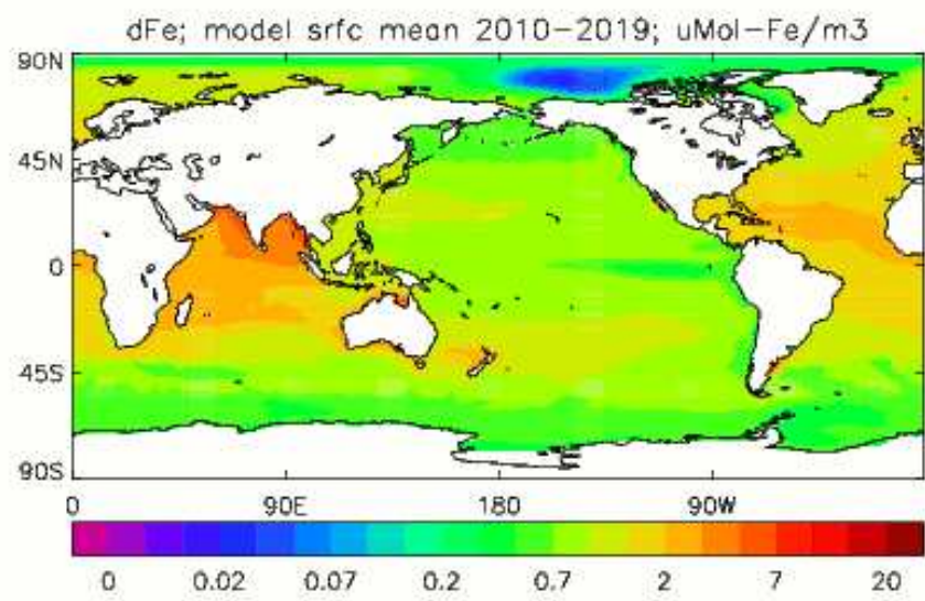
Figure 27. Surface dissolved iron, averaged over model years 2010-2019 inclusive (uMol Fe m -3 ).
