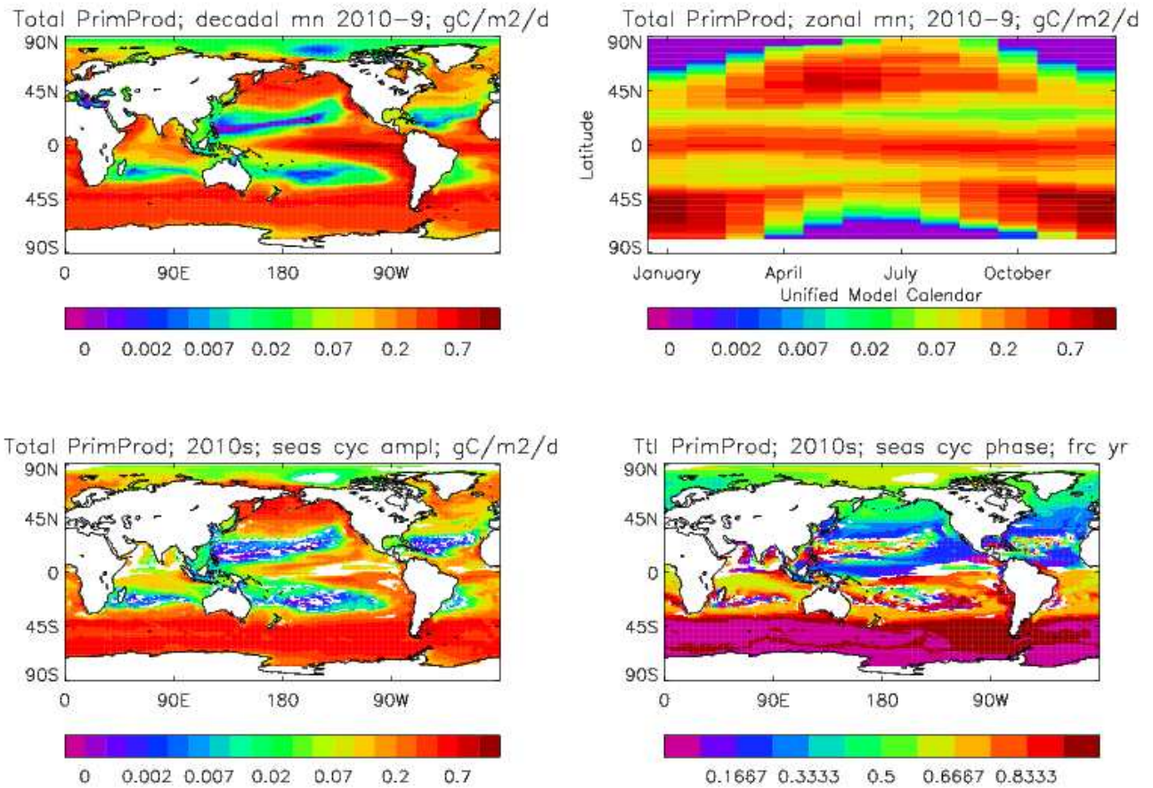
Figure 8. Total Primary Production, depth-integrated, averaged over the model years 2010-2019 inclusive: upper left panel, decadal mean (units: \text{g C m}^{-2} \text{d}^{-1} ); upper right panel, zonal mean for each month, same units; lower left, amplitude of model seasonal cycle (best fitting sine-curve), same units; lower right, phase of model seasonal cycle (units are fraction of year when peak value occurs). As described in the text, the seasonal cycle has been determined by the best-fitting sine-curve, and points are only shown where the variance of the residual cycle is less than half that of the original cycle.
