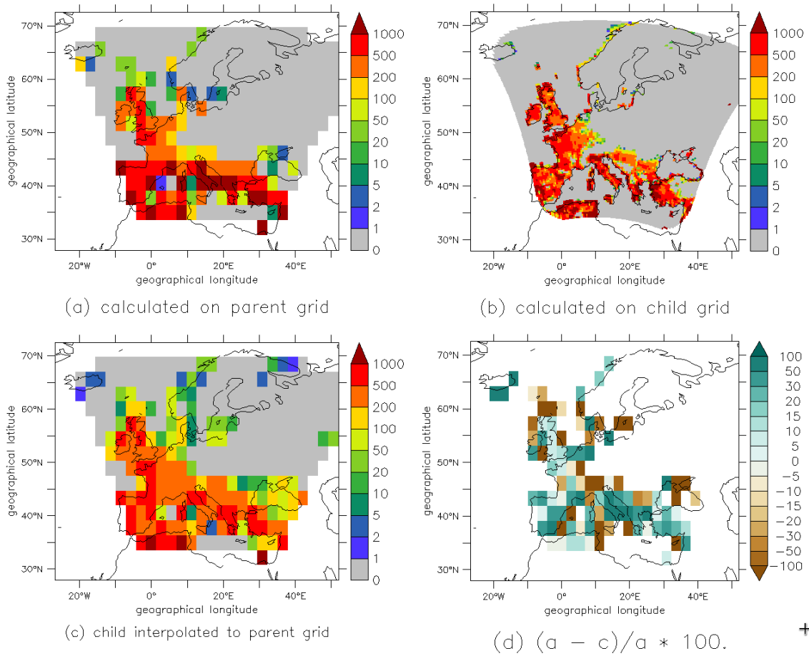
Figure 5. Biogenic NO emissions flux in pg\ m^{-2}\ s^{-1} for one distinct date in January 2003. The data has been masked to show only the coupled region.
