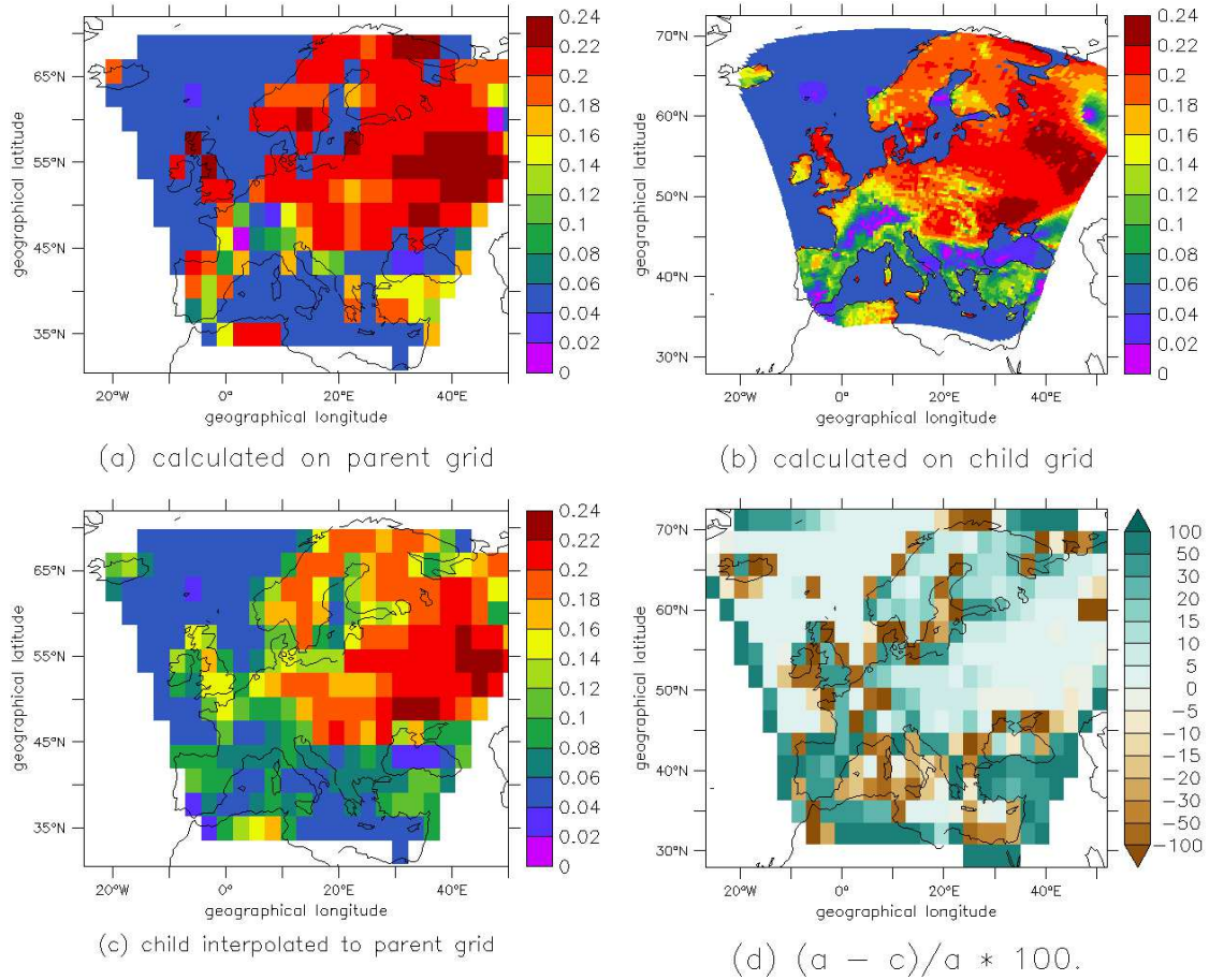
Figure 6. Ozone dry deposition velocities in \text{cm s}^{-1} for one distinct date in January 2003. The data has been masked to show only the coupled region.
