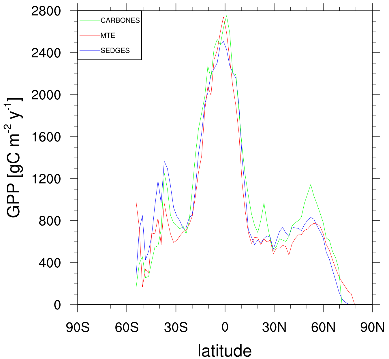
Figure A6. Zonal multi-year annual mean climatology of gross primary productivity (GPP) for SEDGES and the two reference datasets, MTE and CARBONES, for 1990-2009 over non-glaciated land.
