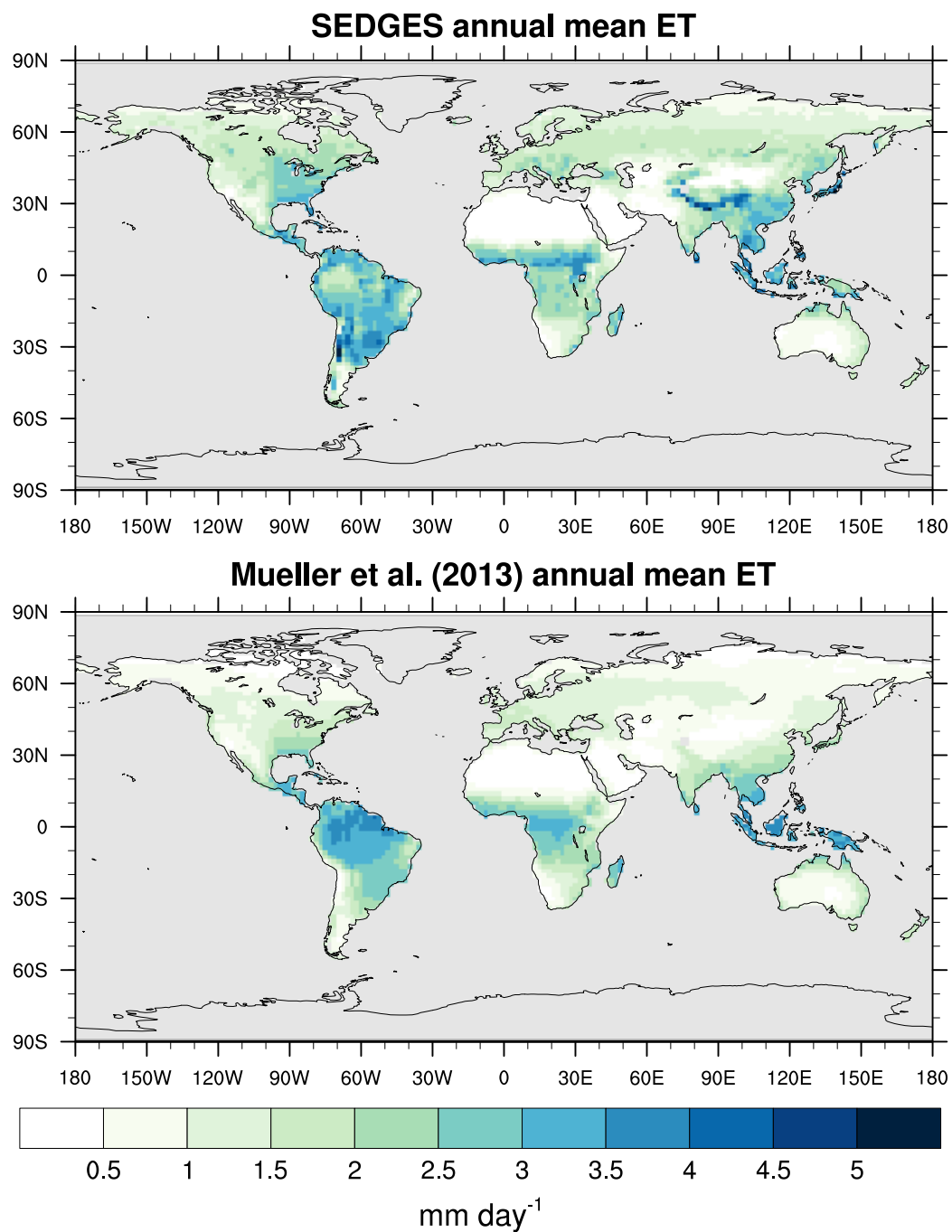
Figure A17. Multi-year annual means of white-sky-albedo evapotranspiration (ET) for 2001-2010 (NASA LP DAAC, b) SEDGES and the Mueller et al. (2013) reference dataset for the 1989-2005 period over non-glaciated land.
