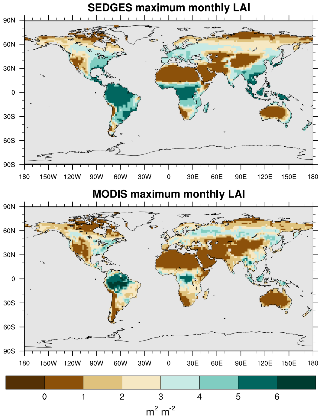
Figure A14. Maximum leaf area index (LAI) of the multi-year monthly mean climatology means for SEDGES and for the BNU MODIS-based reference dataset for the 2001-2010 period.
