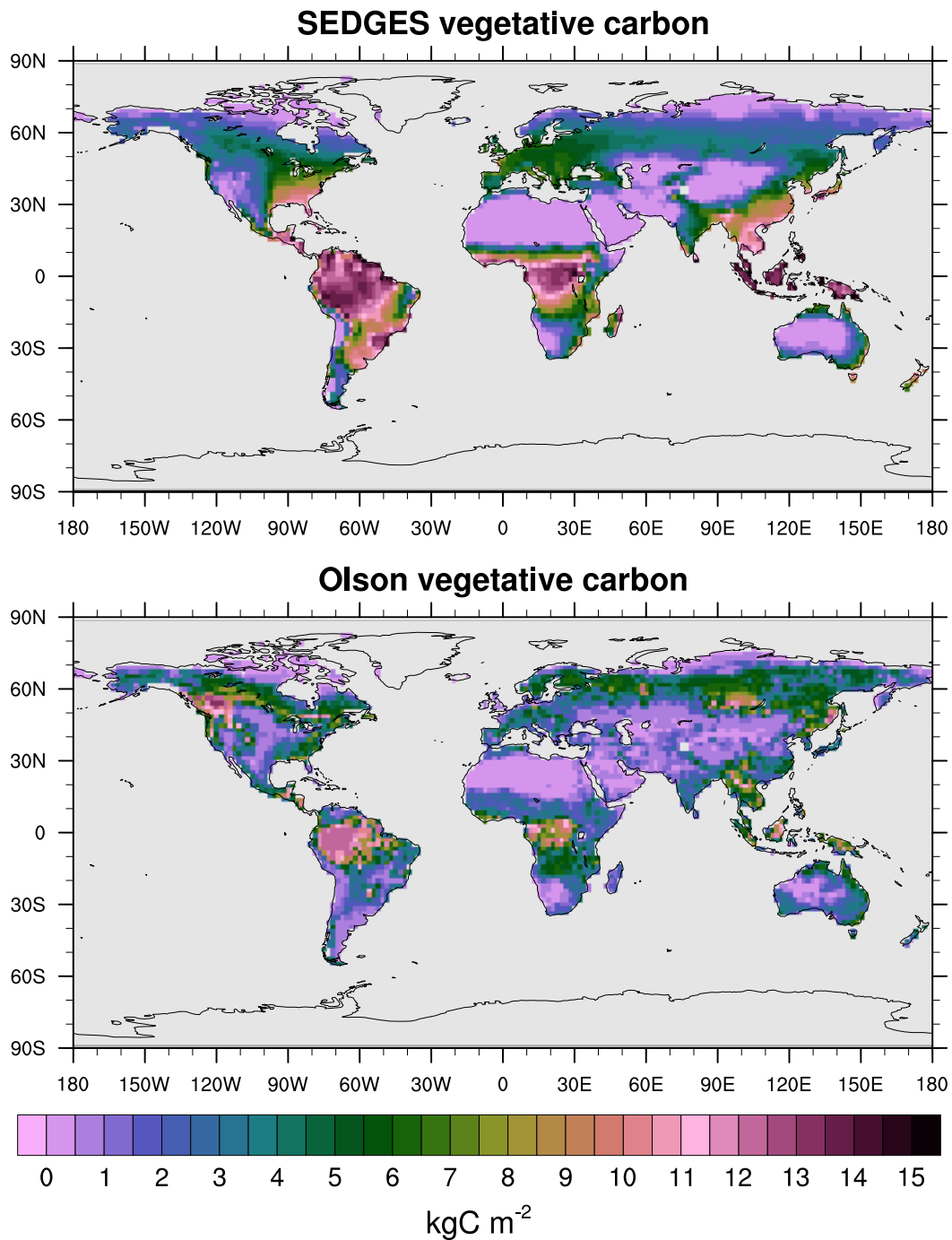
Figure A12. Vegetative carbon for SEDGES: mean over 1981-2010 in the transient CO 2 simulation; vegetative carbon from the Olson et al. (1985) reference dataset, which represents pre-Iron Age vegetation save for the most extreme anthropogenic land cover changes.
