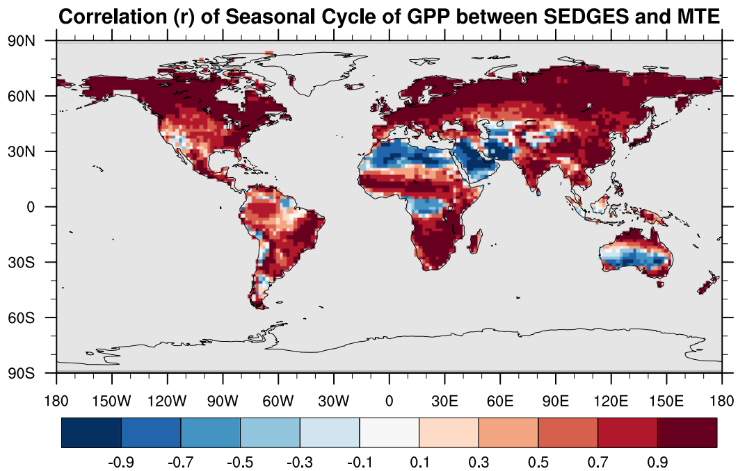
Figure A9. Pearson correlation coefficients of the seasonal cycle (i.e. of the climatological multi-year monthly means) between SEDGES and the MTE reference dataset for the 1986-2005 period.
