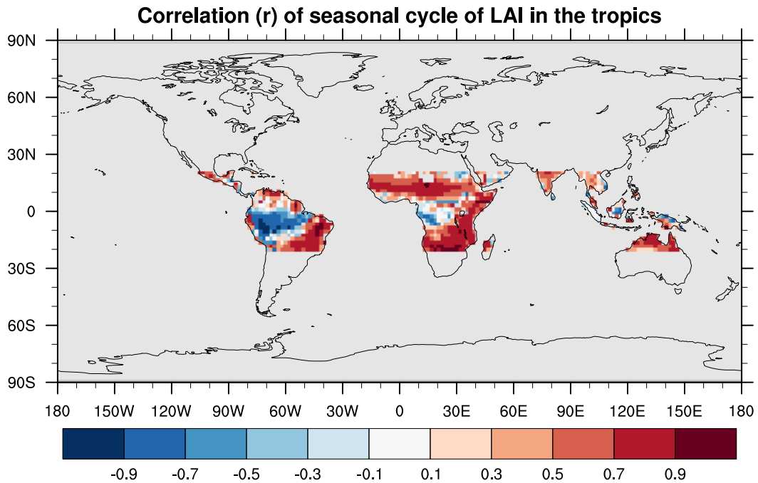
Figure A15. Temporal correlation at each grid point in the tropics ( -20^{\circ} to 20^{\circ} ) between the multi-year monthly mean climatologies means of LAI for 2001-2010 of SEDGES and of the BNU MODIS-based reference dataset. Some desert grid points do not have values because they have LAI's of 0 in one or both sets of data for all 12 months.
