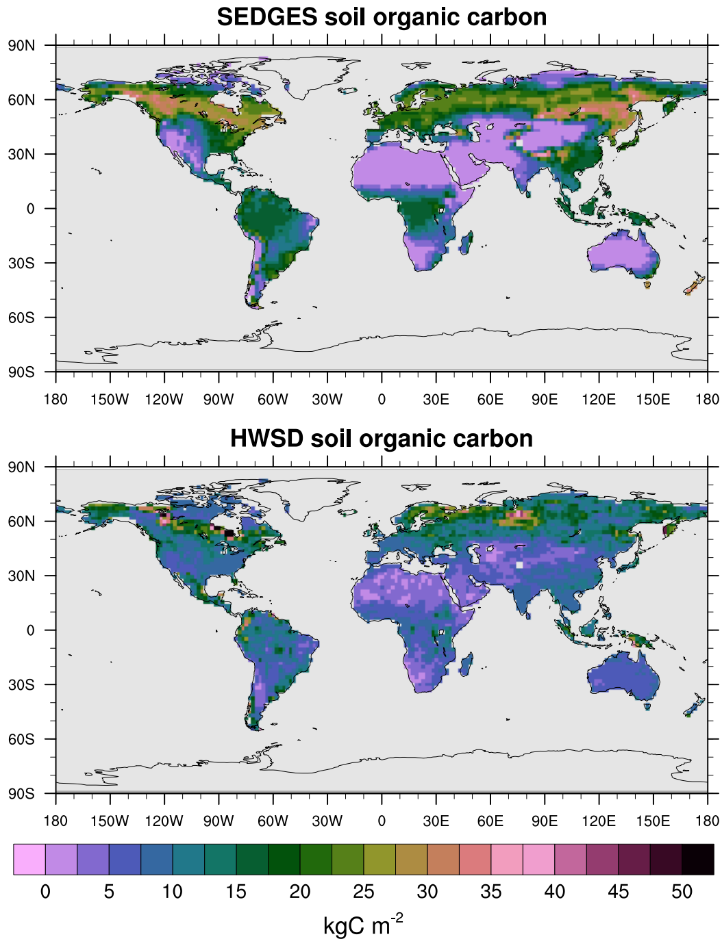
Figure A13. Soil organic carbon for SEDGES: mean over 1981-2010 of the transient CO 2 simulation; Soil-soil organic carbon from the Harmonized World Soil Database (HWSD) reference dataset (Wieder et al., 2011). The HWSD dataset has values for the top meter of the profile, only.
