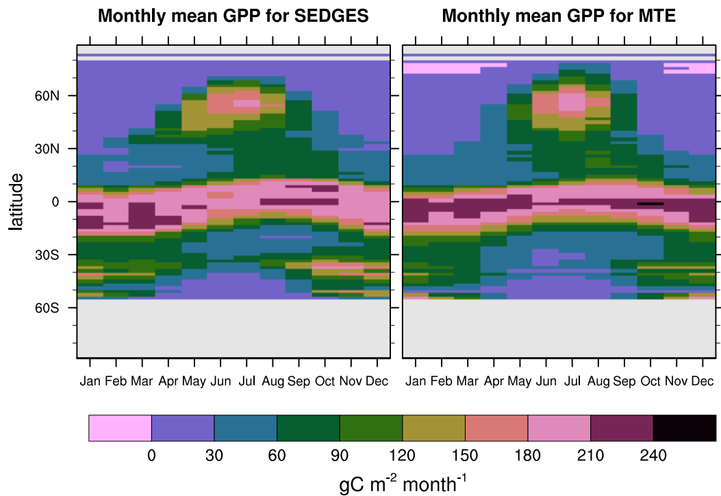
Figure A8. Zonal multi-year monthly mean-climatology-means of gross primary productivity (GPP) for SEDGES and the MTE reference dataset for 1982-2010 over non-glaciated land.
