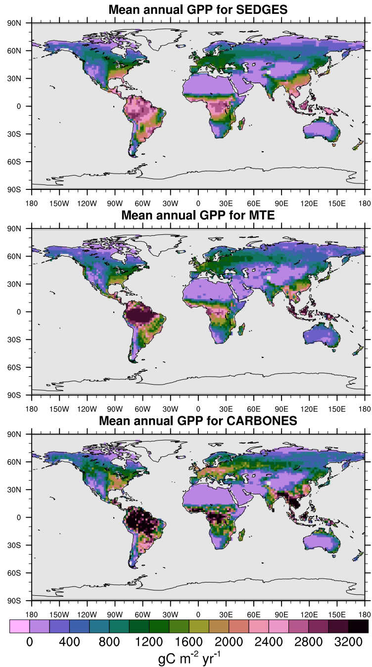
Figure A7. Annual Multi-year annual mean climatology of gross primary productivity (GPP) for SEDGES and the two reference datasets, MTE and CARBONES, for 1990-2009 over non-glaciated land.
