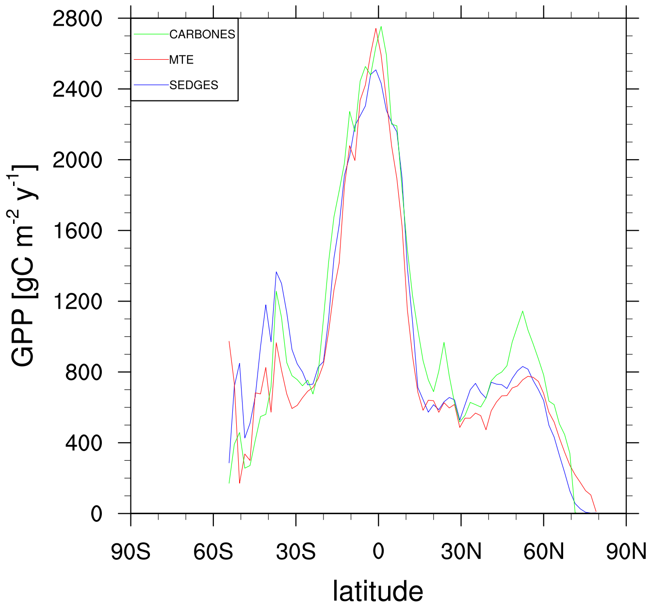
Figure A6. Zonal multi-year annual mean climatology of gross primary productivity (GPP) for SEDGES and the two reference datasets, MTE and CARBONES, for 1990-2009 over non-glaciated land.
