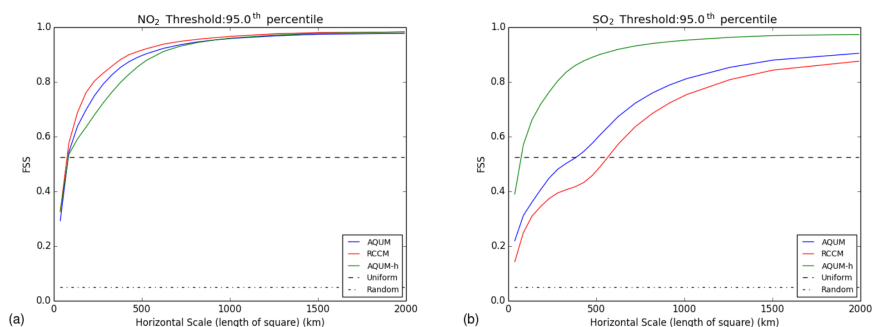
Figure 7. Fractional Skill Score for 95th Percentile for (a) \text{NO}_2 and (b) \text{SO}_2 . The RCCM is shown in red, AQUM in blue and AQUM-h in green. The ‘Random’ (dot-dashed) line represents the FSS for a random forecast with the same fraction of points over the domain exceeding the percentile threshold as the truth field. The ‘Uniform’ (dashed) line represents a forecast with the same fraction of points above the percentile threshold in the neighbourhood surrounding each grid point as the truth field for every grid point. Above this line the forecast is considered skilful.
