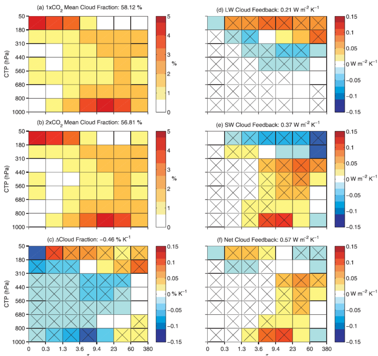
Figure 6. Global, annual, and ensemble mean cloud fraction for the (a) 1 \times \text{CO}_2 and (b) 2 \times \text{CO}_2 runs, along with (c) the average difference expressed per unit change in each model's global mean surface air temperature between the two states. Matrix resulting from multiplying the change in cloud fraction at each location and month with the collocated (d) LW, (e) SW, and (f) net cloud radiative kernels, then taking the global, annual, and ensemble mean. The sum of each matrix is shown in each title. Bins containing an "x" indicate those in which \geq 75\% of the models agree on the sign of the field plotted. Reprinted from Zelinka et al. (2012) ©American Meteorological Society. Used with permission.
