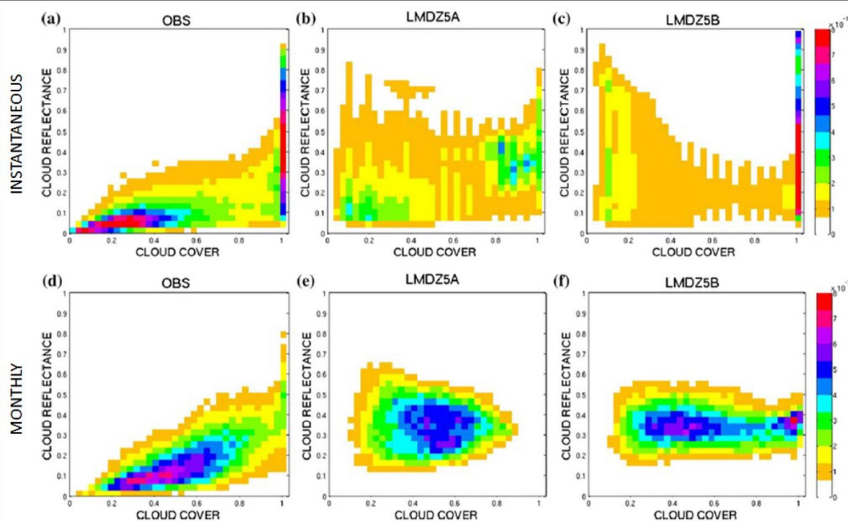
Figure 8. 2D histograms of cloud reflectance and cloud cover over the tropical oceans using instantaneous data ( upper panels ) and monthly data ( lower panels ) (a), (d) observed with PARASOL and CALIPSO-GOCCP, (b), (e) simulated with LMDZ5A and the simulator, and (c), (f) simulated with LMDZ5B and the simulator. The colour bar represents the number of points at each grid cell (cloud cover-cloud reflectance) divided by the total number of points. Reprinted with permission from Konsta et al. (2015).
