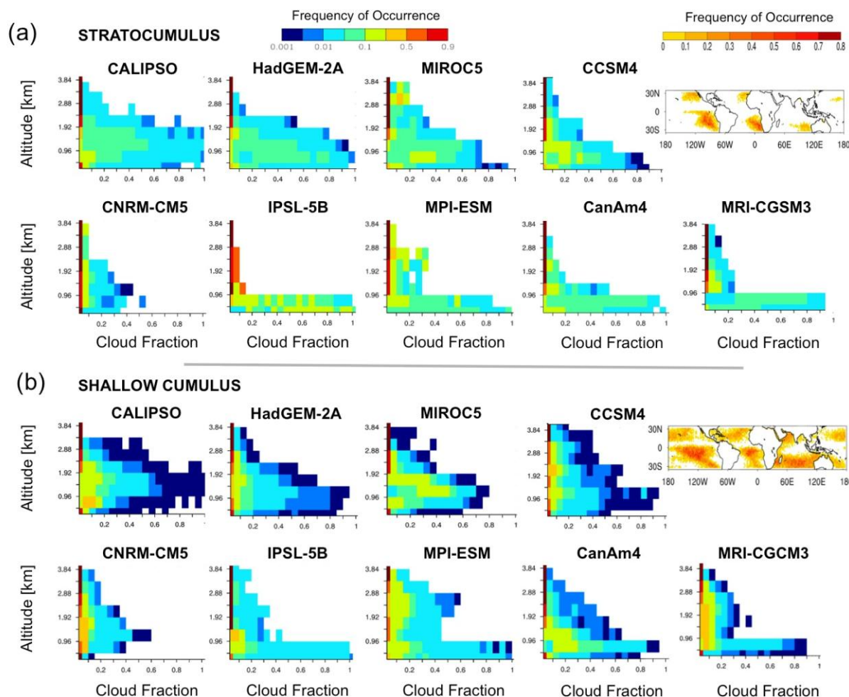
Figure 9. Comparison of the frequency of occurrence of clouds in the lowest 4 kms, of a given fraction at a given altitude under non-overlapped low-level cloud conditions for (a) stratocumulus regime and (b) shallow cumulus regime for CALIPSO-GOCCP and CMIP5 models. Maps show the frequency of occurrence of each regime derived from CALIPSO observations and ERA-Interim reanalysis. Reprinted from Nam et al. (2012).
