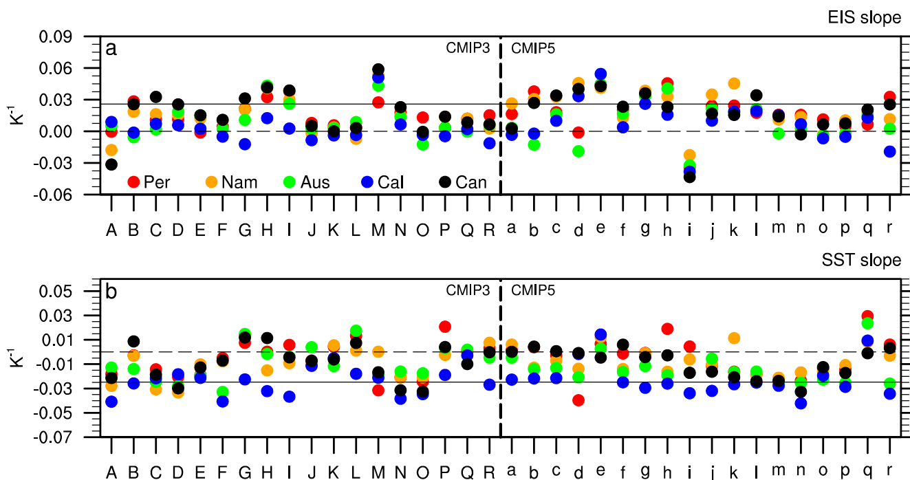
Figure 13. (a) The EIS slope ( \partial LCC / \partial EIS ), (b) the SST slope ( \partial LCC / \partial SST ) in the 5 oceanic regions from 36 models in the 20th-century and from the observations. Note that the observational slope values (solid lines) are the averages over the 5 regions. Reprinted with permission from Qu et al. (2014).
