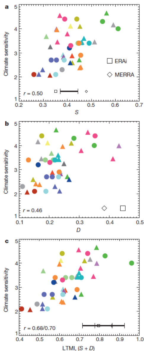
Figure 14. Scatterplot of S (a), D (b) and LTMI (the sum of S and D ) (c) on the abscissa and the equilibrium climate sensitivity (on the ordinate) from 43 CMIP3 (circles) and CMIP5 models (triangles). Symbol color identifies modeling center of origin. Linear correlation coefficients are given in the lower left corner of LTMI with the equilibrium climate sensitivity and the total system feedback, respectively. Two observational estimates for LTMI with error bars are shown on the abscissa with central values indicated by the unfilled square and diamond. Reprinted from Sherwood et al. (2014).
