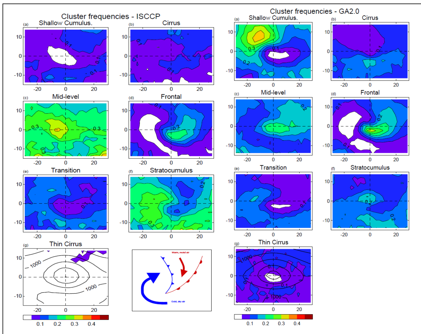
Figure 15. Relative Frequency of Occurrence of ISCCP derived cloud regimes composited on a cyclone-centred reference framework (left) obtained from ERA-40-daily-mean sea level pressure and (right) for a model (GA2.0) 's cloud regimes and mean sea level pressure. In (g), the thick contours show the mean sea level pressure with 8hPa intervals. (h) in the left panel is a schematic with the typical position of the fronts in the cyclone composite. Reprinted from Bodas-Salcedo et al. (2015) ©American Meteorological Society. Used with permission.
