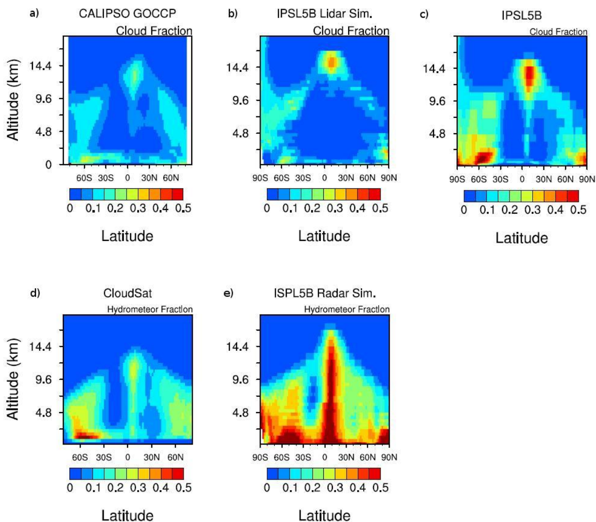
Figure 7. Zonal cloud and hydrometeor fraction for JJA 2007. Cloud Fraction (Top Row): (a) CALIPSO-GOCCP data, (b) IPSL5B with CALIPSO simulator, (c) IPSL5B cloud fraction. Hydrometeor Fraction (Bottom Row): (d) CloudSat data, (e) IPSL5B with CloudSat simulator. Produced for IPSL5B with the observational data used in Nam and Quaas (2012) ©American Meteorological Society. Used with permission.
