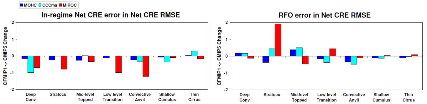
Figure 2. Changes between CFMIP-1 and CFMIP2 of RMSE components of a_i for net CRE within daily ISCCP simulator cloud regimes in the tropics. (a) In-regime net CRE components ( f_i^o C_i^o ), (b) frequency of occurrence components ( f_i^o C_i^o ). Cloud regimes are in the order of larger albedo. A graph drawn using the values in Table 2 in Tsushima et al. (2013).
