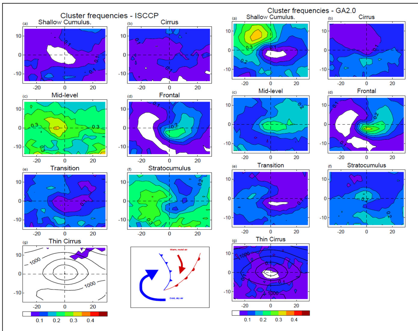
Figure 14. Relative Frequency of Occurrence of ISCCP derived cloud regimes composited on a cyclone-centred reference framework (left) obtained from ERA-40-daily-mean sea level pressure and (right) for a model (GA2.0) 's cloud regimes and mean sea level pressure. In (g), the thick contours show the mean sea level pressure with 8hPa intervals. (h) in the left panel is a schematic with the typical position of the fronts in the cyclone composite. Reprinted from Bodas-Salcedo et al. (2015) ©American Meteorological Society. Used with permission.
