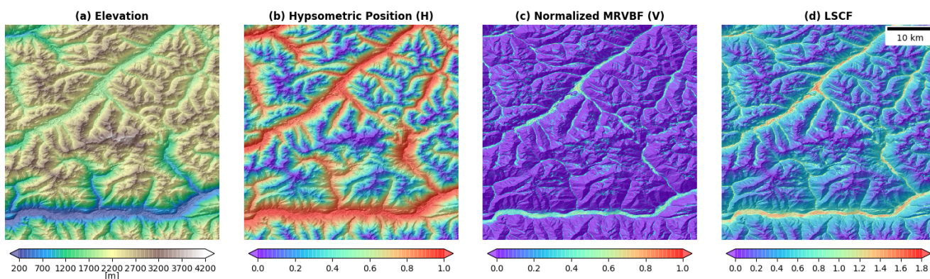
Figure 8. Spatial variation of elevation (a), hypsometric position (b), normalized MRVBF (c) and LSCF (d) in selected slope terrain (9.2999° N, 10.3998° W, 46.9999° N, 45.9999° S).
