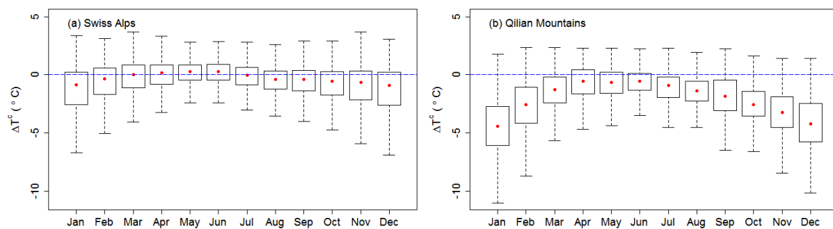
Figure 4. Seasonal changes shown as monthly distributions of average daily \Delta T^c derived from ERA-Interim for the locations of all stations.
