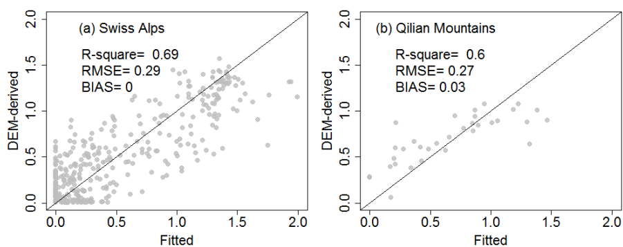
Figure 7. Ten-fold cross-validation of DEM-derived LSCF against fitted values in the Swiss Alps (a) and the Qilian Mountains (b).
