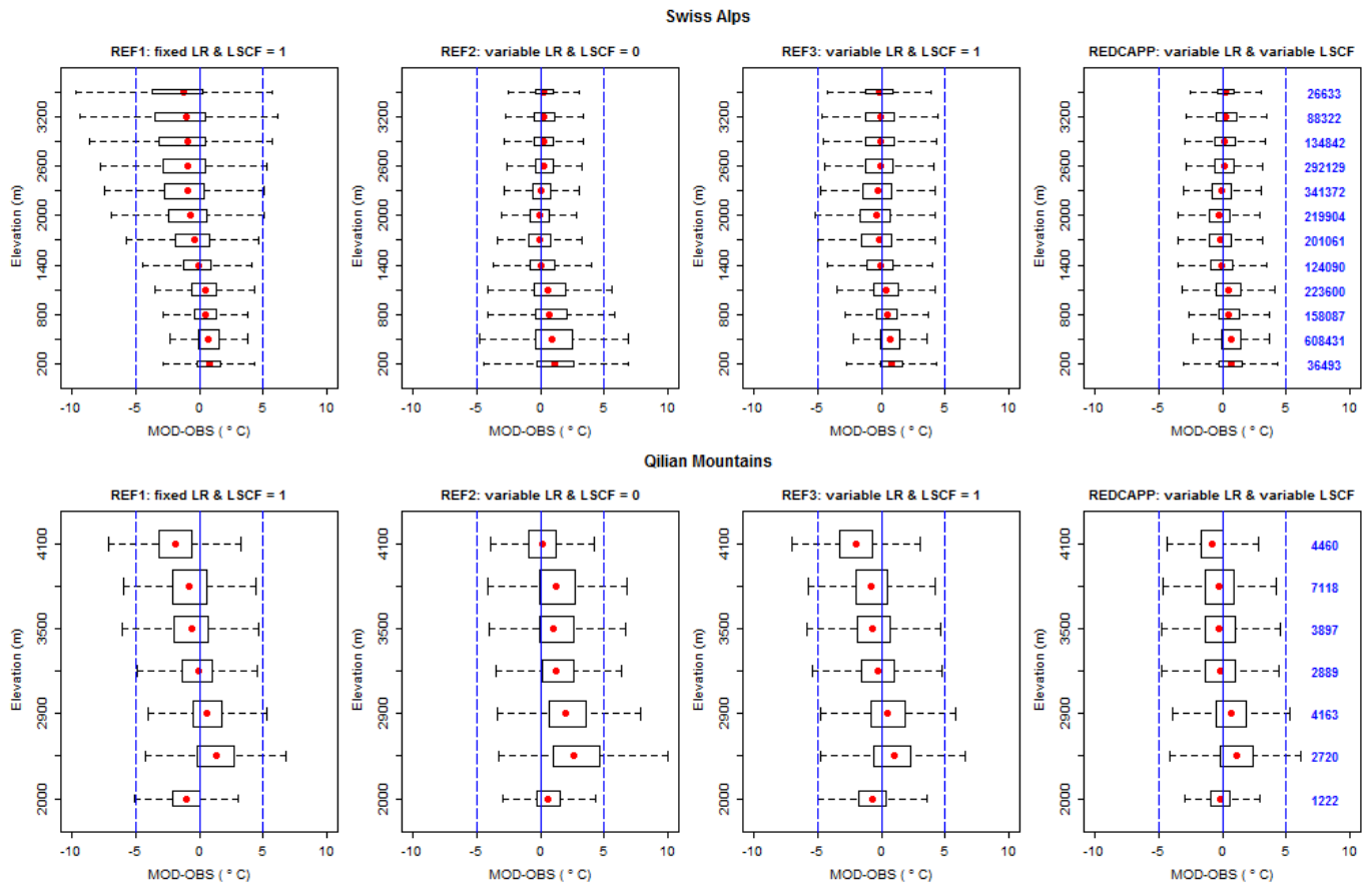
Figure 11. Deviances of downscaled results by elevations. The stations are grouped by elevation with an interval of 300 m. Each box may contain multiple stations and the numbers of observation times (days) are given in blue on the right.
