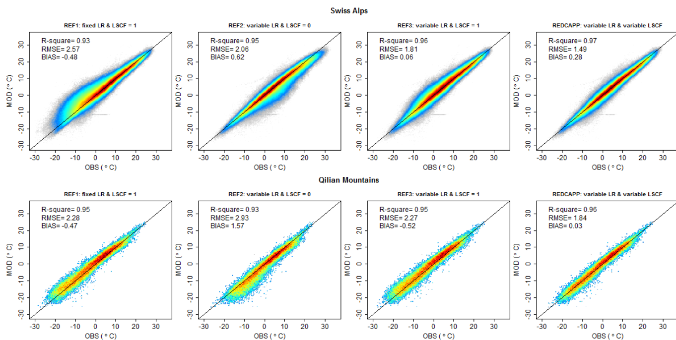
Figure 9. T_{obs} (OBS) against results of REF1, REF2, REF3 and REDCAPP (MOD). LR in subtitle means lapse rate.
