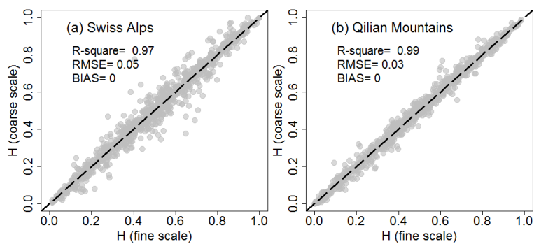
Figure A1. Comparison of hypsometric position derived from coarse-scale (15 arc-second) and fine-scale (3 arc-second) DEMs based on a random sample of 1000 points.
