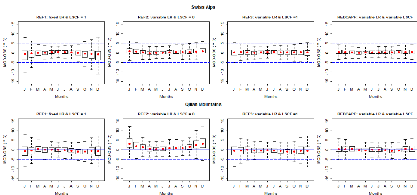
Figure 10. Seasonal deviance of downscaled daily results (MOD-OBS) for different methods.
