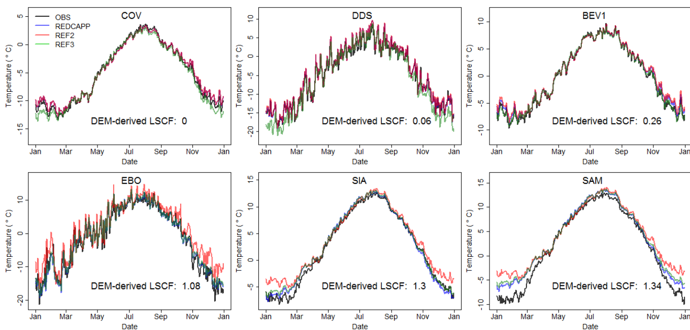
Figure 12. Comparison of REF2, REF3 and REDCAPP with time series at selected stations. The daily temperatures present are averaged based on all available years; the shorter time series for EBO explains the larger variation in the plot.
