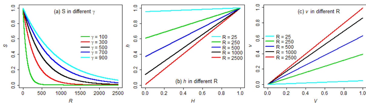
Figure 3. (a) Scale factor ( S ) decreases with increasing elevation range ( R ) by using different \gamma values. Fraction influence of surface effect on T ( h ) increases with hypsometric position ( H ) and strength of CAP ( v ) increases with normalized MRVBF ( V ). \gamma is 500 in figure (b) and (c). The lowest point in the landscape always receive a weight of 1 in h and a weight of 0 in v .
