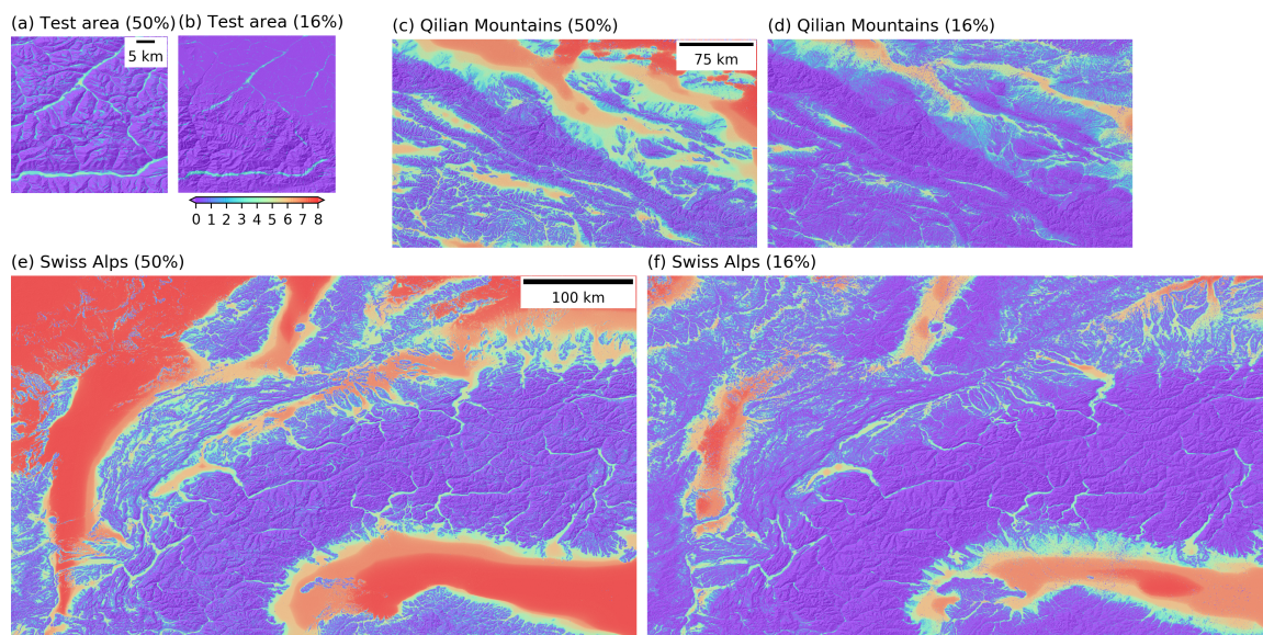
Figure A2. Original MRVBF in the test area, Swiss Alps and the Qilian Mountains by using slope threshold of 50% and 16%.
