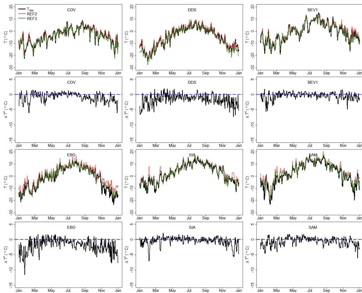
Figure 5. Detailed timeseries of \Delta T^c , T_{obs} , REF2 and REF3 at the selected stations from different geomorphometric positions.
