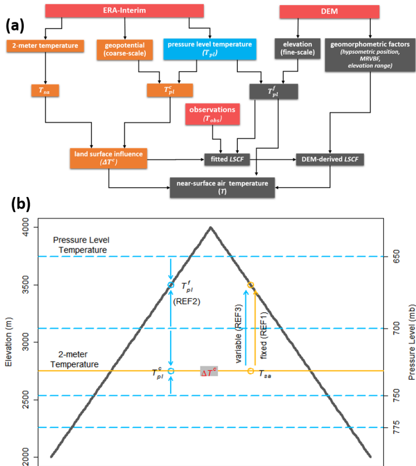
Figure 2. Model flow chart (a) and schematic illustration of interpolations and reference methods (b). Red squares denote input datasets. Variables at the elevation of coarse-scale topography are marked in yellow while the elevation of fine-scale topography is shown in grey. T_{pl} in blue could be at both coarse and fine scale of elevation. Blue arrows and points are variable lapse rates and temperatures derived from T_{pl} , while yellow point is temperature derived from T_{sa} and yellow arrow is the fixed lapse rate of -6.5 \text{ }^\circ\text{C km}^{-1} . Detailed symbol and variable names can be found in Appendix A. Schematic illustration is revised from Fiddes and Gruber (2014).
