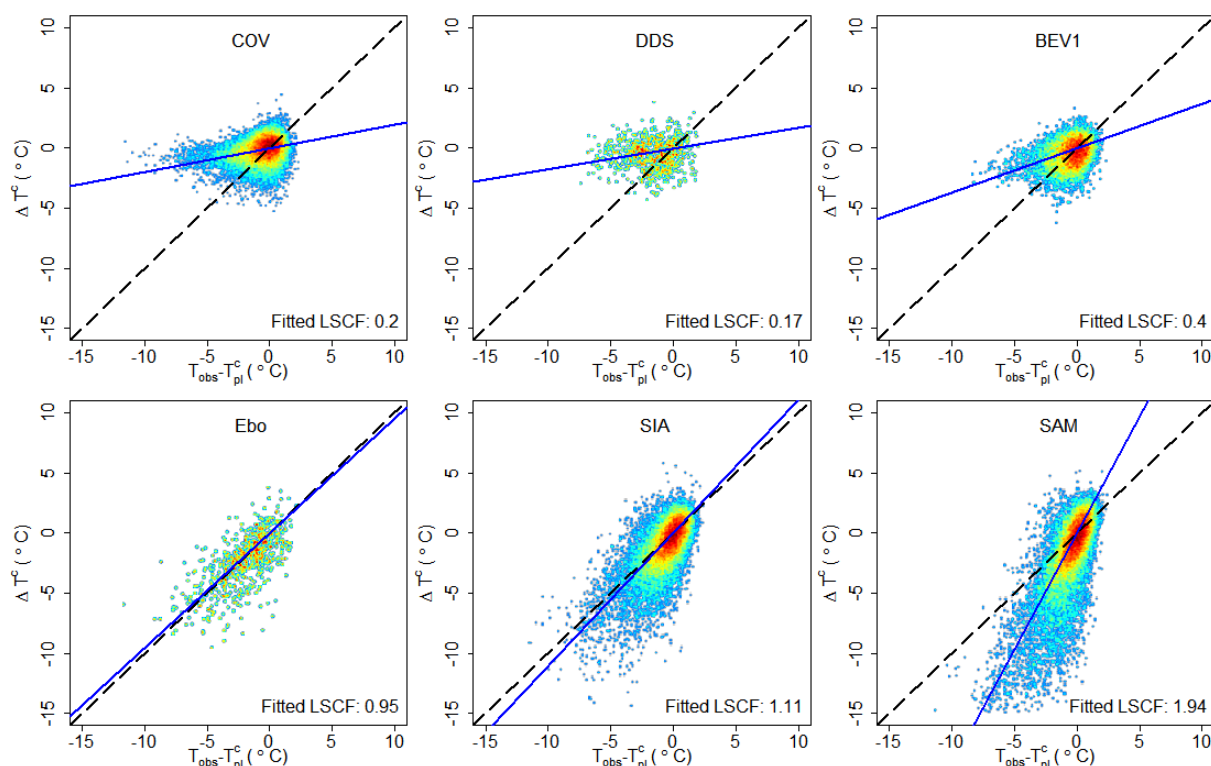
Figure 6. Difference of observed temperature and a prediction involving pressure levels ( T_{obs}-T_{pl}^c ) against \Delta T^c . The representation is a smoothed color density of a scatter plot to make a quality of points visual. The lines are results of LSCF * \Delta T^c by using LSCF = 1 (black dash) and best-fitted LSCF (blue solid) at the selected stations.
