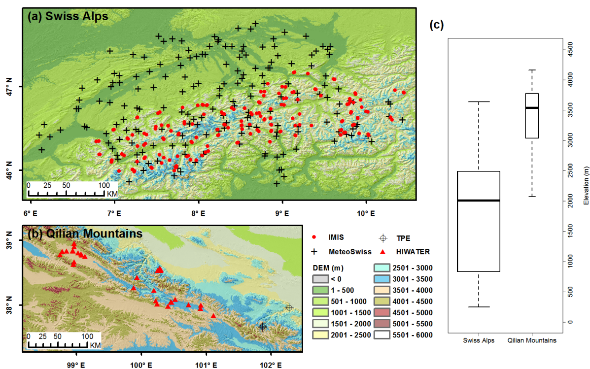
Figure 1. Experimental region of and observation stations in the Swiss Alps (a) and the Qilian Mountains (b). Elevation distribution of observation station (c). N is the number of observation stations.
