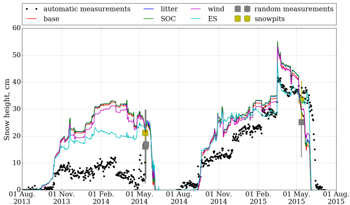
Figure 2. Snow height evolution over the 2 years of observations. Results of several hundred measurements using an avalanche probe (random measurements) and of a few snow pit data close to our site, performed in May 2014 and 2015, are also shown.
