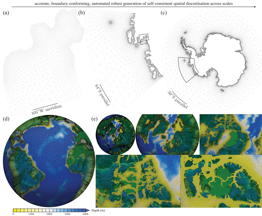
Fig. 9: A selection of further example geophysical domain discretisations straight-forwardly described in BRML and automatically constructed using Shingle. (a) T_h of the Pine Island Glacier ice shelf ocean cavity from ice-bedrock grounding line extended out to the 105°W meridian. (b) The Amundsen Sea region in West Antarctica extended out to the 64°S parallel. (c) The Southern Ocean Antarctic continent landmasses, from ice grounding line to 50°S parallel, built from a high fidelity boundary representation containing 348 automatically identified islands. (d) The full T of the global oceans, with a radial scaling of 300 to exaggerate the vertical extent of the discretised shell and land regions shaded green. (e) Zoomed in regions focusing on the complex Canadian Arctic Archipelago west of Greenland around Ellesmere and Baffin island. (a)–(c) are generated from the GEBCO (2014) DEM and presented under a orthographic projection centred on 90°S, and (d)–(e) from RTopo (Timmermann et al., 2010) and viewed in a Cartesian frame. These contain a multi-scale of spatial resolutions, with element edge-lengths parallel to the geoid in these examples, specified through \mathcal{M}_h , ranging from 2km to 500km. Vertical layers in (d), specified through \mathcal{M}_v , vary from 2m to 500m, under differing regimes in a generalised hybrid coordinate system described further in Candy (2016), and leads to a mesh containing 8,778,728 elements and 35,114,912 spatial degrees of freedom under its discontinuous Galerkin finite element discretisation. Along with other examples presented in figure 1(c)–(g), these are part of the test suite accompanying the library.
