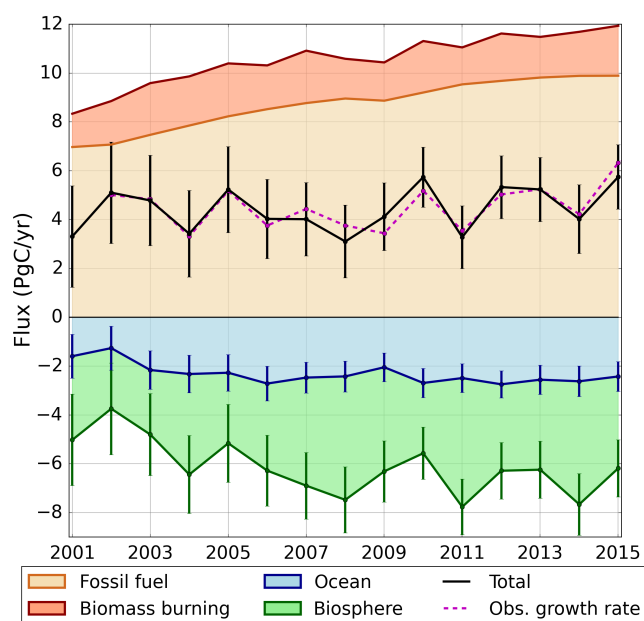
Figure 3. Global annual carbon balance estimated with CTE2016 for the period 2001-2015. Global ocean (blue) and biosphere (green) sinks are indicated as negative values and represent uptake from the atmosphere. The error bars represent the annual 1\sigma uncertainty, based on the average weekly covariances (more information on the error estimates in CarbonTracker is given in Sect. 3.4). Fossil fuel (orange) and biomass burning (red) emissions are not optimized. The total flux (black line) is the sum of the four components. The observed global annual atmospheric \text{CO}_2 growth rate from the NOAA network (dashed magenta line) was converted from ppm/year using a conversion factor of 2.12 PgC per ppm (Prather et al., 2012).
