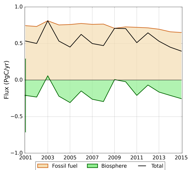
Figure 7. Annual carbon balance for European forests estimated with CTE2016 for the period 2001-2015. The biosphere (green) sink is shown together with the fossil fuel (orange) emission from the same region. The error bar represents the annual 1\sigma uncertainty, based on the average weekly covariances, and is shown only for 2001 for clarity (more information on the error estimates in CarbonTracker is given in Sect. 3.4). The total flux (black line) is the sum of the components.
